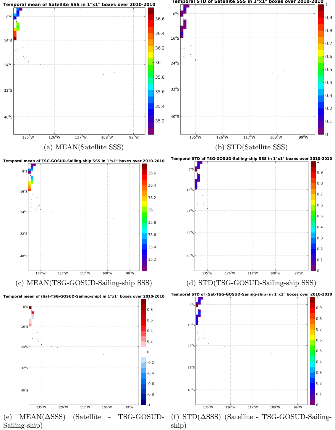
Figure 6: Temporal mean (left) and STD (right) of SSS from SMOS-L3-ICDC-V3-MONTHLY-0.5DEG (top), TSG-GOSUD-Sailing-ship (middle), and of \Delta SSS (Satellite - TSG-GOSUD-Sailing-ship). Only match-up pairs are used to generate these maps.
