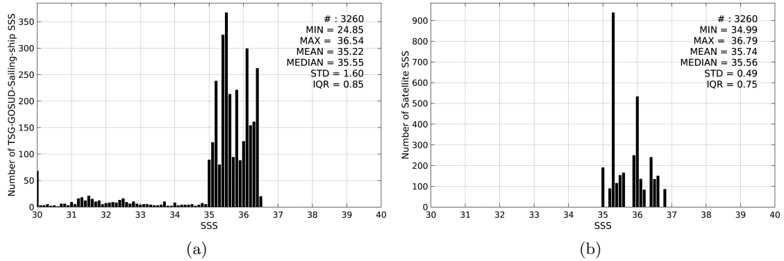
Figure 2: Histograms of SSS from TSG-GOSUD-Sailing-ship (a) and SMOS-L3-ICDC-V3-MONTHLY-0.5DEG (b) considering all match-up pairs per bins of 0.1 over the OTT zone Pi-MEP region and for the full satellite product period.
