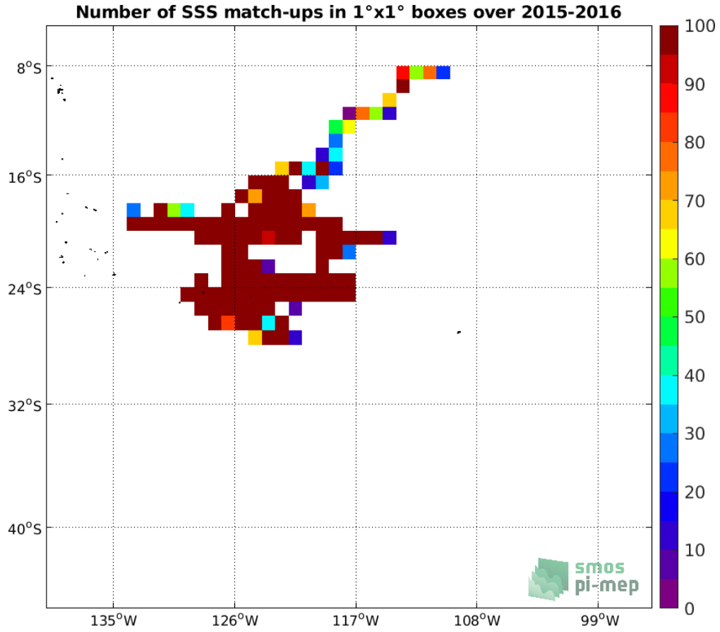
Figure 3: Number of SSS match-ups between Surface drifters SSS and the SMOS SSS L3 v3 Monthly (ICDC) SSS product for the OTT zone Pi-MEP region over 1^\circ \times 1^\circ boxes and for the full satellite product period.
