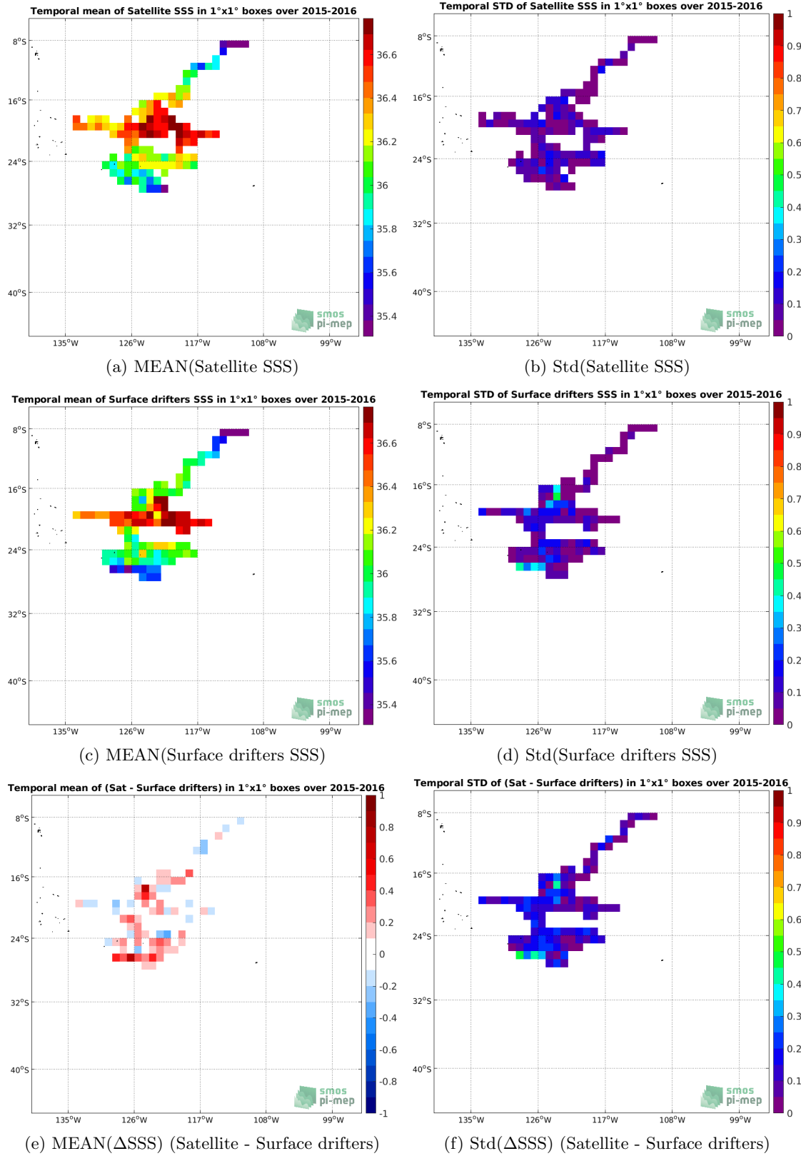
Figure 5: Temporal mean (left) and Std (right) of SSS from SMOS SSS L3 v3 Monthly (ICDC) (top), Surface drifters (middle), and of \Delta SSS (Satellite - Surface drifters). Only match-up pairs are used to generate these maps.
