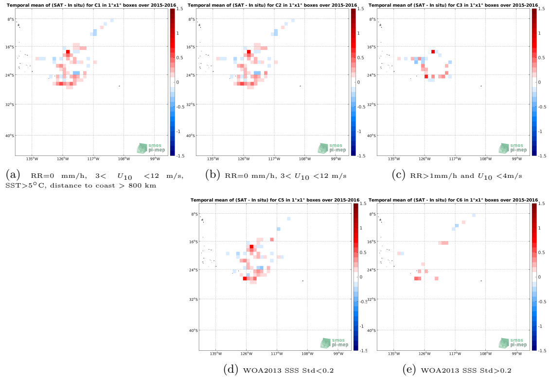
Figure 11: Temporal mean gridded over spatial boxes of size 1^\circ \times 1^\circ of \Delta SSS (SMOS SSS L3 v3 Monthly (ICDC) - Surface drifters) for 5 different subdatasets corresponding to: RR=0 mm/h, 3 < U_{10} < 12 m/s, SST > 5^\circ C , distance to coast > 800 km (a), RR=0 mm/h, 3 < U_{10} < 12 m/s (b), RR > 1 mm/h and U_{10} < 4 m/s (c), WOA2013 SSS Std < 0.2 (d), WOA2013 SSS Std > 0.2 (e).
