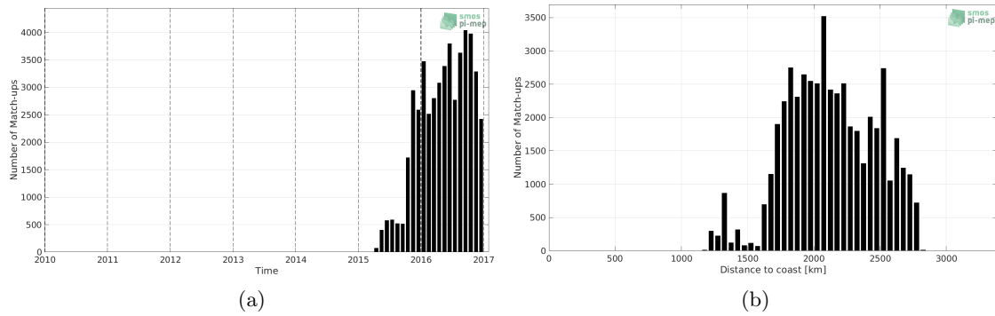
Figure 1: Number of match-ups between Surface drifters and SMOS SSS L3 v3 Monthly (ICDC) SSS as a function of time (a) and as function of the distance to coast (b) over the OTT zone Pi-MEP region and for the full satellite product period.
