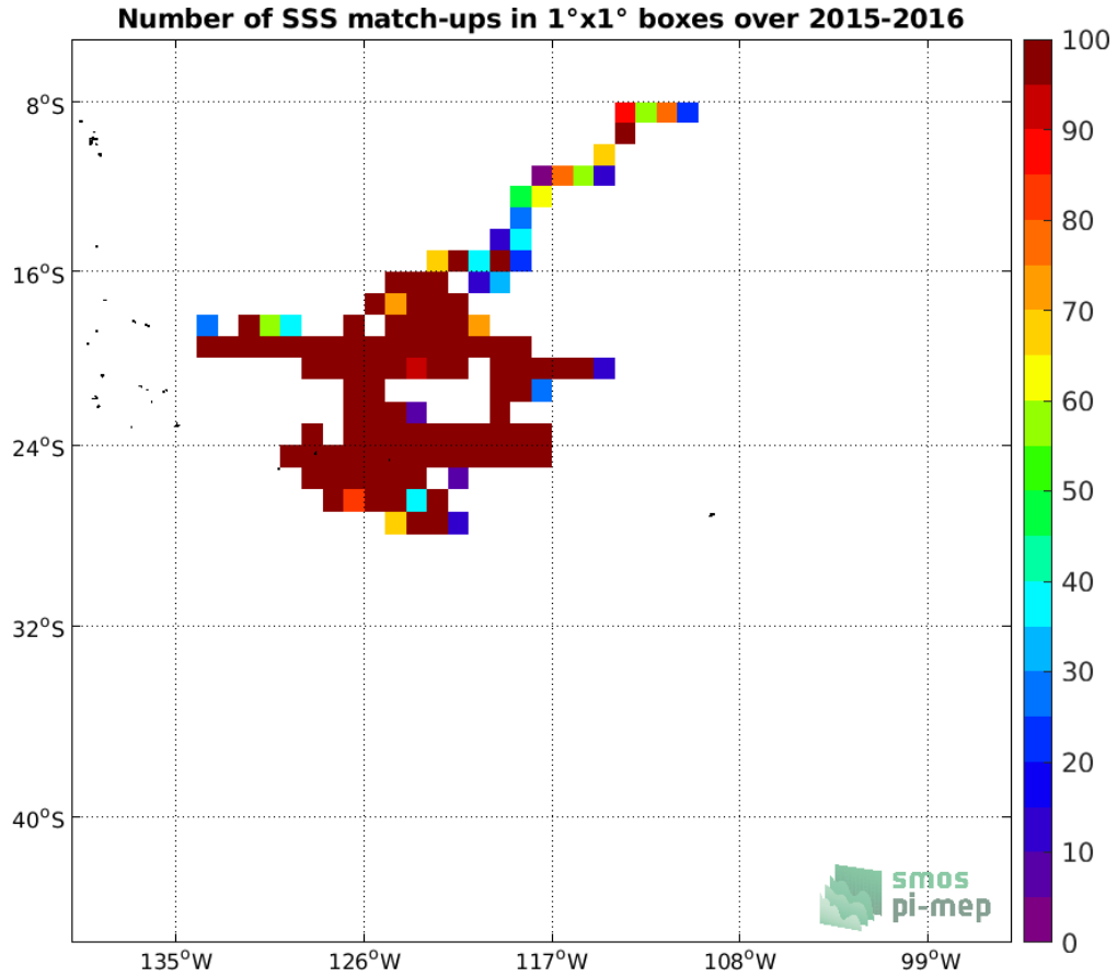
Figure 3: Number of SSS match-ups between Surface drifters SSS and the SMOS SSS L3 v3 Monthly (ICDC) SSS product for the OTT zone Pi-MEP region over 1°x1° boxes and for the full satellite product period.
