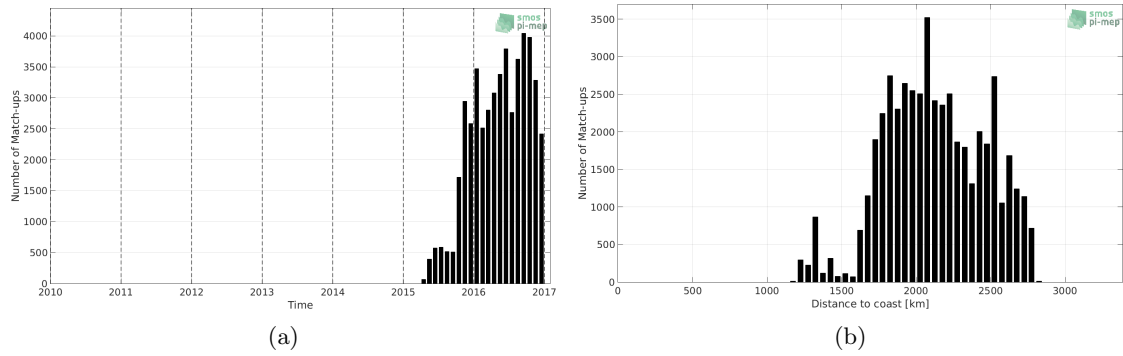
Figure 1: Number of match-ups between Surface drifters and SMOS-L3-ICDC-V3-MONTHLY-0.5DEG SSS as a function of time (a) and as function of the distance to coast (b) over the OTT zone Pi-MEP region and for the full satellite product period.
