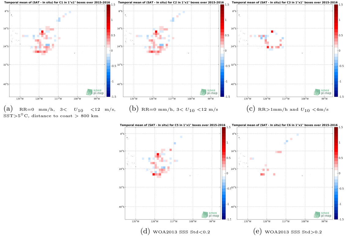
Figure 11: Temporal mean gridded over spatial boxes of size 1^\circ \times 1^\circ of \Delta SSS (SMOS-L3-ICDC-V3-MONTHLY-0.5DEG - Surface drifters) for 5 different subdatasets corresponding to:RR=0 mm/h, 3 < U_{10} < 12 m/s, SST >5^\circ\text{C} , distance to coast > 800 km (a), RR=0 mm/h, 3 < U_{10} < 12 m/s (b), RR >1 mm/h and U_{10} < 4 m/s (c), WOA2013 SSS Std <0.2 (d), WOA2013 SSS Std >0.2 (e).
