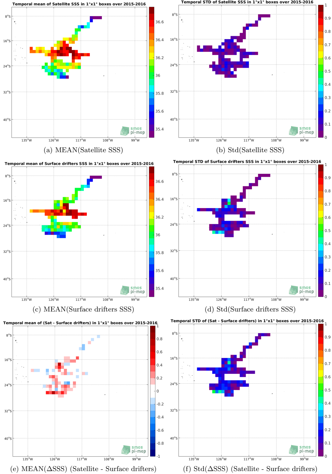
Figure 5: Temporal mean (left) and Std (right) of SSS from SMOS-L3-ICDC-V3-MONTHLY-0.5DEG (top), Surface drifters (middle), and of \Delta SSS (Satellite - Surface drifters). Only match-up pairs are used to generate these maps.
