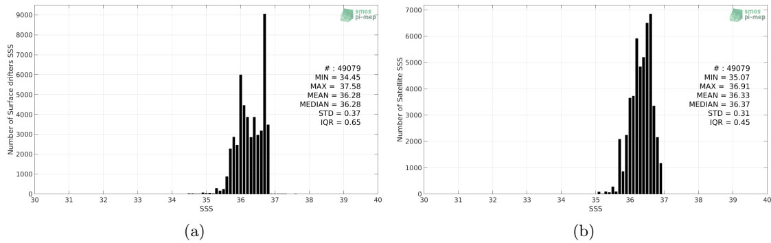
Figure 2: Histograms of SSS from Surface drifters (a) and SMOS-L3-ICDC-V3-MONTHLY-0.5DEG (b) considering all match-up pairs per bins of 0.1 over the OTT zone Pi-MEP region and for the full satellite product period.
