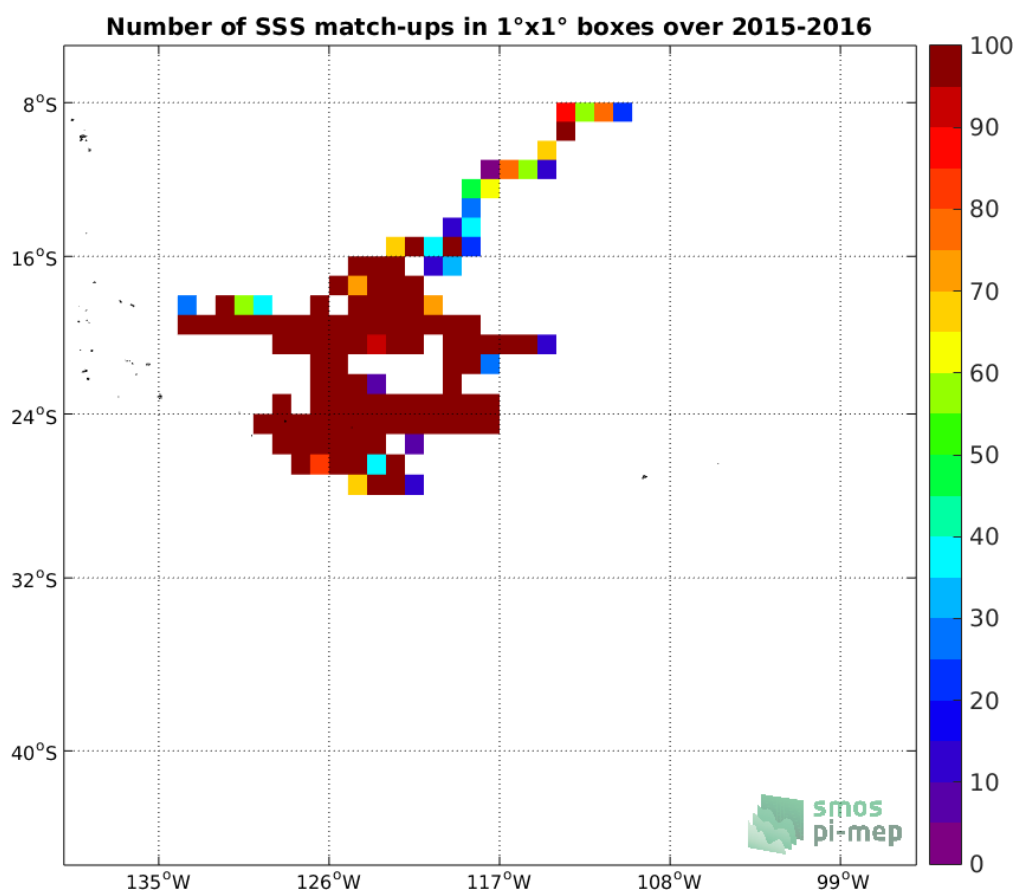
Figure 3: Number of SSS match-ups between Surface drifters SSS and the SMOS-L3-ICDC-V3-MONTHLY-0.5DEG SSS product for the OTT zone Pi-MEP region over 1°x1° boxes and for the full satellite product period.
