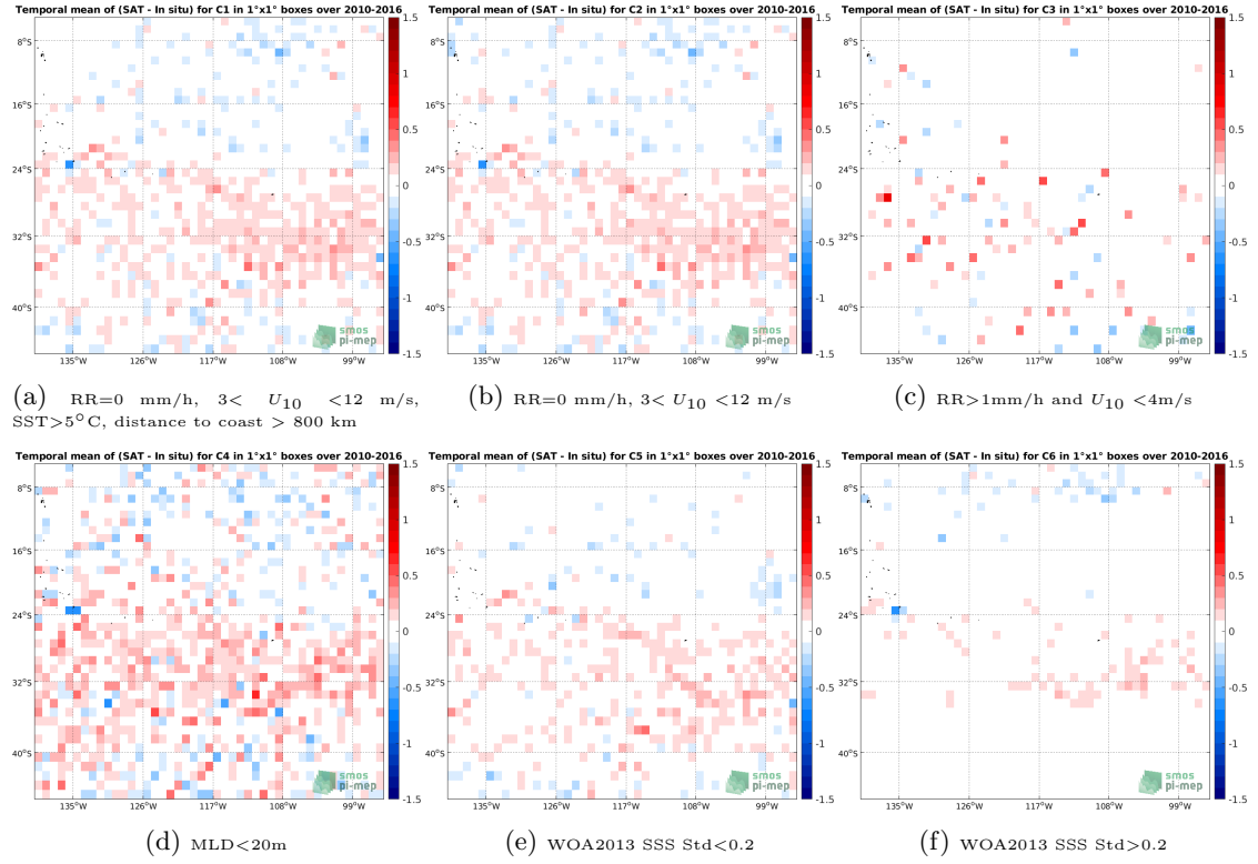
Figure 12: Temporal mean gridded over spatial boxes of size 1^\circ \times 1^\circ of \Delta SSS (SMOS SSS L3 v3 Monthly (ICDC) - Argo) for 6 different subdatasets corresponding to:RR=0 mm/h, 3 < U_{10} < 12 m/s, SST >5^\circ\text{C} , distance to coast > 800 km (a), RR=0 mm/h, 3 < U_{10} < 12 m/s (b), RR >1 mm/h and U_{10} < 4 m/s (c),MLD <20 m (d),WOA2013 SSS Std <0.2 (e),WOA2013 SSS Std >0.2 (f).
