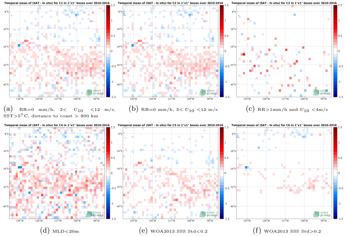
Figure 12: Temporal mean gridded over spatial boxes of size 1^\circ \times 1^\circ of \Delta SSS (SMOS-L3-ICDC-V3-MONTHLY-0.5DEG - Argo) for 6 different subdatasets corresponding to: RR=0 mm/h, 3 < U_{10} < 12 m/s, SST > 5^\circ\text{C} , distance to coast > 800 km (a), RR=0 mm/h, 3 < U_{10} < 12 m/s (b), RR > 1 mm/h and U_{10} < 4 m/s (c), MLD < 20 m (d), WOA2013 SSS Std < 0.2 (e), WOA2013 SSS Std > 0.2 (f).
