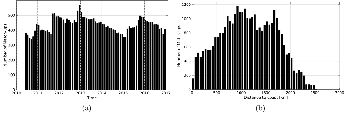
Figure 1: Number of match-ups between Argo and SMOS-L3-ICDC-V3-MONTHLY-0.5DEG SSS as a function of time (a) and as function of the distance to coast (b) over the OTT zone Pi-MEP region and for the full satellite product period.
