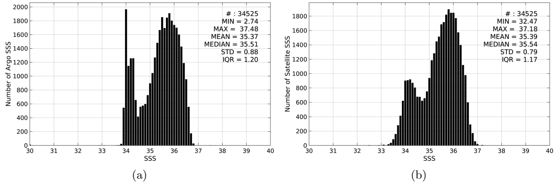
Figure 2: Histograms of SSS from Argo (a) and SMOS-L3-ICDC-V3-MONTHLY-0.5DEG (b) considering all match-up pairs per bins of 0.1 over the OTT zone Pi-MEP region and for the full satellite product period.
