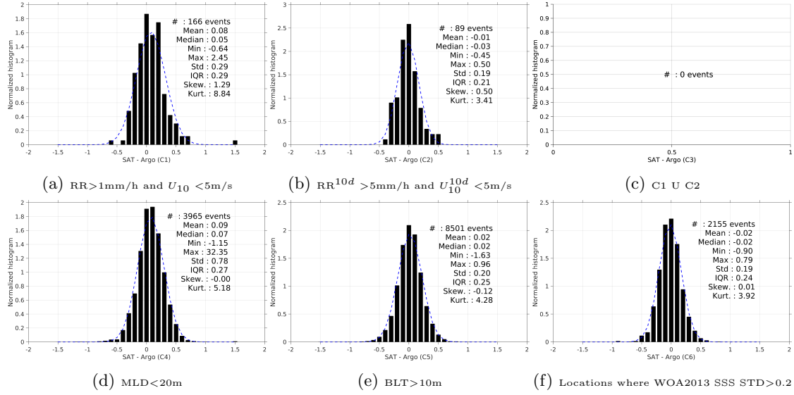
Figure 13: Normalized histogram of \Delta SSS (SMOS-L3-ICDC-V3-MONTHLY-0.5DEG - Argo) for 6 different subdatasets corresponding to: RR > 1\text{mm/h} and U_{10} < 5\text{m/s} (a), RR^{10d} > 5\text{mm/h} and U_{10}^{10d} < 5\text{m/s} (b), C1 \cup C2 (c), MLD < 20\text{m} (d), BLT > 10\text{m} (e), Locations where WOA2013 SSS STD > 0.2 (f).
