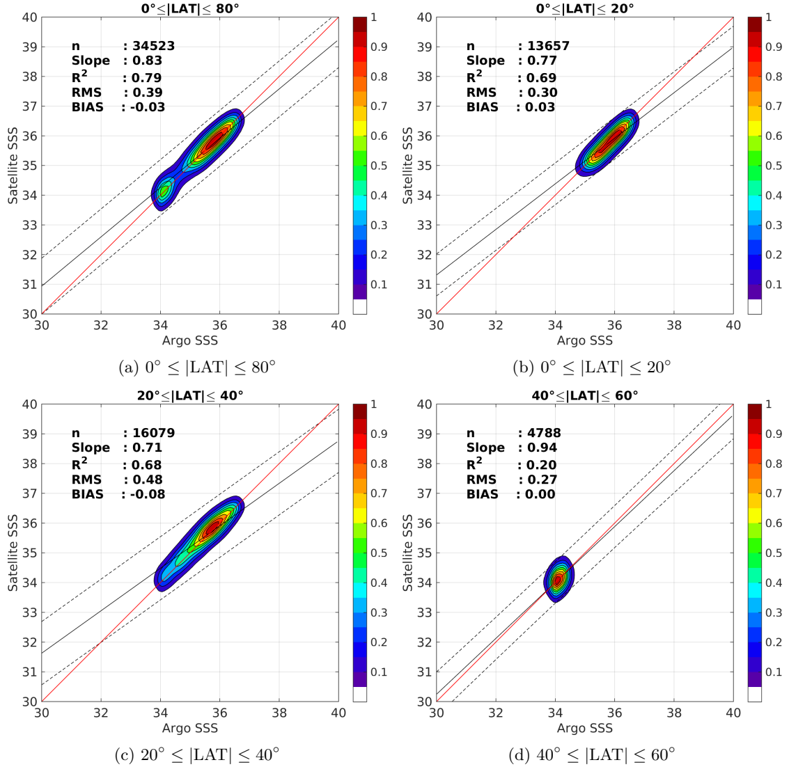
Figure 9: Contour maps of the concentration of SMOS-L3-ICDC-V3-MONTHLY-0.5DEG SSS (y-axis) versus Argo SSS (x-axis) at match-up pairs for different latitude bands. For each plot, the red line shows x=y . The black thin and dashed lines indicate a linear fit through the data cloud and the \pm 95\% confidence levels, respectively. The number match-up pairs n , the slope and R^2 coefficient of the linear fit, the root mean square (RMS) and the mean bias between satellite and in situ data are indicated for each latitude band in each plots.
