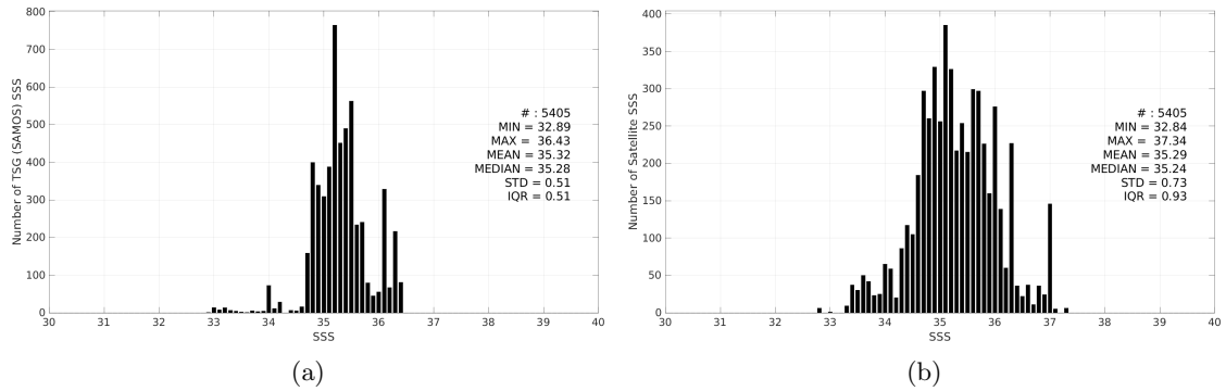
Figure 3: Histograms of SSS from TSG (SAMOS) (a) and SMOS SSS L2Q v331 - With FLAG (CMEMS-CATDS-CPDC) (b) considering all match-up pairs per bins of 0.1 over the OTT zone Pi-MEP region and for the full satellite product period.
