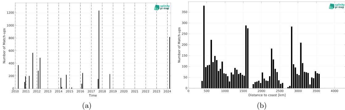
Figure 2: Number of match-ups between TSG (SAMOS) and SMOS SSS L2Q v331 - With FLAG (CMEMS-CATDS-CPDC) SSS as a function of time (a) and as function of the distance to coast (b) over the OTT zone Pi-MEP region and for the full satellite product period.
