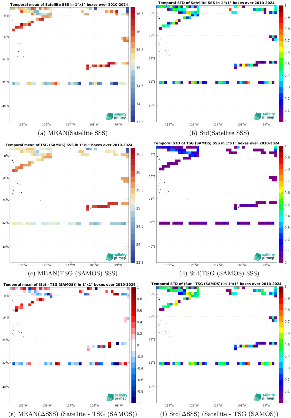
Figure 7: Temporal mean (left) and Std (right) of SSS from SMOS SSS L2Q v331 - With FLAG (CMEMS-CATDS-CPDC) (top), TSG (SAMOS) (middle), and of \Delta SSS (Satellite - TSG (SAMOS)). Only match-up pairs are used to generate these maps.
