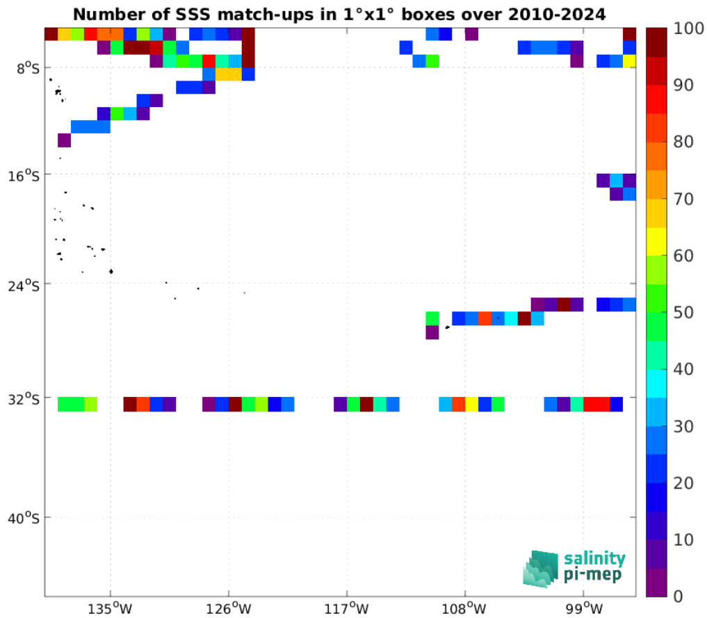
Figure 5: Number of SSS match-ups between TSG (SAMOS) SSS and the SMOS SSS L2Q v331 - With FLAG (CMEMS-CATDS-CPDC) SSS product for the OTT zone Pi-MEP region over 1^\circ \times 1^\circ boxes and for the full satellite product period.
