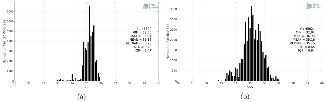
Figure 2: Histograms of SSS from TSG (SAMOS) (a) and SMOS SSS L2Q v331 - With FLAG (CMEMS-CATDS-CPDC) (b) considering all match-up pairs per bins of 0.1 over the OTT zone Pi-MEP region and for the full satellite product period.
