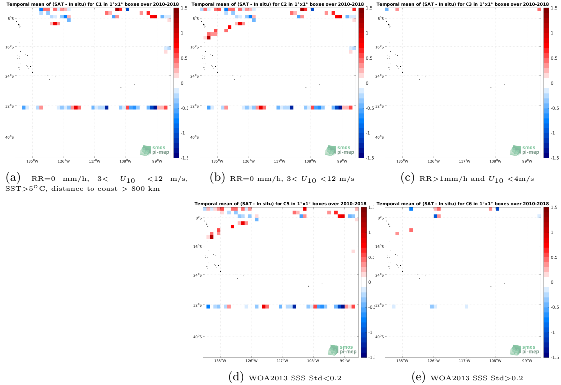
Figure 12: Temporal mean gridded over spatial boxes of size 1^{\circ}\times 1^{\circ} of \Delta\text{SSS} (SMOS SSS L2Q v331 - With FLAG (CMEMS-CATDS-CPDC) - TSG (SAMOS)) for 5 different subdatasets corresponding to:RR=0 mm/h, 3 < U_{10} < 12 m/s, SST >5^{\circ}\text{C} , distance to coast > 800 km (a), RR=0 mm/h, 3 < U_{10} < 12 m/s (b), RR >1 mm/h and U_{10} < 4 m/s (c), WOA2013 SSS Std <0.2 (d), WOA2013 SSS Std >0.2 (e).
