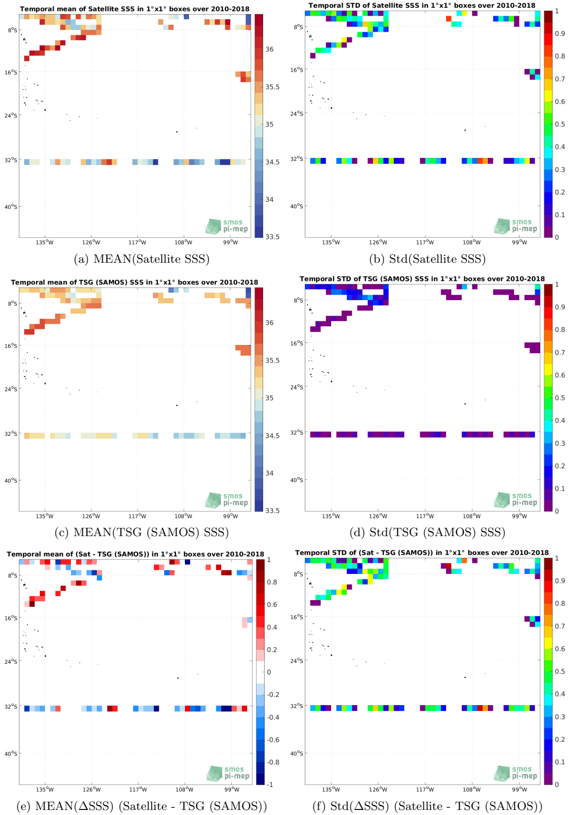
Figure 6: Temporal mean (left) and Std (right) of SSS from SMOS SSS L2Q v331 - With FLAG (CMEMS-CATDS-CPDC) (top), TSG (SAMOS) (middle), and of \Delta SSS (Satellite - TSG (SAMOS)). Only match-up pairs are used to generate these maps.
