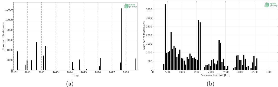
Figure 1: Number of match-ups between TSG (SAMOS) and SMOS SSS L2Q v331 - With FLAG (CMEMS-CATDS-CPDC) SSS as a function of time (a) and as function of the distance to coast (b) over the OTT zone Pi-MEP region and for the full satellite product period.
