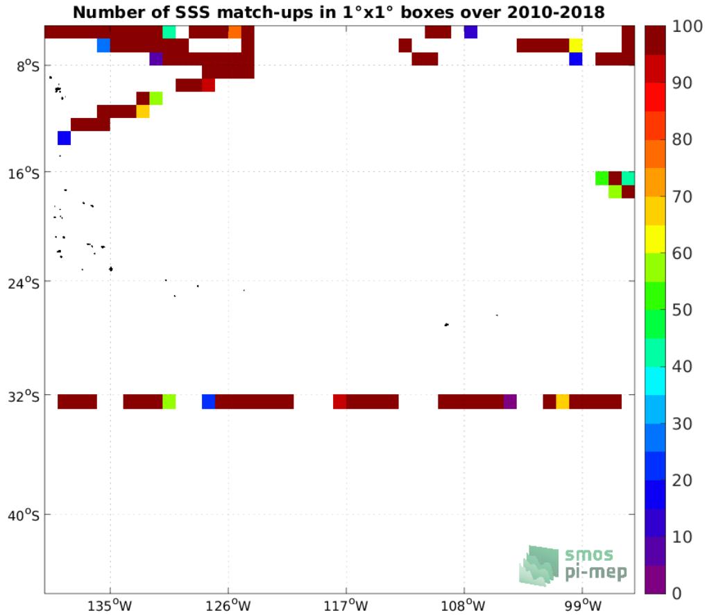
Figure 4: Number of SSS match-ups between TSG (SAMOS) SSS and the SMOS SSS L2Q v331 - With FLAG (CMEMS-CATDS-CPDC) SSS product for the OTT zone Pi-MEP region over 1^\circ \times 1^\circ boxes and for the full satellite product period.
