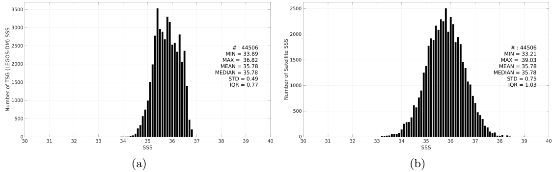
Figure 3: Histograms of SSS from TSG (LEGOS-DM) (a) and SMOS SSS L2Q v331 - With FLAG (CMEMS-CATDS-CPDC) (b) considering all match-up pairs per bins of 0.1 over the OTT zone Pi-MEP region and for the full satellite product period.
