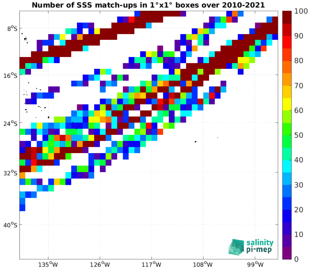
Figure 5: Number of SSS match-ups between TSG (LEGOS-DM) SSS and the SMOS SSS L2Q v331 - With FLAG (CMEMS-CATDS-CPDC) SSS product for the OTT zone Pi-MEP region over 1^\circ \times 1^\circ boxes and for the full satellite product period.
