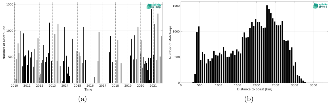
Figure 2: Number of match-ups between TSG (LEGOS-DM) and SMOS SSS L2Q v331 - With FLAG (CMEMS-CATDS-CPDC) SSS as a function of time (a) and as function of the distance to coast (b) over the OTT zone Pi-MEP region and for the full satellite product period.
