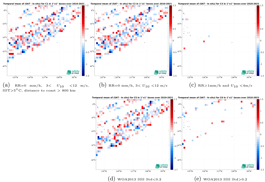
Figure 14: Temporal mean gridded over spatial boxes of size 1^\circ \times 1^\circ of \Delta SSS (SMOS SSS L2Q v331 - With FLAG (CMEMS-CATDS-CPDC) - TSG (LEGOS-DM)) for 5 different subdatasets corresponding to:RR=0 mm/h, 3 < U_{10} < 12 m/s, SST >5^\circ\text{C} , distance to coast > 800 km (a), RR=0 mm/h, 3 < U_{10} < 12 m/s (b), RR >1 mm/h and U_{10} < 4 m/s (c), WOA2013 SSS Std <0.2 (d), WOA2013 SSS Std >0.2 (e).
