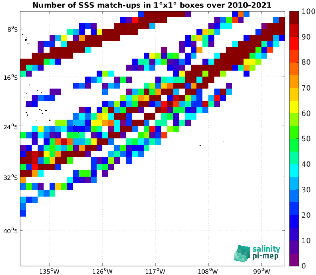
Figure 4: Number of SSS match-ups between TSG (LEGOS-DM) SSS and the SMOS SSS L2Q v331 - With FLAG (CMEMS-CATDS-CPDC) SSS product for the OTT zone Pi-MEP region over 1^\circ \times 1^\circ boxes and for the full satellite product period.
