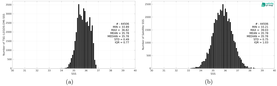
Figure 2: Histograms of SSS from TSG (LEGOS-DM) (a) and SMOS SSS L2Q v331 - With FLAG (CMEMS-CATDS-CPDC) (b) considering all match-up pairs per bins of 0.1 over the OTT zone Pi-MEP region and for the full satellite product period.
