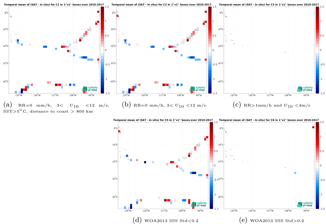
Figure 12: Temporal mean gridded over spatial boxes of size 1^\circ \times 1^\circ of \Delta SSS (SMOS SSS L2Q v331 - With FLAG (CMEMS-CATDS-CPDC) - TSG (GOSUD-Sailing-ship)) for 5 different subdatasets corresponding to: RR=0 mm/h, 3 < U_{10} < 12 m/s, SST > 5^\circ C , distance to coast > 800 km (a), RR=0 mm/h, 3 < U_{10} < 12 m/s (b), RR > 1 mm/h and U_{10} < 4 m/s (c), WOA2013 SSS Std < 0.2 (d), WOA2013 SSS Std > 0.2 (e).
