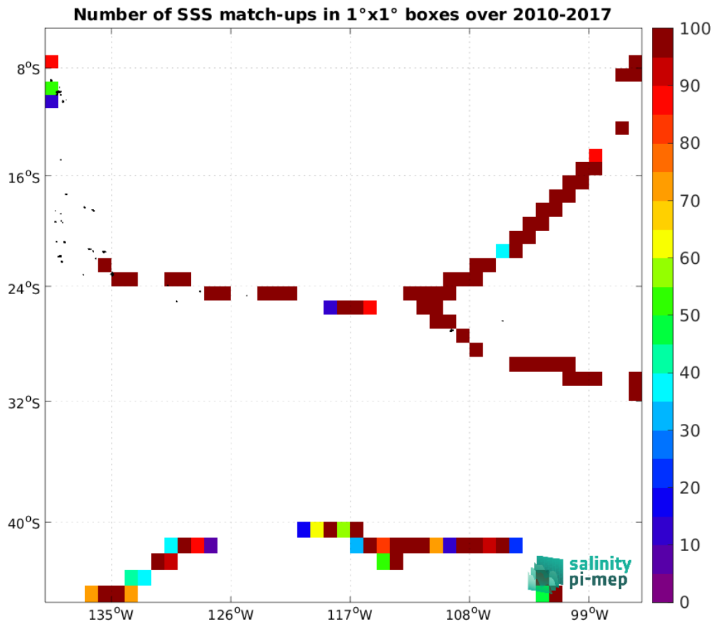
Figure 4: Number of SSS match-ups between TSG (GOSUD-Sailing-ship) SSS and the SMOS SSS L2Q v331 - With FLAG (CMEMS-CATDS-CPDC) SSS product for the OTT zone Pi-MEP region over 1°x1° boxes and for the full satellite product period.
