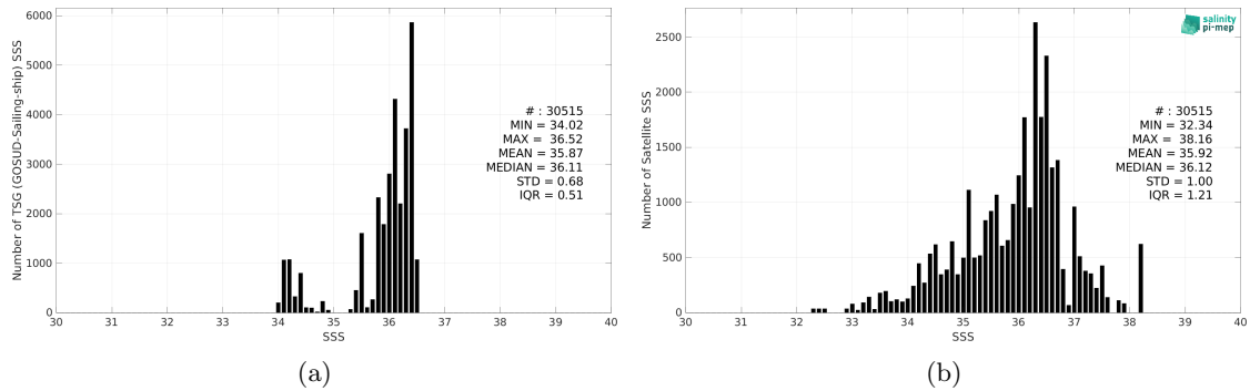
Figure 2: Histograms of SSS from TSG (GOSUD-Sailing-ship) (a) and SMOS SSS L2Q v331 - With FLAG (CMEMS-CATDS-CPDC) (b) considering all match-up pairs per bins of 0.1 over the OTT zone Pi-MEP region and for the full satellite product period.
