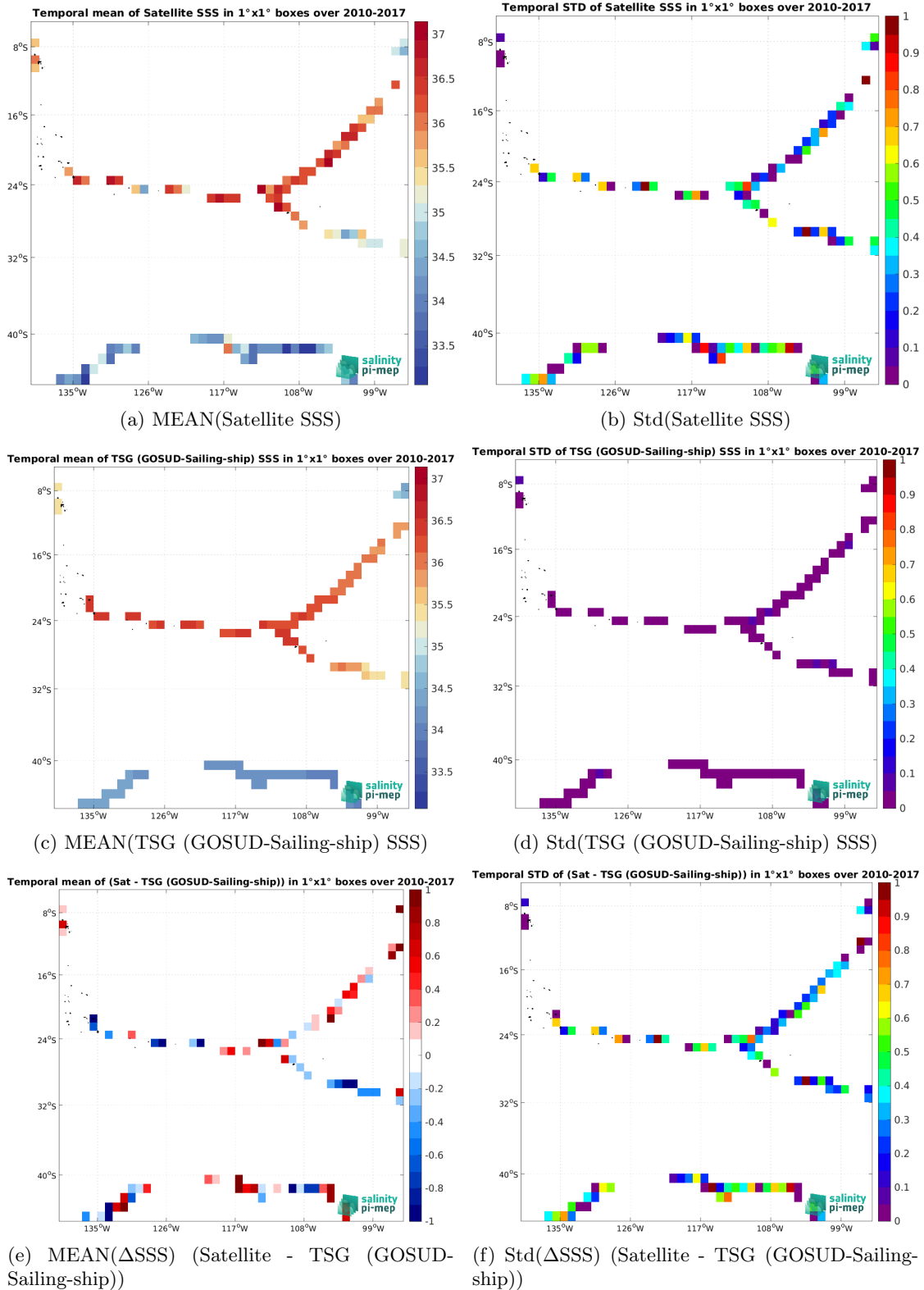
Figure 6: Temporal mean (left) and Std (right) of SSS from SMOS SSS L2Q v331 - With FLAG (CMEMS-CATDS-CPDC) (top), TSG (GOSUD-Sailing-ship) (middle), and of \Delta SSS (Satellite - TSG (GOSUD-Sailing-ship)). Only match-up pairs are used to generate these maps.
