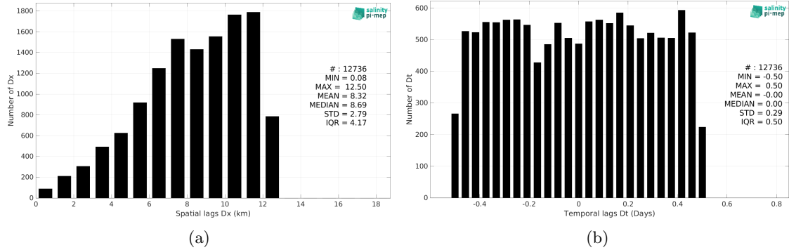
Figure 6: Histograms of the spatial (a) and temporal (b) lags between the location/time of the TSG (GOSUD-Research-vessel) measurement and the date of the corresponding SMOS SSS L2Q v331 - With FLAG (CMEMS-CATDS-CPDC) SSS pixel.
