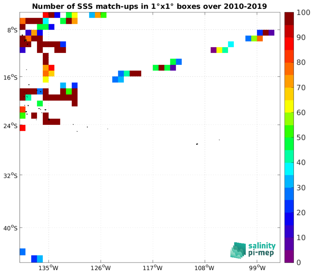
Figure 5: Number of SSS match-ups between TSG (GOSUD-Research-vessel) SSS and the SMOS SSS L2Q v331 - With FLAG (CMEMS-CATDS-CPDC) SSS product for the OTT zone Pi-MEP region over 1^\circ \times 1^\circ boxes and for the full satellite product period.
