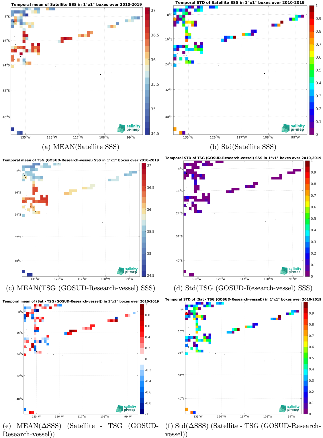
Figure 7: Temporal mean (left) and Std (right) of SSS from SMOS SSS L2Q v331 - With FLAG (CMEMS-CATDS-CPDC) (top), TSG (GOSUD-Research-vessel) (middle), and of \Delta SSS (Satellite - TSG (GOSUD-Research-vessel)). Only match-up pairs are used to generate these maps.
