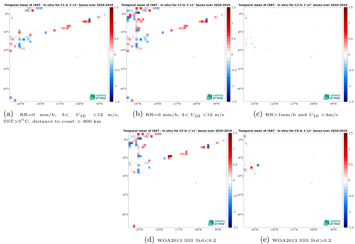
Figure 14: Temporal mean gridded over spatial boxes of size 1^\circ \times 1^\circ of \Delta SSS (SMOS SSS L2Q v331 - With FLAG (CMEMS-CATDS-CPDC) - TSG (GOSUD-Research-vessel)) for 5 different subdatasets corresponding to:RR=0 mm/h, 3 < U_{10} < 12 m/s, SST >5^\circ\text{C} , distance to coast > 800 km (a), RR=0 mm/h, 3 < U_{10} < 12 m/s (b), RR >1 mm/h and U_{10} < 4 m/s (c), WOA2013 SSS Std <0.2 (d), WOA2013 SSS Std >0.2 (e).
