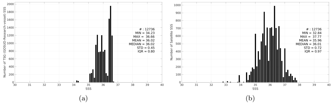
Figure 3: Histograms of SSS from TSG (GOSUD-Research-vessel) (a) and SMOS SSS L2Q v331 - With FLAG (CMEMS-CATDS-CPDC) (b) considering all match-up pairs per bins of 0.1 over the OTT zone Pi-MEP region and for the full satellite product period.
