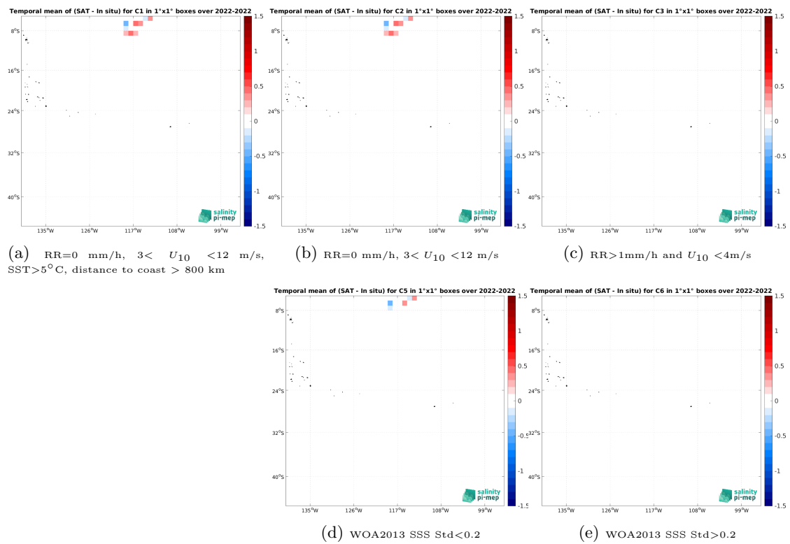
Figure 14: Temporal mean gridded over spatial boxes of size 1^\circ \times 1^\circ of \Delta SSS (SMOS SSS L2Q v331 - With FLAG (CMEMS-CATDS-CPDC) - Saildrone) for 5 different subdatasets corresponding to:RR=0 mm/h, 3 < U_{10} < 12 m/s, SST >5^\circ C, distance to coast > 800 km (a), RR=0 mm/h, 3 < U_{10} < 12 m/s (b), RR >1 mm/h and U_{10} < 4 m/s (c), WOA2013 SSS Std <0.2 (d), WOA2013 SSS Std >0.2 (e).
