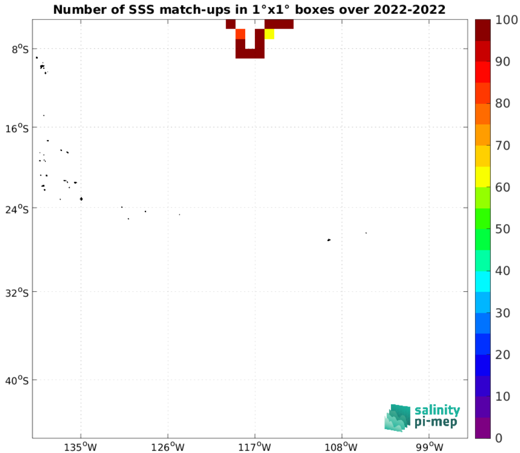
Figure 5: Number of SSS match-ups between Saildrone SSS and the SMOS SSS L2Q v331 - With FLAG (CMEMS-CATDS-CPDC) SSS product for the OTT zone Pi-MEP region over 1^\circ \times 1^\circ boxes and for the full satellite product period.
