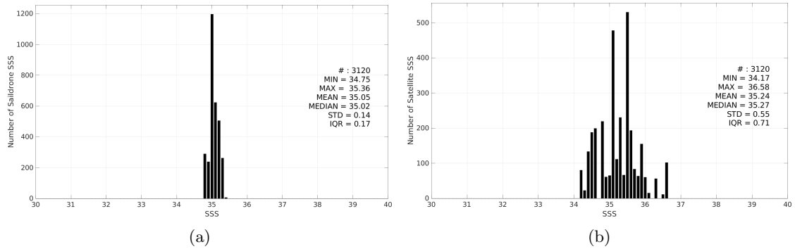
Figure 3: Histograms of SSS from Saildrone (a) and SMOS SSS L2Q v331 - With FLAG (CMEMS-CATDS-CPDC) (b) considering all match-up pairs per bins of 0.1 over the OTT zone Pi-MEP region and for the full satellite product period.
