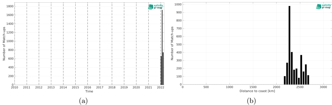
Figure 1: Number of match-ups between Saildrone and SMOS SSS L2Q v331 - With FLAG (CMEMS-CATDS-CPDC) SSS as a function of time (a) and as function of the distance to coast (b) over the OTT zone Pi-MEP region and for the full satellite product period.
