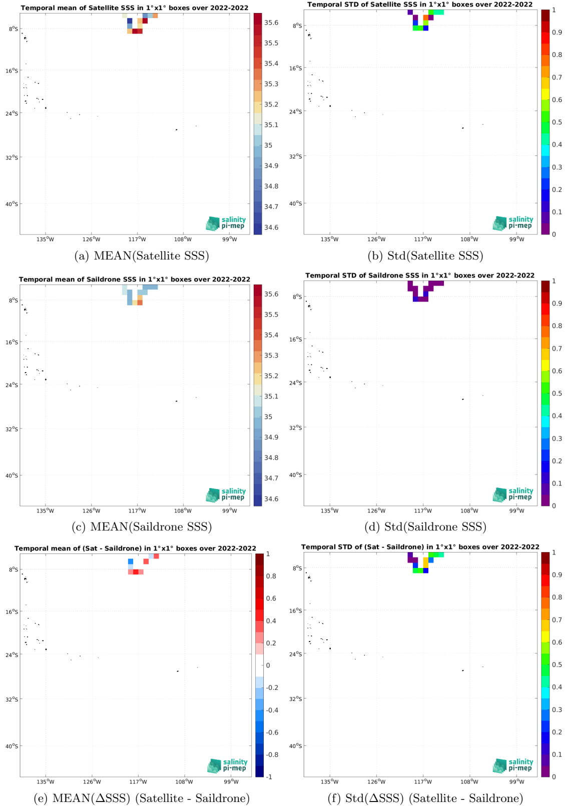
Figure 6: Temporal mean (left) and Std (right) of SSS from SMOS SSS L2Q v331 - With FLAG (CMEMS-CATDS-CPDC) (top), Saildrone (middle), and of \Delta SSS (Satellite - Saildrone). Only match-up pairs are used to generate these maps.
