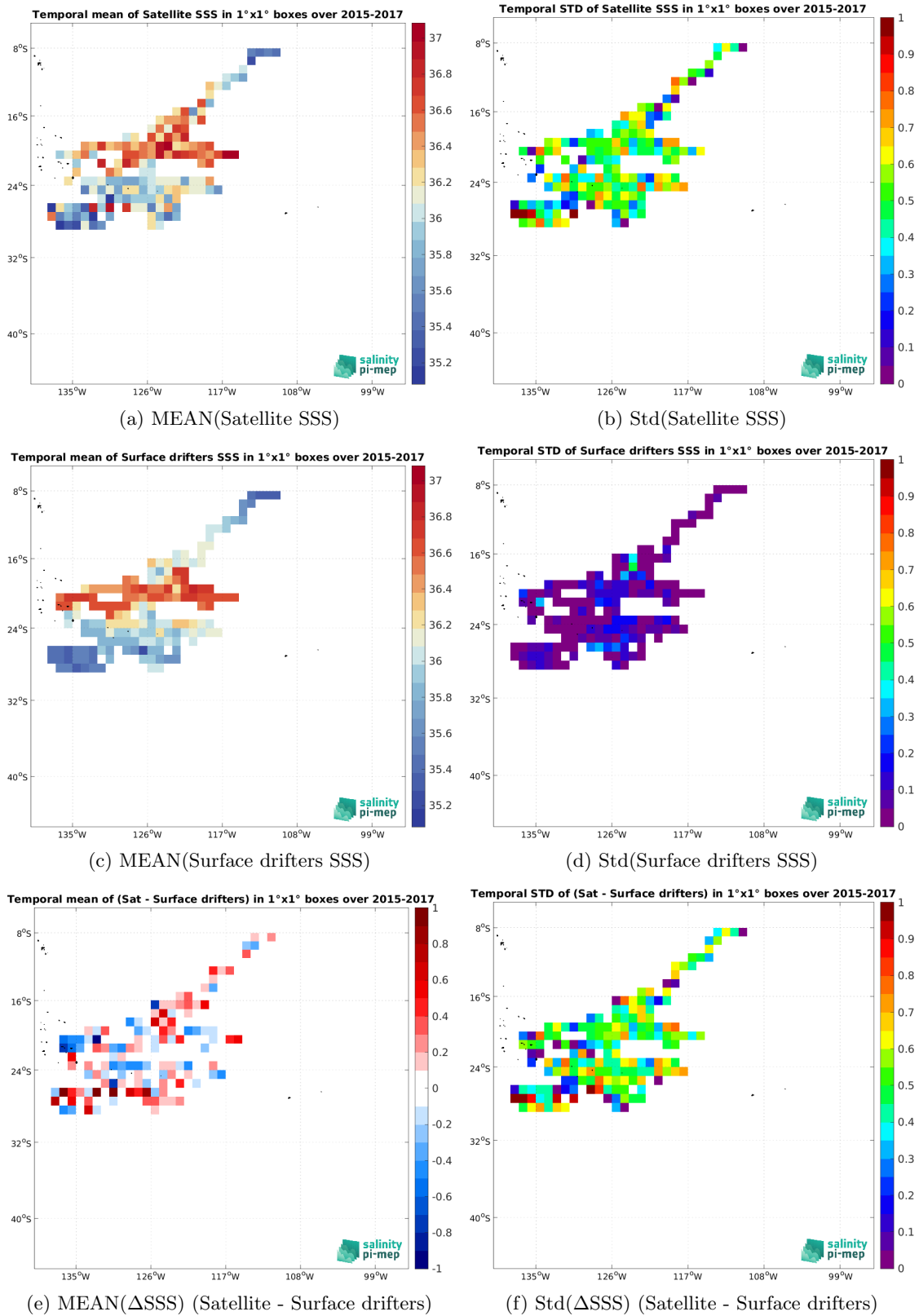
Figure 6: Temporal mean (left) and Std (right) of SSS from SMOS SSS L2Q v331 - With FLAG (CMEMS-CATDS-CPDC) (top), Surface drifters (middle), and of \Delta SSS (Satellite - Surface drifters). Only match-up pairs are used to generate these maps.
