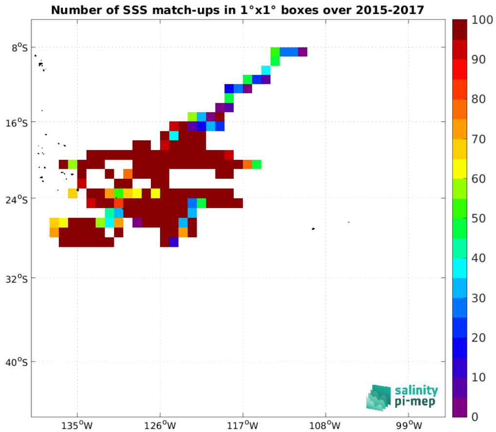
Figure 4: Number of SSS match-ups between Surface drifters SSS and the SMOS SSS L2Q v331 - With FLAG (CMEMS-CATDS-CPDC) SSS product for the OTT zone Pi-MEP region over 1°x1° boxes and for the full satellite product period.
