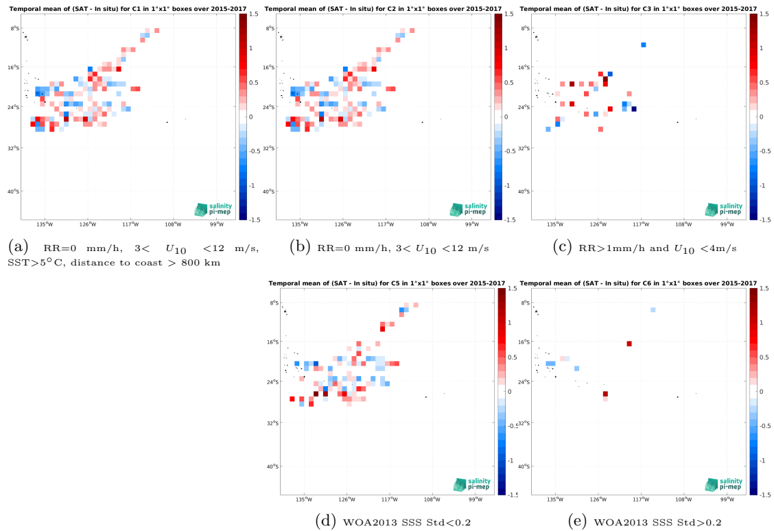
Figure 13: Temporal mean gridded over spatial boxes of size 1^\circ \times 1^\circ of \Delta SSS (SMOS SSS L2Q v331 - With FLAG (CMEMS-CATDS-CPDC) - Surface drifters) for 5 different subdatasets corresponding to:RR=0 mm/h, 3 < U_{10} < 12 m/s, SST >5^\circ\text{C} , distance to coast > 800 km (a), RR=0 mm/h, 3 < U_{10} < 12 m/s (b), RR >1 mm/h and U_{10} < 4 m/s (c), WOA2013 SSS Std <0.2 (d), WOA2013 SSS Std >0.2 (e).
