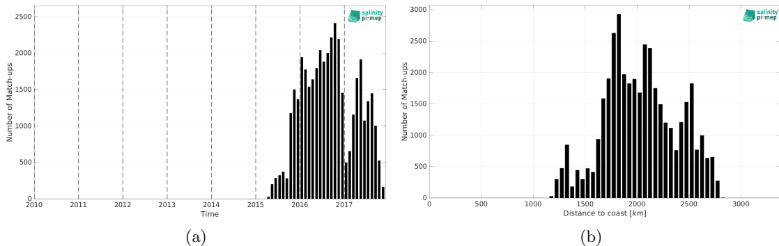
Figure 2: Number of match-ups between Surface drifters and SMOS SSS L2Q v331 - With FLAG (CMEMS-CATDS-CPDC) SSS as a function of time (a) and as function of the distance to coast (b) over the OTT zone Pi-MEP region and for the full satellite product period.
