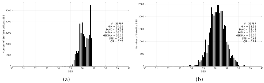
Figure 3: Histograms of SSS from Surface drifters (a) and SMOS SSS L2Q v331 - With FLAG (CMEMS-CATDS-CPDC) (b) considering all match-up pairs per bins of 0.1 over the OTT zone Pi-MEP region and for the full satellite product period.
