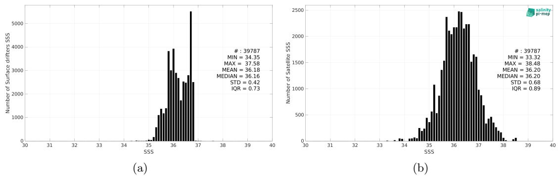
Figure 2: Histograms of SSS from Surface drifters (a) and SMOS SSS L2Q v331 - With FLAG (CMEMS-CATDS-CPDC) (b) considering all match-up pairs per bins of 0.1 over the OTT zone Pi-MEP region and for the full satellite product period.
