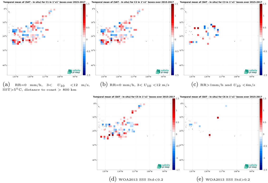
Figure 11: Temporal mean gridded over spatial boxes of size 1^{\circ}\times 1^{\circ} of \Delta\text{SSS} (SMOS SSS L2Q v331 - With FLAG (CMEMS-CATDS-CPDC) - Surface drifters) for 5 different subdatasets corresponding to:RR=0 mm/h, 3 < U_{10} < 12 m/s, SST >5^{\circ}\text{C} , distance to coast > 800 km (a), RR=0 mm/h, 3 < U_{10} < 12 m/s (b), RR >1\text{mm/h} and U_{10} < 4\text{m/s} (c), WOA2013 SSS Std <0.2 (d), WOA2013 SSS Std >0.2 (e).
