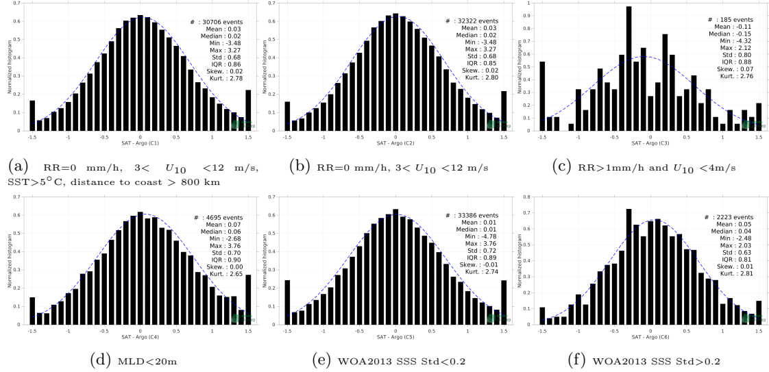
Figure 13: Normalized histogram of \Delta SSS (SMOS SSS L2Q v331 - With FLAG (CMEMS-CATDS-CPDC) - Argo) for 6 different subdatasets corresponding to: RR=0 mm/h, 3 < U_{10} < 12 m/s, SST>5°C, distance to coast > 800 km (a), RR=0 mm/h, 3 < U_{10} < 12 m/s (b), RR>1mm/h and U_{10} < 4 m/s (c), MLD<20m (d), WOA2013 SSS Std<0.2 (e), WOA2013 SSS Std>0.2 (f).
