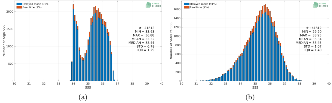
Figure 2: Histograms of SSS from Argo (a) and SMOS SSS L2Q v331 - With FLAG (CMEMS-CATDS-CPDC) (b) considering all match-up pairs per bins of 0.1 over the OTT zone Pi-MEP region and for the full satellite product period.
