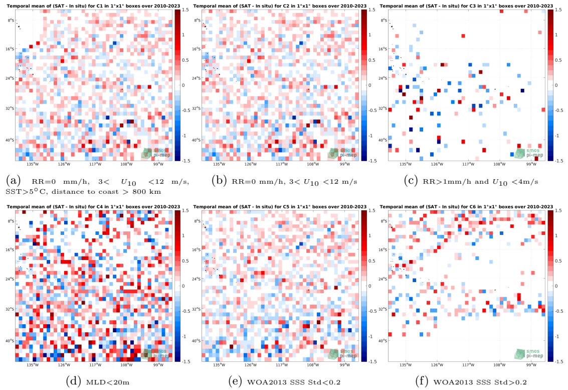
Figure 12: Temporal mean gridded over spatial boxes of size 1^\circ \times 1^\circ of \Delta SSS (SMOS SSS L2Q v331 - With FLAG (CMEMS-CATDS-CPDC) - Argo) for 6 different subdatasets corresponding to:RR=0 mm/h, 3 < U_{10} < 12 m/s, SST >5^\circ C, distance to coast > 800 km (a), RR=0 mm/h, 3 < U_{10} < 12 m/s (b), RR >1 mm/h and U_{10} < 4 m/s (c),MLD <20 m (d),WOA2013 SSS Std <0.2 (e),WOA2013 SSS Std >0.2 (f).
