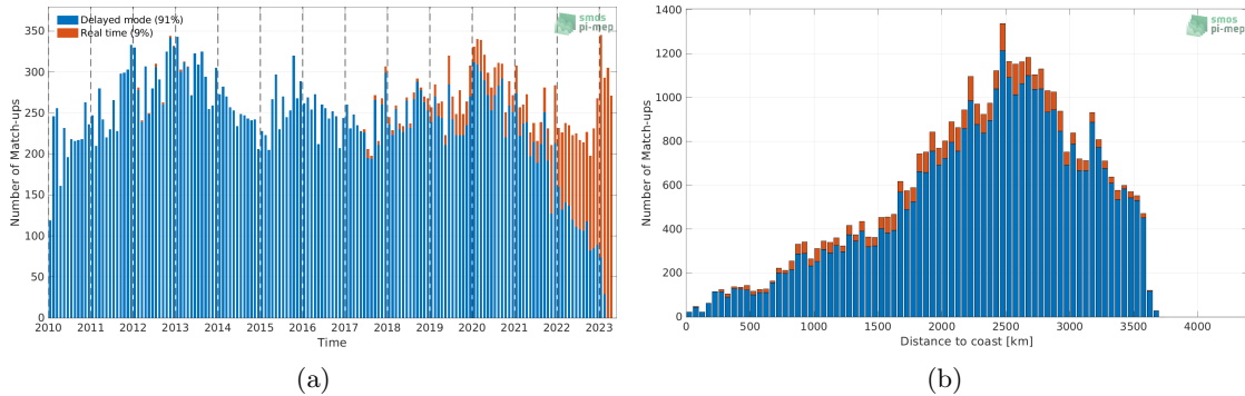
Figure 1: Number of match-ups between Argo and SMOS SSS L2Q v331 - With FLAG (CMEMS-CATDS-CPDC) SSS as a function of time (a) and as function of the distance to coast (b) over the OTT zone Pi-MEP region and for the full satellite product period.
