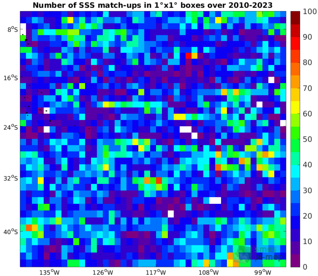
Figure 4: Number of SSS match-ups between Argo SSS and the SMOS SSS L2Q v331 - With FLAG (CMEMS-CATDS-CPDC) SSS product for the OTT zone Pi-MEP region over 1^\circ \times 1^\circ boxes and for the full satellite product period.
