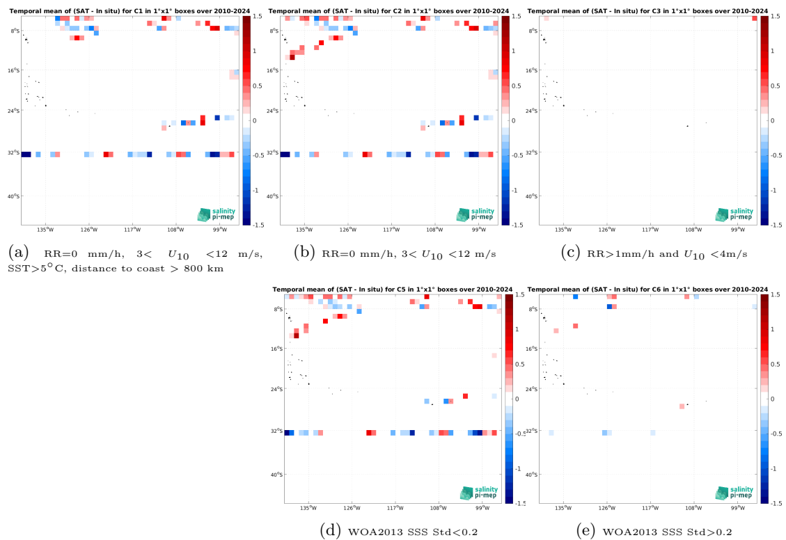
Figure 14: Temporal mean gridded over spatial boxes of size 1^\circ \times 1^\circ of \Delta SSS (SMOS SSS L2Q v331 - No FLAG (CMEMS-CATDS-CPDC) - TSG (SAMOS)) for 5 different subdatasets corresponding to: RR=0 mm/h, 3 < U_{10} < 12 m/s, SST > 5^\circ C , distance to coast > 800 km (a), RR=0 mm/h, 3 < U_{10} < 12 m/s (b), RR > 1 mm/h and U_{10} < 4 m/s (c), WOA2013 SSS Std < 0.2 (d), WOA2013 SSS Std > 0.2 (e).
