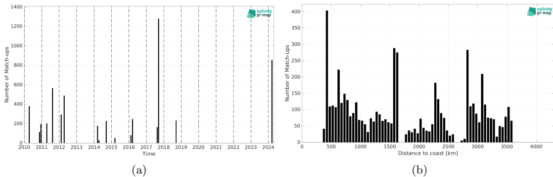
Figure 2: Number of match-ups between TSG (SAMOS) and SMOS SSS L2Q v331 - No FLAG (CMEMS-CATDS-CPDC) SSS as a function of time (a) and as function of the distance to coast (b) over the OTT zone Pi-MEP region and for the full satellite product period.
