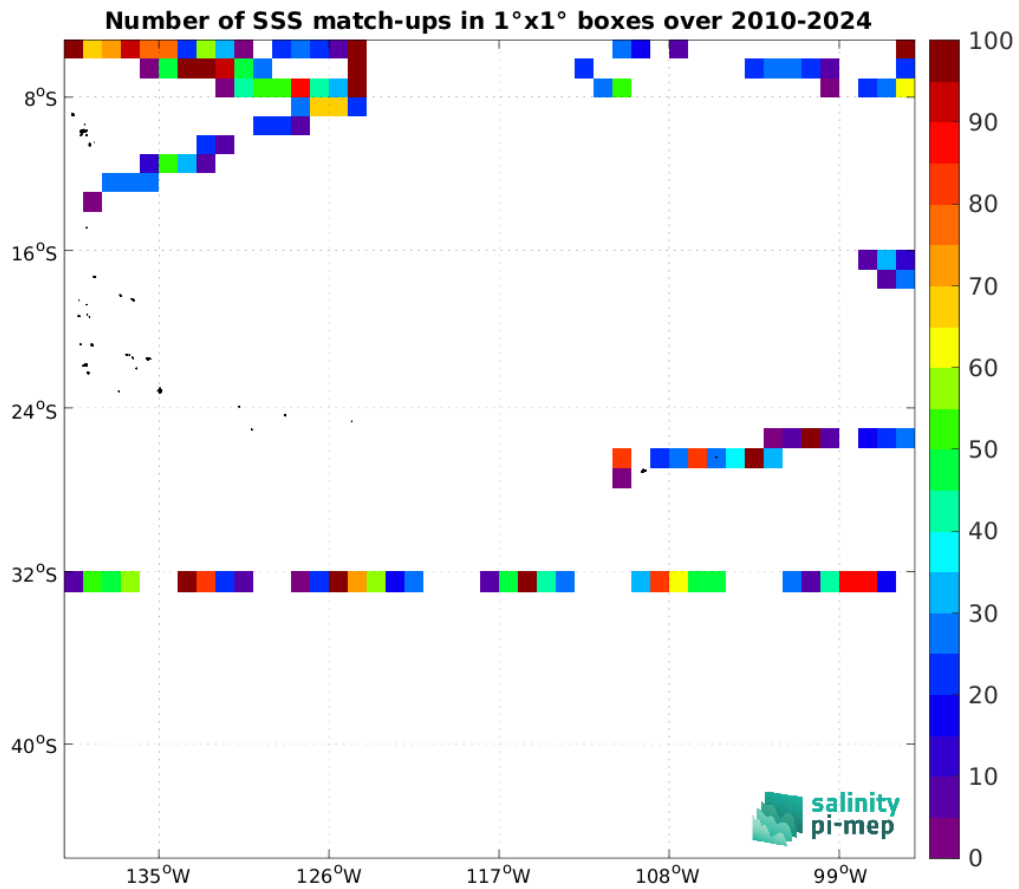
Figure 5: Number of SSS match-ups between TSG (SAMOS) SSS and the SMOS SSS L2Q v331 - No FLAG (CMEMS-CATDS-CPDC) SSS product for the OTT zone Pi-MEP region over 1^\circ \times 1^\circ boxes and for the full satellite product period.
