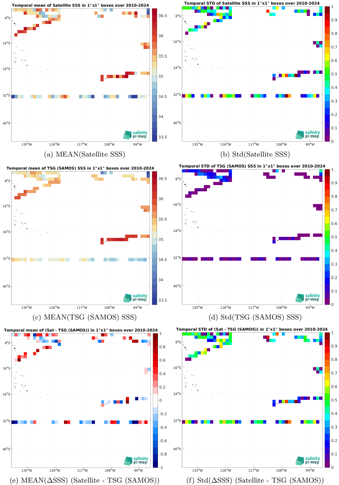
Figure 7: Temporal mean (left) and Std (right) of SSS from SMOS SSS L2Q v331 - No FLAG (CMEMS-CATDS-CPDC) (top), TSG (SAMOS) (middle), and of \Delta SSS (Satellite - TSG (SAMOS)). Only match-up pairs are used to generate these maps.
