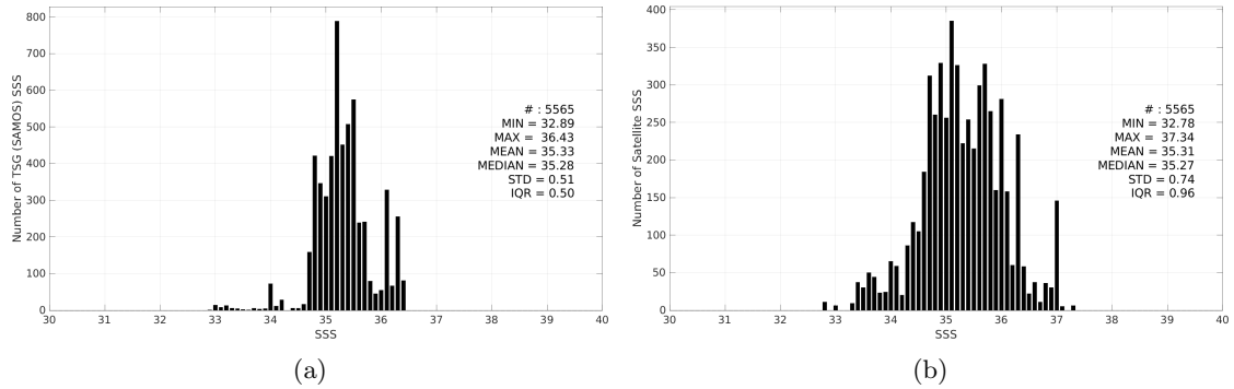
Figure 3: Histograms of SSS from TSG (SAMOS) (a) and SMOS SSS L2Q v331 - No FLAG (CMEMS-CATDS-CPDC) (b) considering all match-up pairs per bins of 0.1 over the OTT zone Pi-MEP region and for the full satellite product period.
