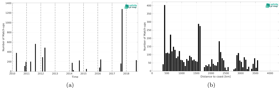
Figure 1: Number of match-ups between TSG (SAMOS) and SMOS SSS L2Q v331 - No FLAG (CMEMS-CATDS-CPDC) SSS as a function of time (a) and as function of the distance to coast (b) over the OTT zone Pi-MEP region and for the full satellite product period.
