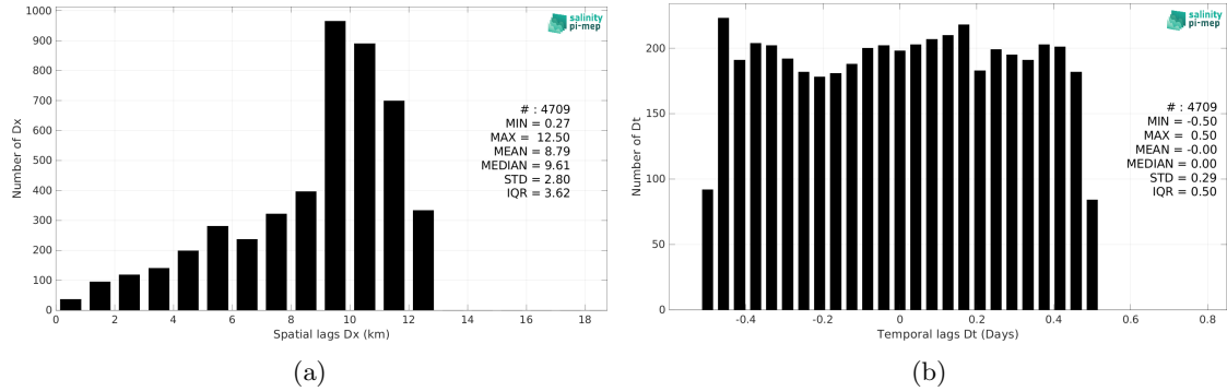
Figure 5: Histograms of the spatial (a) and temporal (b) lags between the location/time of the TSG (SAMOS) measurement and the date of the corresponding SMOS SSS L2Q v331 - No FLAG (CMEMS-CATDS-CPDC) SSS pixel.
