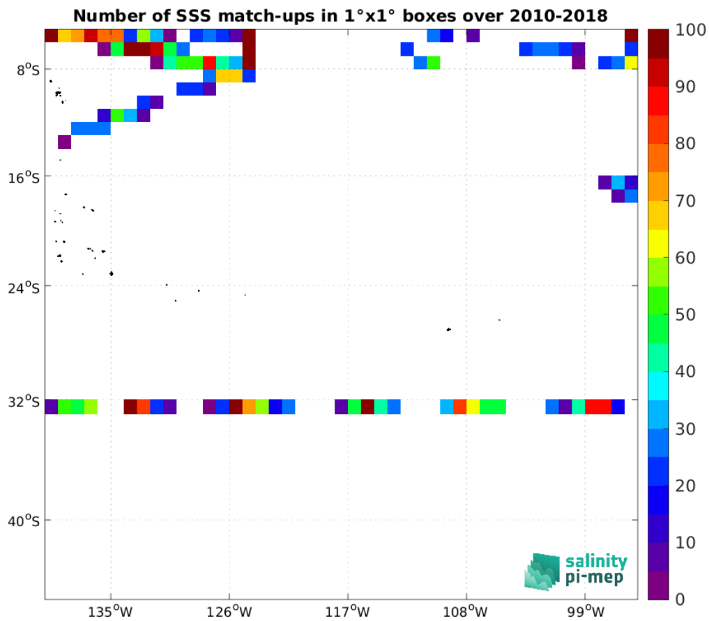
Figure 4: Number of SSS match-ups between TSG (SAMOS) SSS and the SMOS SSS L2Q v331 - No FLAG (CMEMS-CATDS-CPDC) SSS product for the OTT zone Pi-MEP region over 1^\circ \times 1^\circ boxes and for the full satellite product period.
