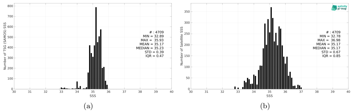
Figure 2: Histograms of SSS from TSG (SAMOS) (a) and SMOS SSS L2Q v331 - No FLAG (CMEMS-CATDS-CPDC) (b) considering all match-up pairs per bins of 0.1 over the OTT zone Pi-MEP region and for the full satellite product period.
