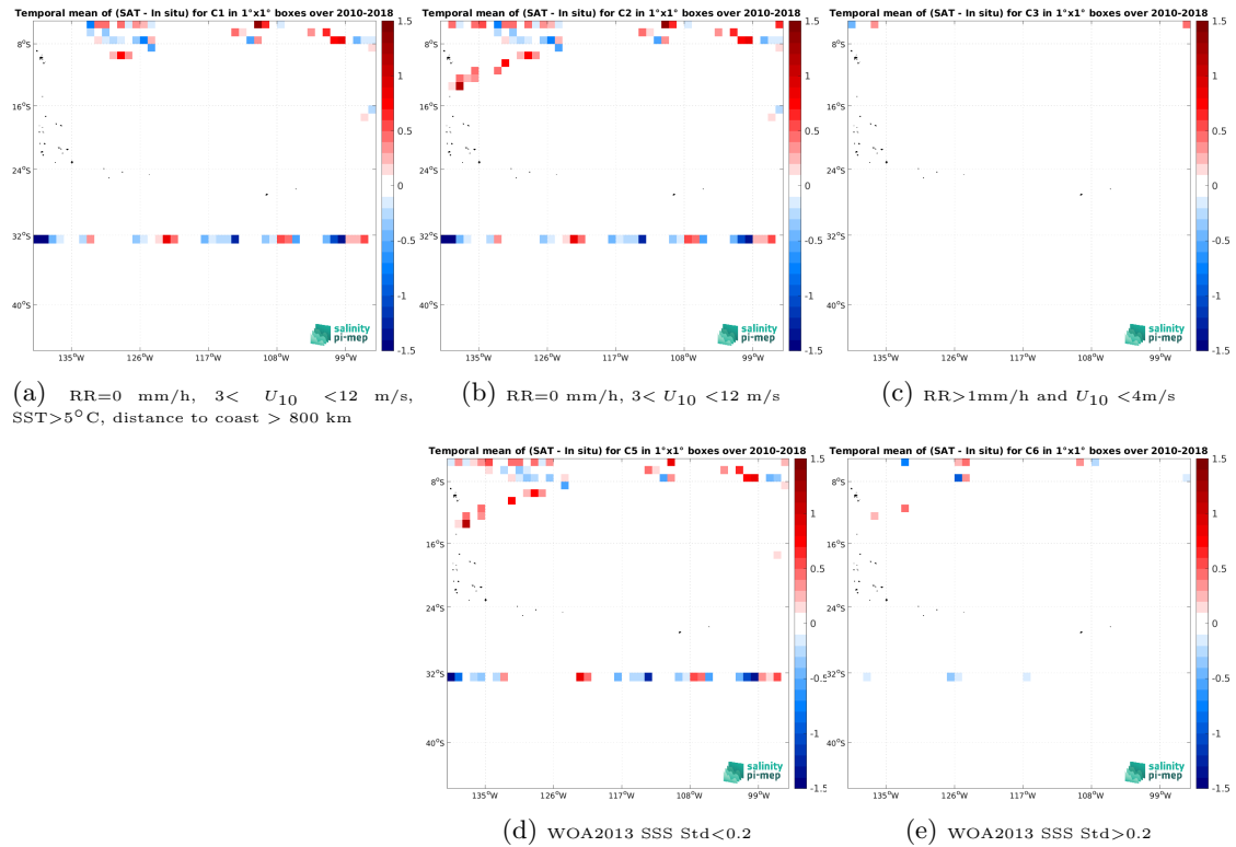
Figure 12: Temporal mean gridded over spatial boxes of size 1^{\circ}\times 1^{\circ} of \Delta\text{SSS} (SMOS SSS L2Q v331 - No FLAG (CMEMS-CATDS-CPDC) - TSG (SAMOS)) for 5 different subdatasets corresponding to:RR=0 mm/h, 3 < U_{10} < 12 m/s, SST >5^{\circ}\text{C} , distance to coast > 800 km (a), RR=0 mm/h, 3 < U_{10} < 12 m/s (b), RR >1\text{mm/h} and U_{10} < 4\text{m/s} (c), WOA2013 SSS Std <0.2 (d), WOA2013 SSS Std >0.2 (e).
