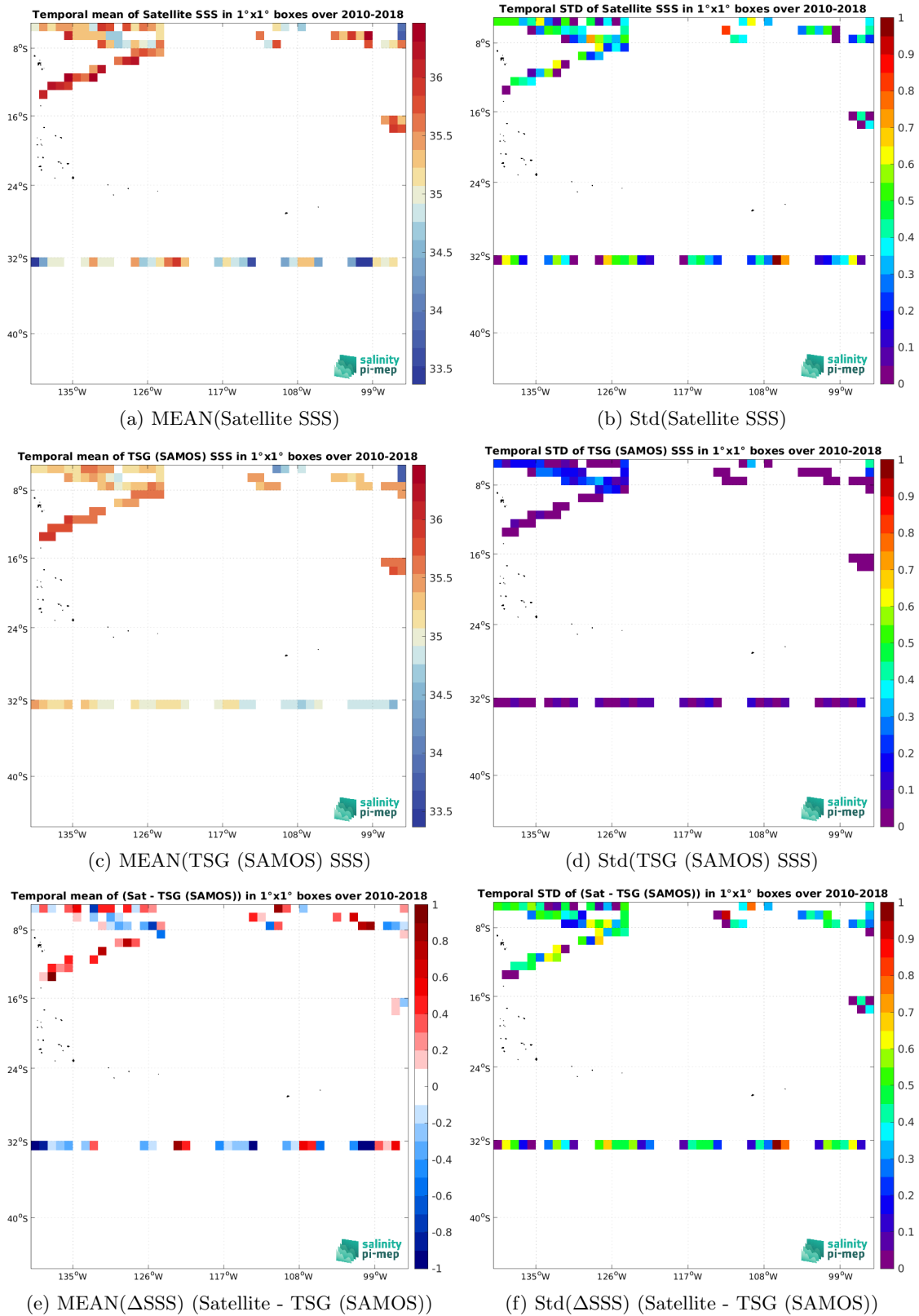
Figure 6: Temporal mean (left) and Std (right) of SSS from SMOS SSS L2Q v331 - No FLAG (CMEMS-CATDS-CPDC) (top), TSG (SAMOS) (middle), and of \Delta SSS (Satellite - TSG (SAMOS)). Only match-up pairs are used to generate these maps.
