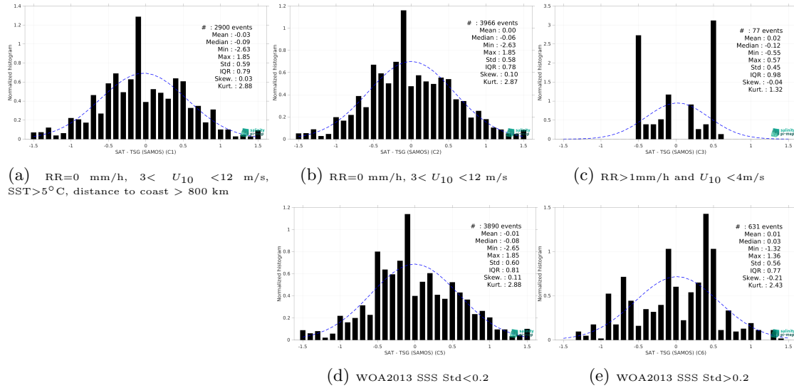
Figure 13: Normalized histogram of \Delta\text{SSS} (SMOS SSS L2Q v331 - No FLAG (CMEMS-CATDS-CPDC) - TSG (SAMOS)) for 5 different subdatasets corresponding to: RR=0 mm/h, 3 < U_{10} < 12 m/s, SST > 5^\circ\text{C} , distance to coast > 800 km (a), RR=0 mm/h, 3 < U_{10} < 12 m/s (b), RR > 1 mm/h and U_{10} < 4 m/s (c), WOA2013 SSS Std < 0.2 (d), WOA2013 SSS Std > 0.2 (e).
