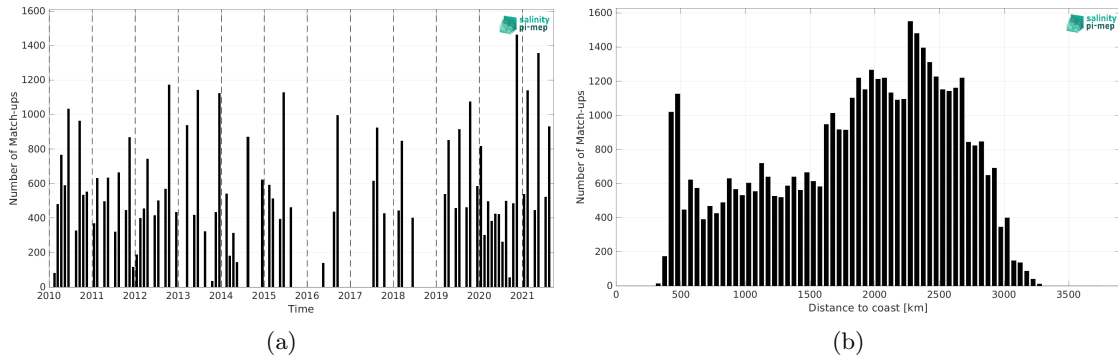
Figure 2: Number of match-ups between TSG (LEGOS-DM) and SMOS SSS L2Q v331 - No FLAG (CMEMS-CATDS-CPDC) SSS as a function of time (a) and as function of the distance to coast (b) over the OTT zone Pi-MEP region and for the full satellite product period.
