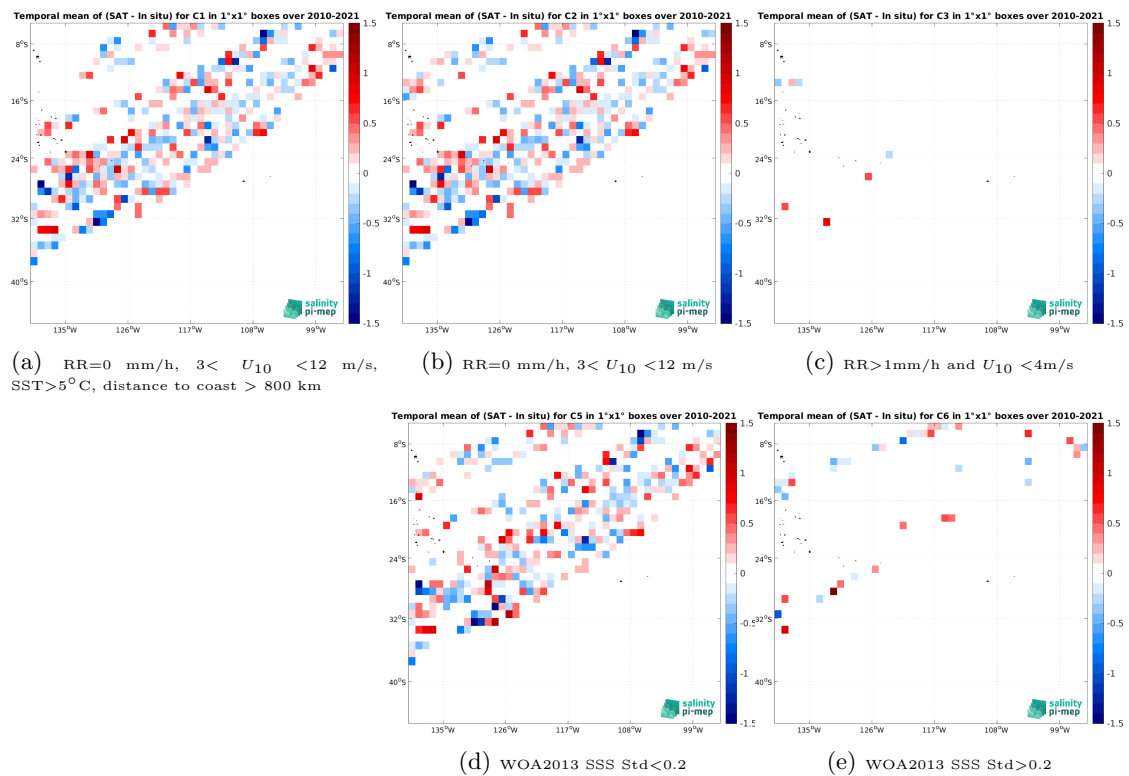
Figure 14: Temporal mean gridded over spatial boxes of size 1^\circ \times 1^\circ of \Delta\text{SSS} (SMOS SSS L2Q v331 - No FLAG (CMEMS-CATDS-CPDC) - TSG (LEGOS-DM)) for 5 different subdatasets corresponding to:RR=0 mm/h, 3 < U_{10} < 12 m/s, SST >5^\circ\text{C} , distance to coast > 800 km (a), RR=0 mm/h, 3 < U_{10} < 12 m/s (b), RR >1 mm/h and U_{10} < 4 m/s (c), WOA2013 SSS Std <0.2 (d), WOA2013 SSS Std >0.2 (e).
