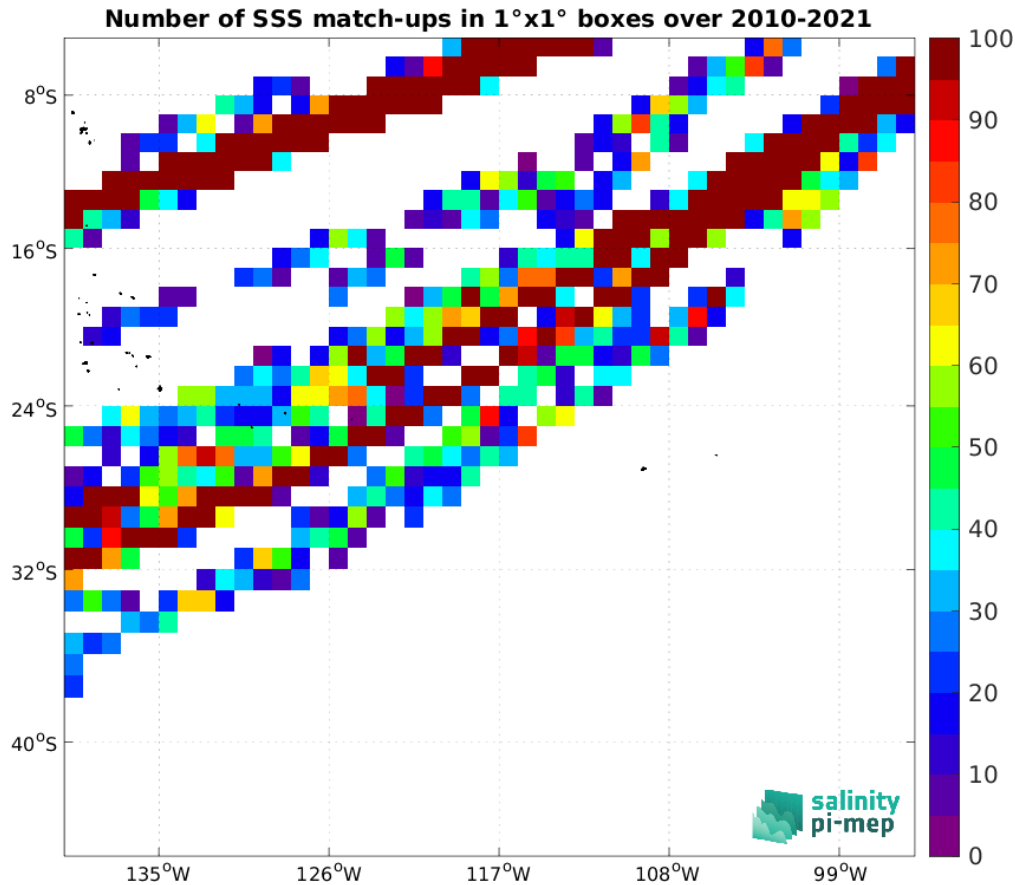
Figure 5: Number of SSS match-ups between TSG (LEGOS-DM) SSS and the SMOS SSS L2Q v331 - No FLAG (CMEMS-CATDS-CPDC) SSS product for the OTT zone Pi-MEP region over 1^\circ \times 1^\circ boxes and for the full satellite product period.
