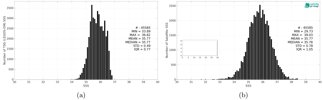
Figure 3: Histograms of SSS from TSG (LEGOS-DM) (a) and SMOS SSS L2Q v331 - No FLAG (CMEMS-CATDS-CPDC) (b) considering all match-up pairs per bins of 0.1 over the OTT zone Pi-MEP region and for the full satellite product period.
