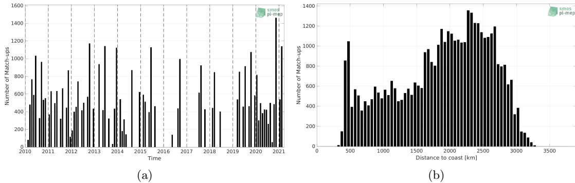
Figure 1: Number of match-ups between TSG (LEGOS-DM) and SMOS SSS L2Q v331 - No FLAG (CMEMS-CATDS-CPDC) SSS as a function of time (a) and as function of the distance to coast (b) over the OTT zone Pi-MEP region and for the full satellite product period.
