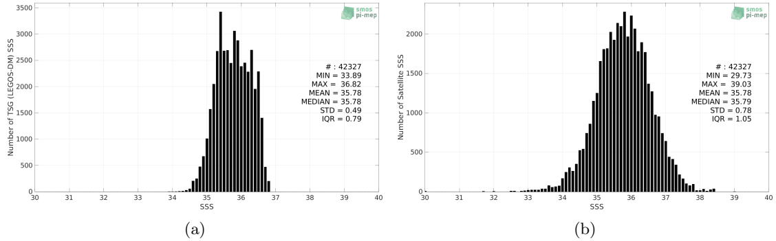
Figure 2: Histograms of SSS from TSG (LEGOS-DM) (a) and SMOS SSS L2Q v331 - No FLAG (CMEMS-CATDS-CPDC) (b) considering all match-up pairs per bins of 0.1 over the OTT zone Pi-MEP region and for the full satellite product period.
