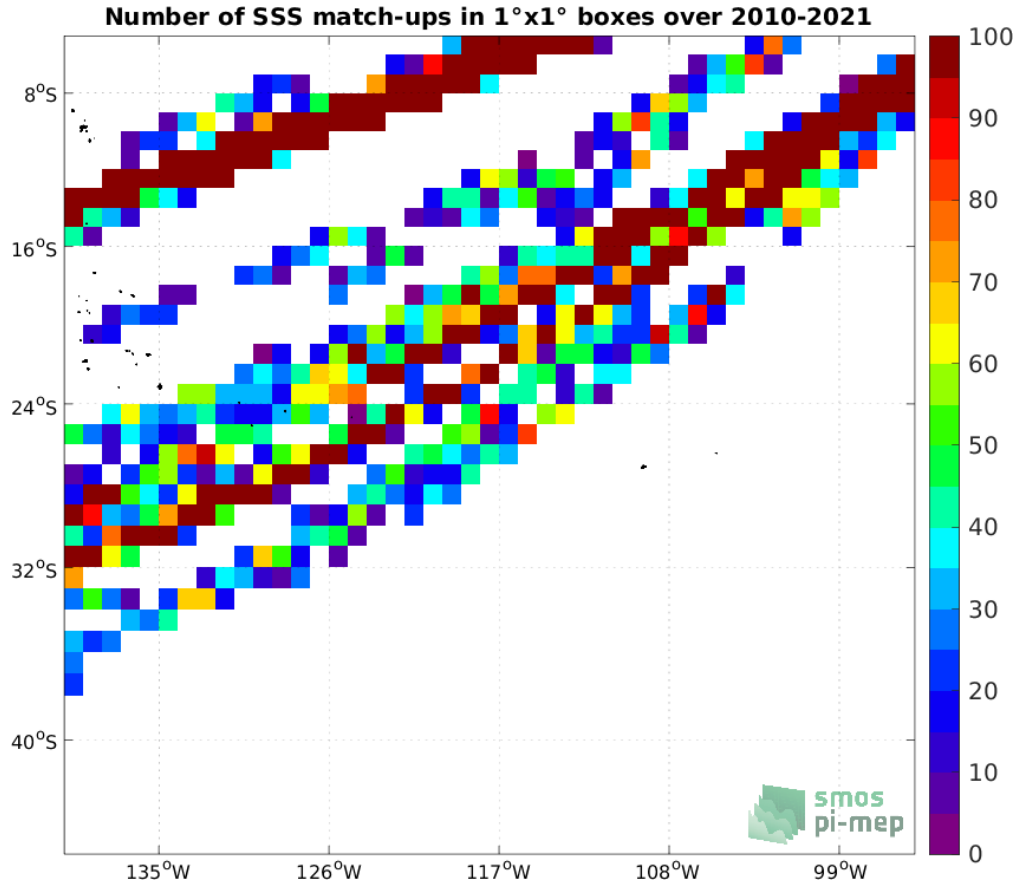
Figure 4: Number of SSS match-ups between TSG (LEGOS-DM) SSS and the SMOS SSS L2Q v331 - No FLAG (CMEMS-CATDS-CPDC) SSS product for the OTT zone Pi-MEP region over 1^\circ \times 1^\circ boxes and for the full satellite product period.
