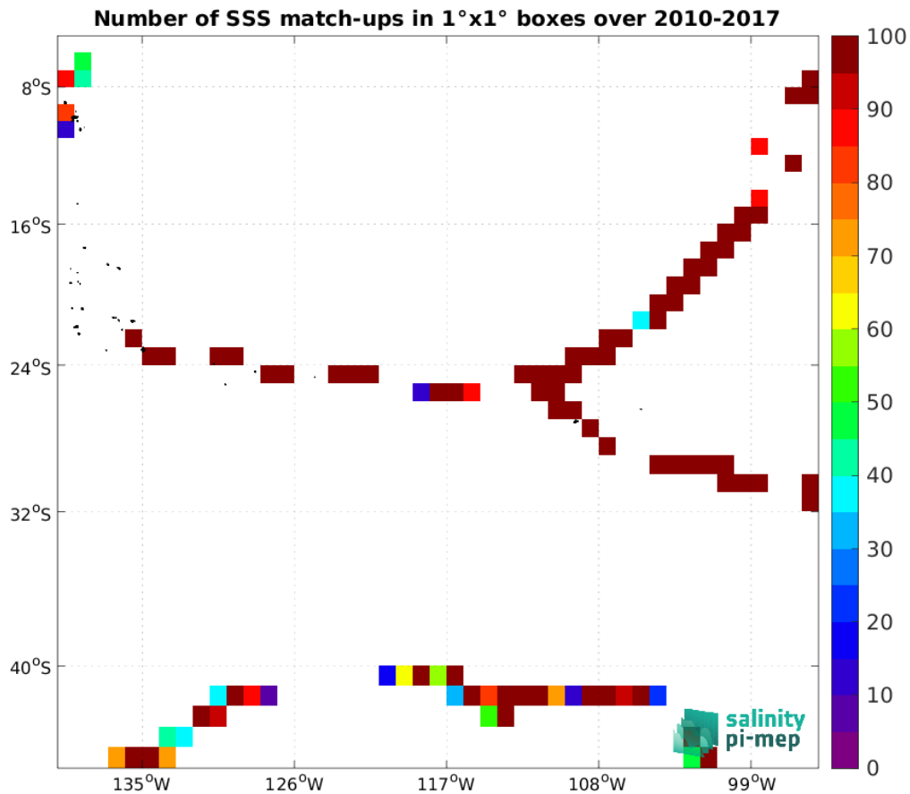
Figure 5: Number of SSS match-ups between TSG (GOSUD-Sailing-ship) SSS and the SMOS SSS L2Q v331 - No FLAG (CMEMS-CATDS-CPDC) SSS product for the OTT zone Pi-MEP region over 1°x1° boxes and for the full satellite product period.
