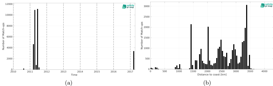
Figure 2: Number of match-ups between TSG (GOSUD-Sailing-ship) and SMOS SSS L2Q v331 - No FLAG (CMEMS-CATDS-CPDC) SSS as a function of time (a) and as function of the distance to coast (b) over the OTT zone Pi-MEP region and for the full satellite product period.
