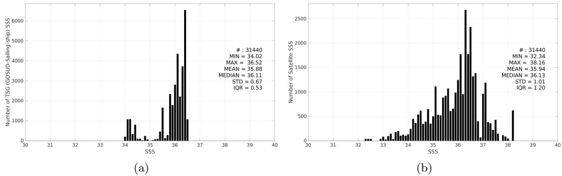
Figure 3: Histograms of SSS from TSG (GOSUD-Sailing-ship) (a) and SMOS SSS L2Q v331 - No FLAG (CMEMS-CATDS-CPDC) (b) considering all match-up pairs per bins of 0.1 over the OTT zone Pi-MEP region and for the full satellite product period.
