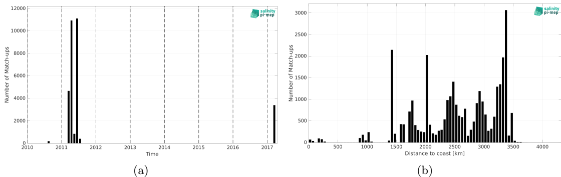
Figure 1: Number of match-ups between TSG (GOSUD-Sailing-ship) and SMOS SSS L2Q v331 - No FLAG (CMEMS-CATDS-CPDC) SSS as a function of time (a) and as function of the distance to coast (b) over the OTT zone Pi-MEP region and for the full satellite product period.
