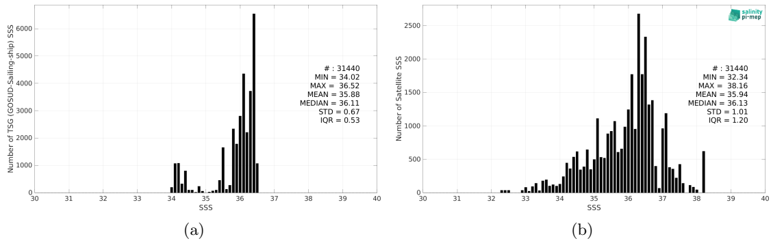
Figure 2: Histograms of SSS from TSG (GOSUD-Sailing-ship) (a) and SMOS SSS L2Q v331 - No FLAG (CMEMS-CATDS-CPDC) (b) considering all match-up pairs per bins of 0.1 over the OTT zone Pi-MEP region and for the full satellite product period.
