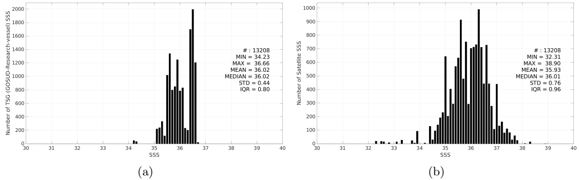
Figure 3: Histograms of SSS from TSG (GOSUD-Research-vessel) (a) and SMOS SSS L2Q v331 - No FLAG (CMEMS-CATDS-CPDC) (b) considering all match-up pairs per bins of 0.1 over the OTT zone Pi-MEP region and for the full satellite product period.
