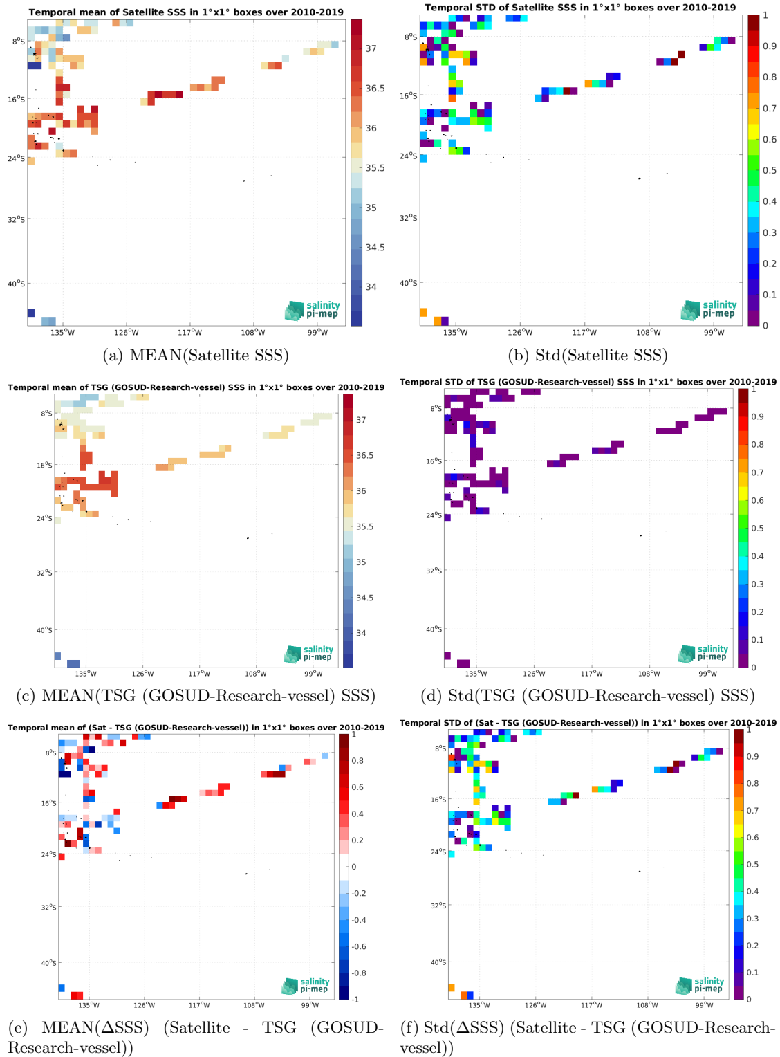
Figure 7: Temporal mean (left) and Std (right) of SSS from SMOS SSS L2Q v331 - No FLAG (CMEMS-CATDS-CPDC) (top), TSG (GOSUD-Research-vessel) (middle), and of \Delta SSS (Satellite - TSG (GOSUD-Research-vessel)). Only match-up pairs are used to generate these maps.
