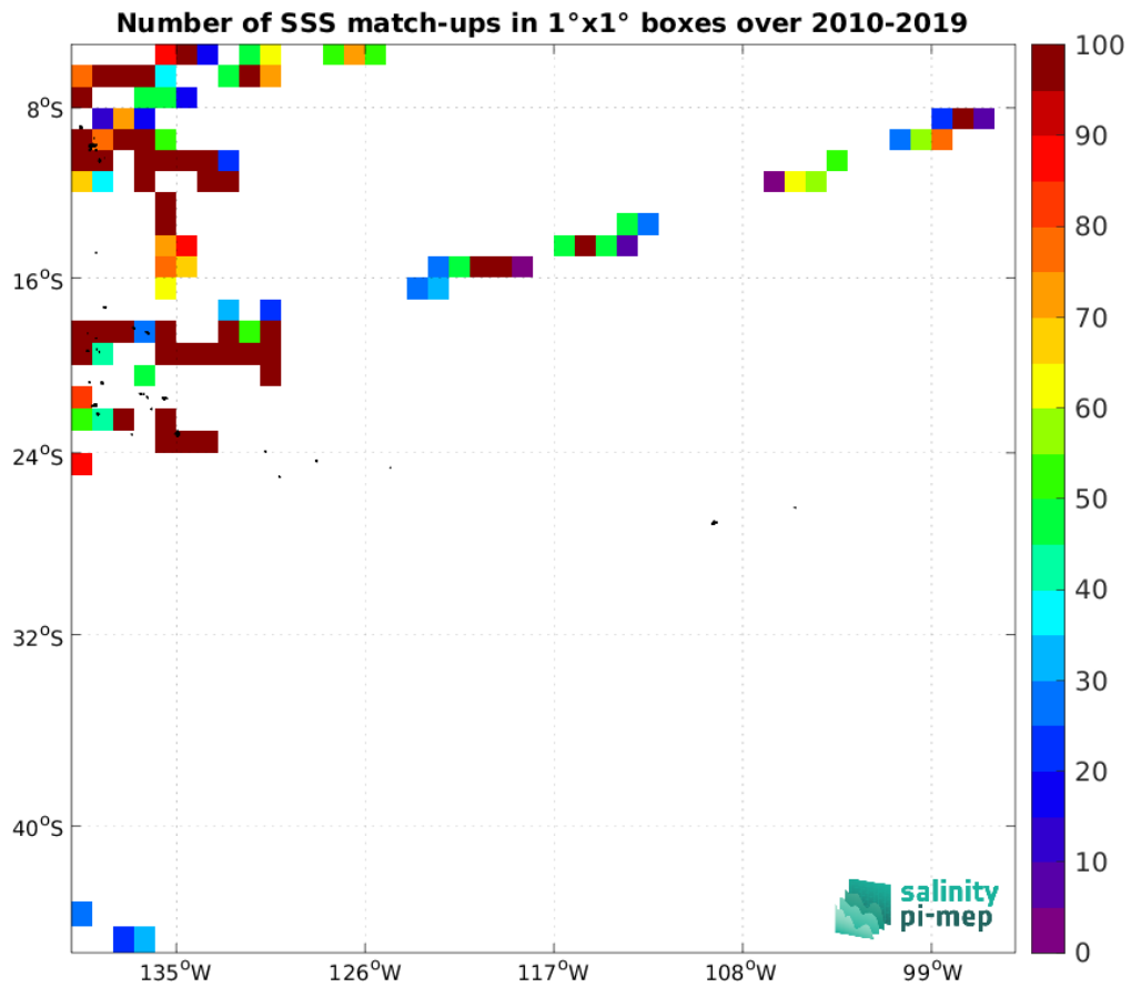
Figure 5: Number of SSS match-ups between TSG (GOSUD-Research-vessel) SSS and the SMOS SSS L2Q v331 - No FLAG (CMEMS-CATDS-CPDC) SSS product for the OTT zone Pi-MEP region over 1^\circ \times 1^\circ boxes and for the full satellite product period.
