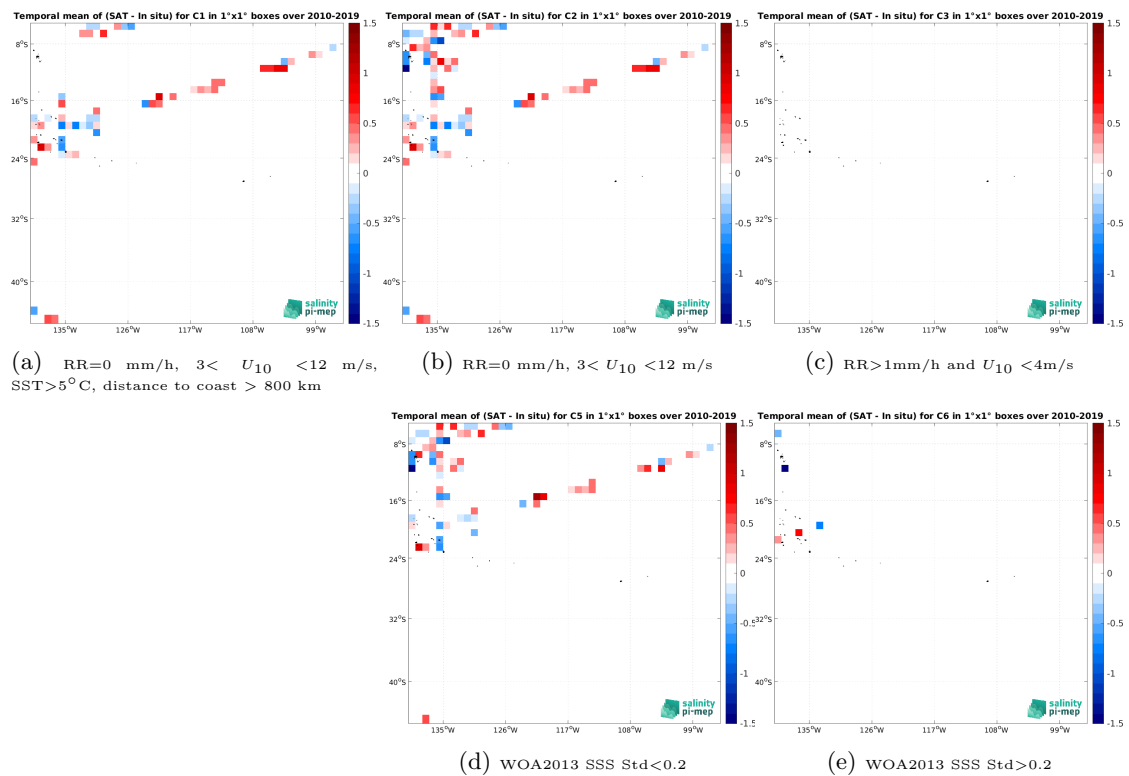
Figure 12: Temporal mean gridded over spatial boxes of size 1^\circ \times 1^\circ of \Delta SSS (SMOS SSS L2Q v331 - No FLAG (CMEMS-CATDS-CPDC) - TSG (GOSUD-Research-vessel)) for 5 different subdatasets corresponding to:RR=0 mm/h, 3 < U_{10} < 12 m/s, SST >5^\circ\text{C} , distance to coast > 800 km (a), RR=0 mm/h, 3 < U_{10} < 12 m/s (b), RR >1 mm/h and U_{10} < 4 m/s (c), WOA2013 SSS Std <0.2 (d), WOA2013 SSS Std >0.2 (e).
