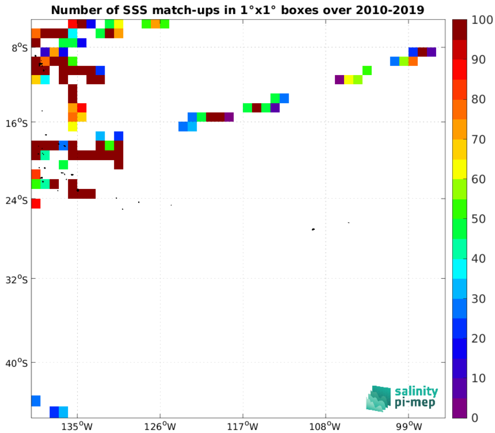
Figure 4: Number of SSS match-ups between TSG (GOSUD-Research-vessel) SSS and the SMOS SSS L2Q v331 - No FLAG (CMEMS-CATDS-CPDC) SSS product for the OTT zone Pi-MEP region over 1^\circ \times 1^\circ boxes and for the full satellite product period.
