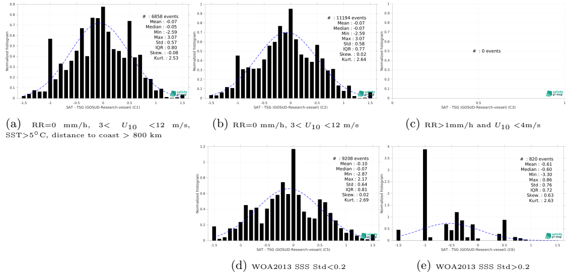
Figure 13: Normalized histogram of \Delta\text{SSS} (SMOS SSS L2Q v331 - No FLAG (CMEMS-CATDS-CPDC) - TSG (GOSUD-Research-vessel)) for 5 different subdatasets corresponding to: RR=0 mm/h, 3 < U_{10} < 12 m/s, SST > 5^\circ\text{C} , distance to coast > 800 km (a), RR=0 mm/h, 3 < U_{10} < 12 m/s (b), RR > 1 mm/h and U_{10} < 4 m/s (c), WOA2013 SSS Std < 0.2 (d), WOA2013 SSS Std > 0.2 (e).
