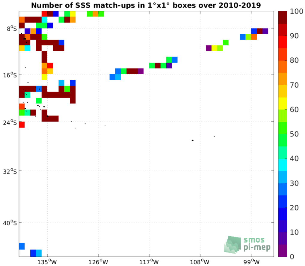
Figure 4: Number of SSS match-ups between TSG (GOSUD-Research-vessel) SSS and the SMOS SSS L2Q v331 - No FLAG (CMEMS-CATDS-CPDC) SSS product for the OTT zone Pi-MEP region over 1°x1° boxes and for the full satellite product period.
