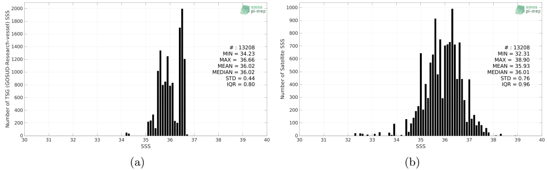
Figure 2: Histograms of SSS from TSG (GOSUD-Research-vessel) (a) and SMOS SSS L2Q v331 - No FLAG (CMEMS-CATDS-CPDC) (b) considering all match-up pairs per bins of 0.1 over the OTT zone Pi-MEP region and for the full satellite product period.
