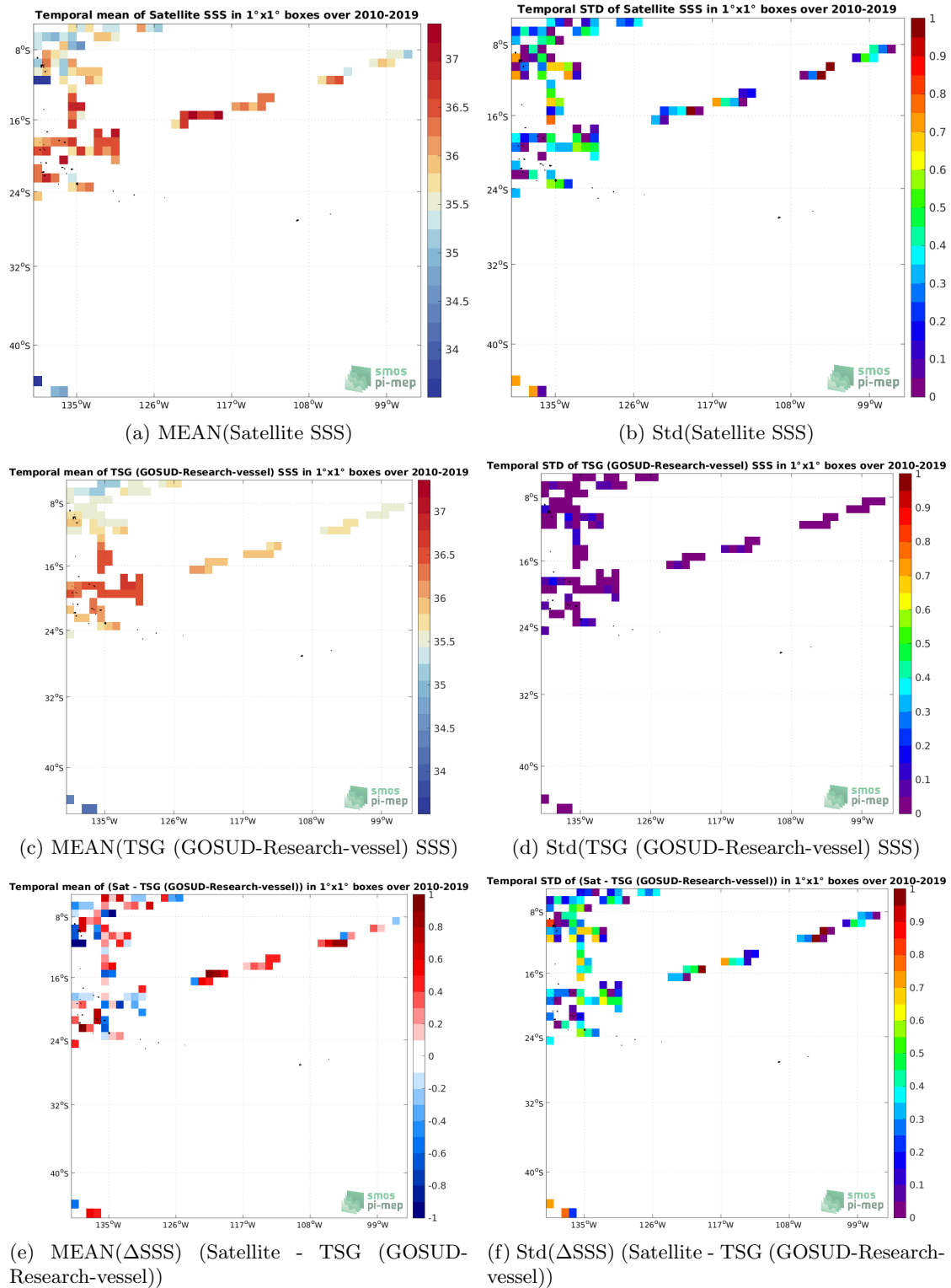
Figure 6: Temporal mean (left) and Std (right) of SSS from SMOS SSS L2Q v331 - No FLAG (CMEMS-CATDS-CPDC) (top), TSG (GOSUD-Research-vessel) (middle), and of \Delta SSS (Satellite - TSG (GOSUD-Research-vessel)). Only match-up pairs are used to generate these maps.
