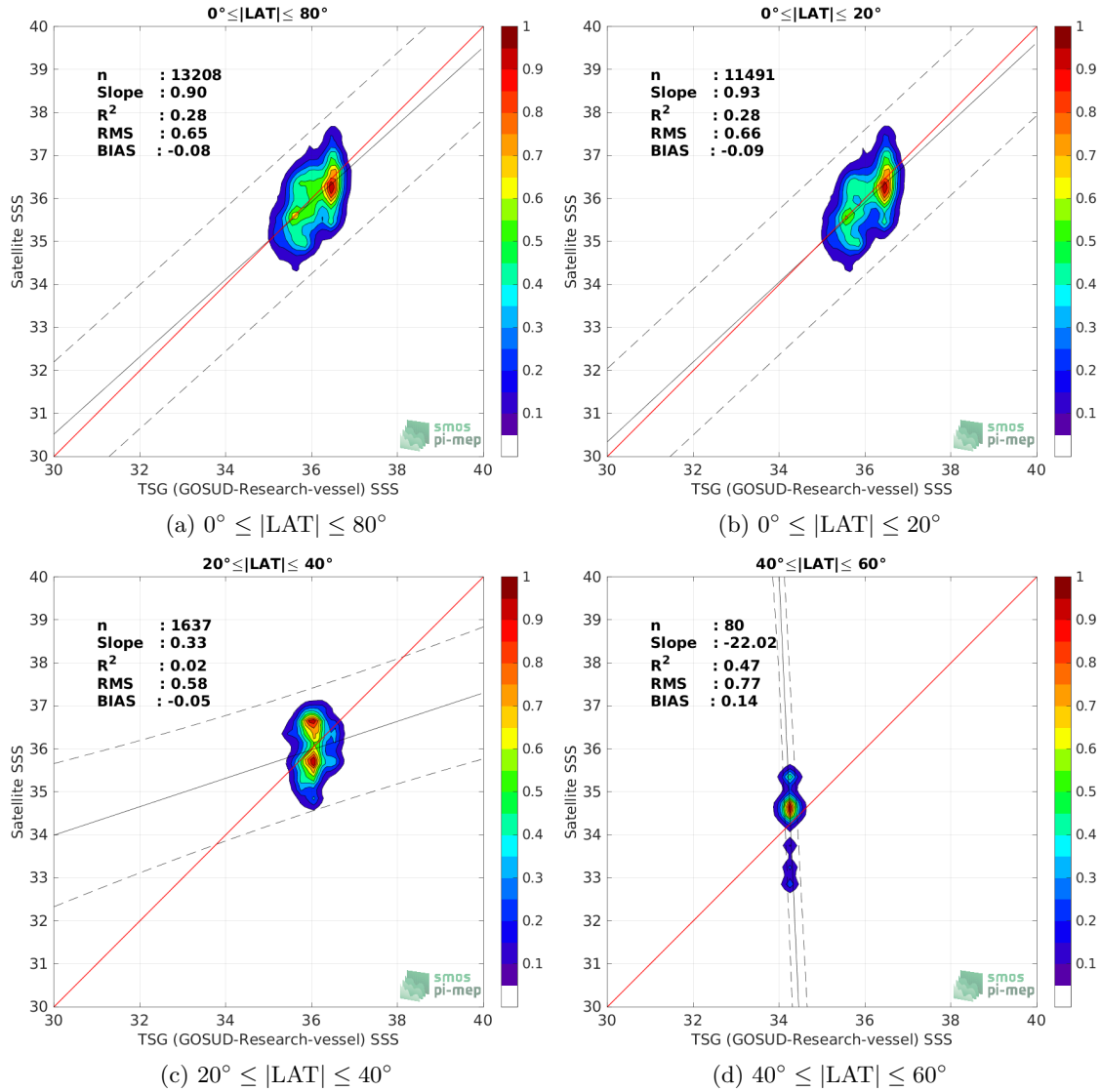
Figure 9: Contour maps of the concentration of SMOS SSS L2Q v331 - No FLAG (CMEMS-CATDS-CPDC) SSS ( y -axis) versus TSG (GOSUD-Research-vessel) SSS ( x -axis) at match-up pairs for different latitude bands. For each plot, the red line shows x=y . The black thin and dashed lines indicate a linear fit through the data cloud and the \pm 95\% confidence levels, respectively. The number match-up pairs n , the slope and R^2 coefficient of the linear fit, the root mean square (RMS) and the mean bias between satellite and in situ data are indicated for each latitude band in each plots.
