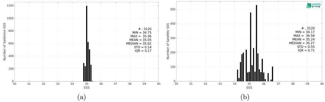
Figure 2: Histograms of SSS from Saildrone (a) and SMOS SSS L2Q v331 - No FLAG (CMEMS-CATDS-CPDC) (b) considering all match-up pairs per bins of 0.1 over the OTT zone Pi-MEP region and for the full satellite product period.
