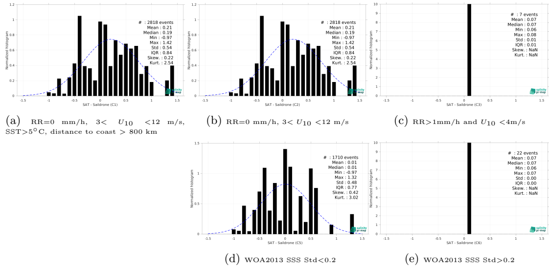
Figure 13: Normalized histogram of \Delta SSS (SMOS SSS L2Q v331 - No FLAG (CMEMS-CATDS-CPDC) - Sairdrone) for 5 different subdatasets corresponding to: RR=0 mm/h, 3 < U_{10} < 12 m/s, SST > 5°C, distance to coast > 800 km (a), RR=0 mm/h, 3 < U_{10} < 12 m/s (b), RR > 1mm/h and U_{10} < 4 m/s (c), WOA2013 SSS Std < 0.2 (d), WOA2013 SSS Std > 0.2 (e).
