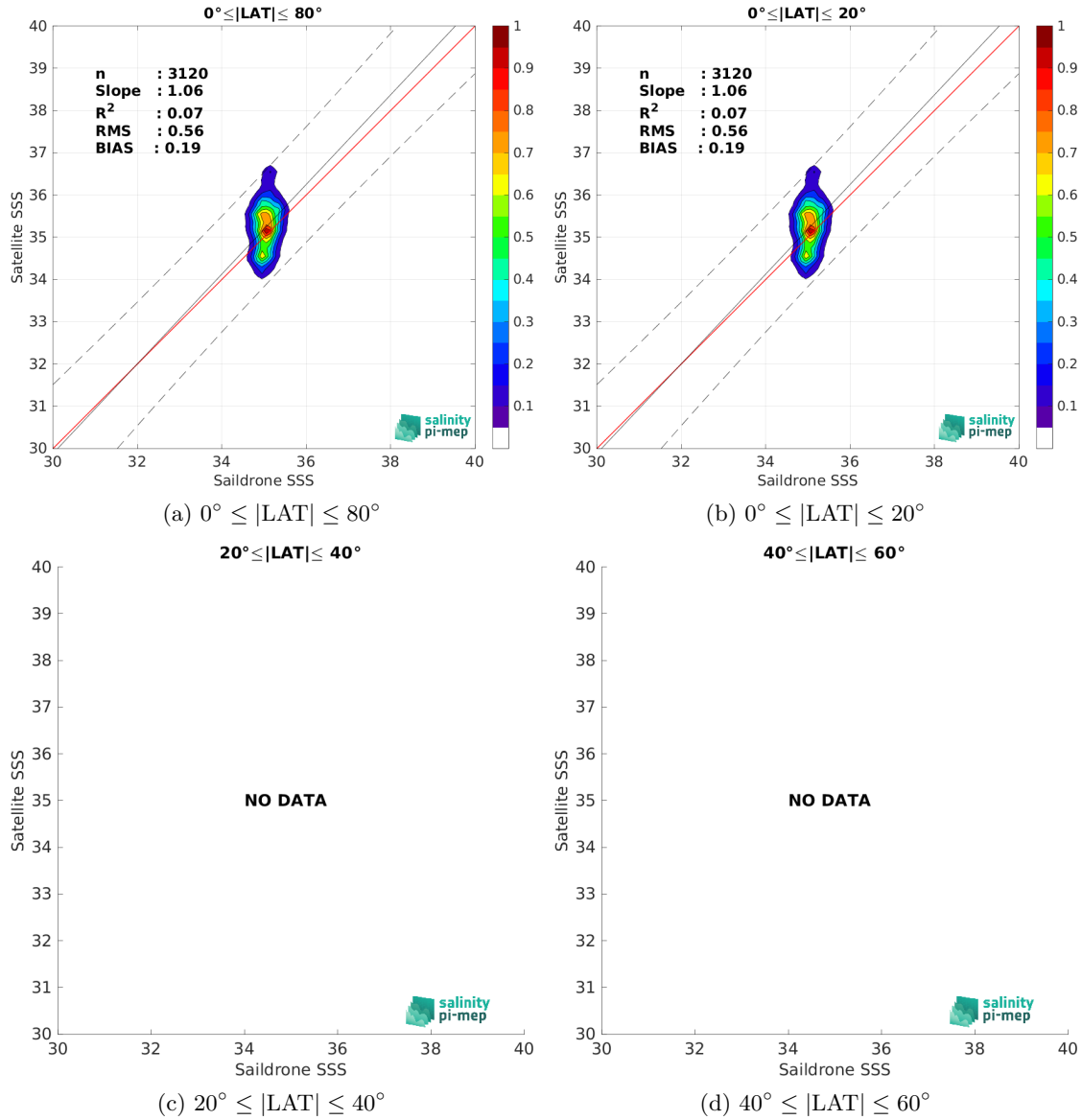
Figure 9: Contour maps of the concentration of SMOS SSS L2Q v331 - No FLAG (CMEMS-CATDS-CPDC) SSS (y-axis) versus Saildrone SSS (x-axis) at match-up pairs for different latitude bands. For each plot, the red line shows x=y . The black thin and dashed lines indicate a linear fit through the data cloud and the \pm 95\% confidence levels, respectively. The number match-up pairs n , the slope and R^2 coefficient of the linear fit, the root mean square (RMS) and the mean bias between satellite and in situ data are indicated for each latitude band in each plots.
