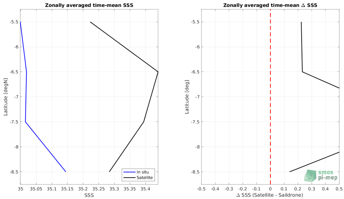
Figure 8: Left panel: Zonal mean SSS from SMOS SSS L2Q v331 - No FLAG (CMEMS-CATDS-CPDC) satellite product (black) and from Saïdrone (blue). Right panel: Zonal mean of \Delta SSS (Satellite - Saïdrone) for all the collected Pi-MEP match-up pairs estimated over the full satellite product period.
