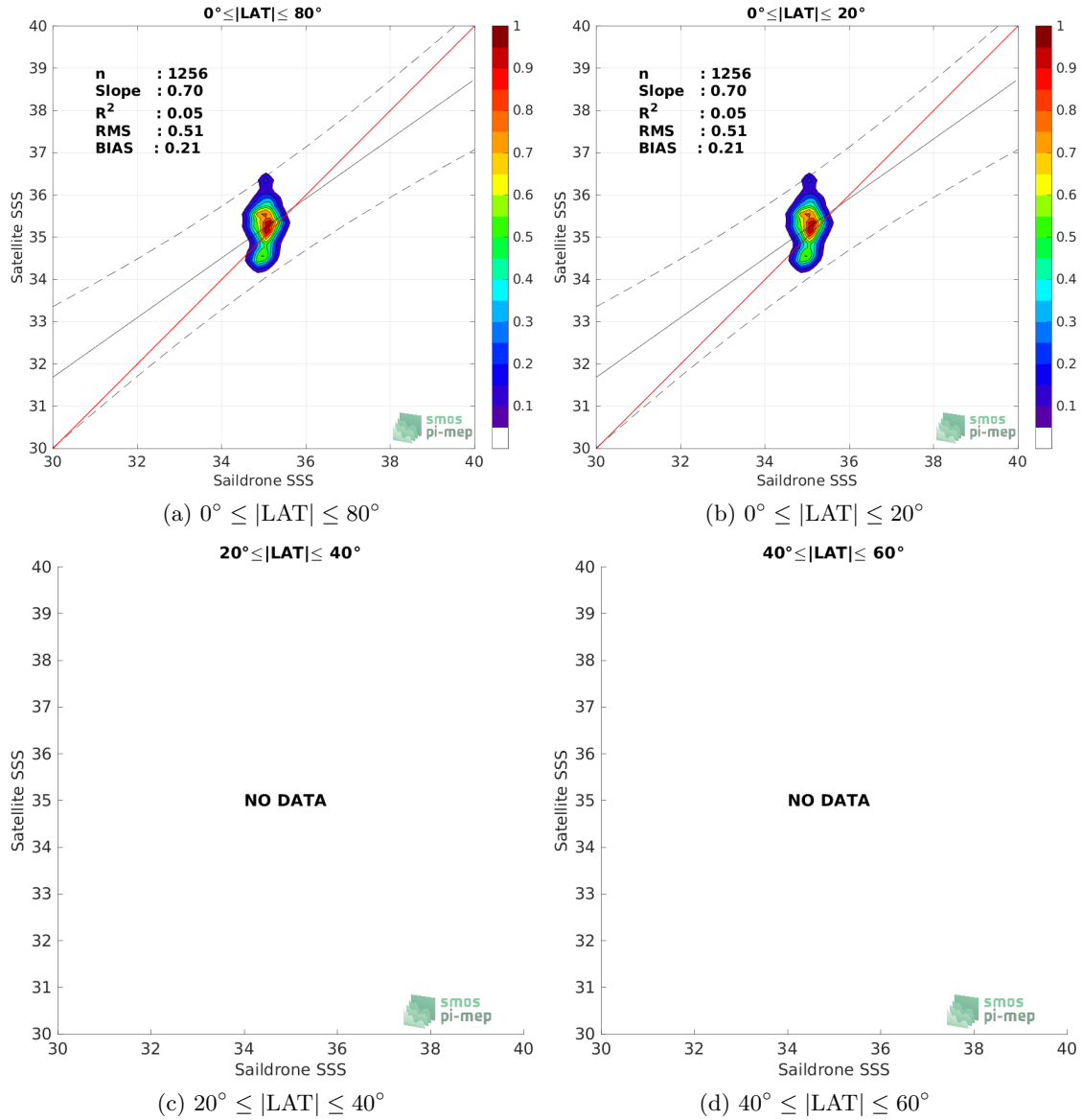
Figure 9: Contour maps of the concentration of SMOS SSS L2Q v331 - No FLAG (CMEMS-CATDS-CPDC) SSS (y-axis) versus Saieldrone SSS (x-axis) at match-up pairs for different latitude bands. For each plot, the red line shows x=y . The black thin and dashed lines indicate a linear fit through the data cloud and the \pm 95\% confidence levels, respectively. The number match-up pairs n , the slope and R^2 coefficient of the linear fit, the root mean square (RMS) and the mean bias between satellite and in situ data are indicated for each latitude band in each plots.
