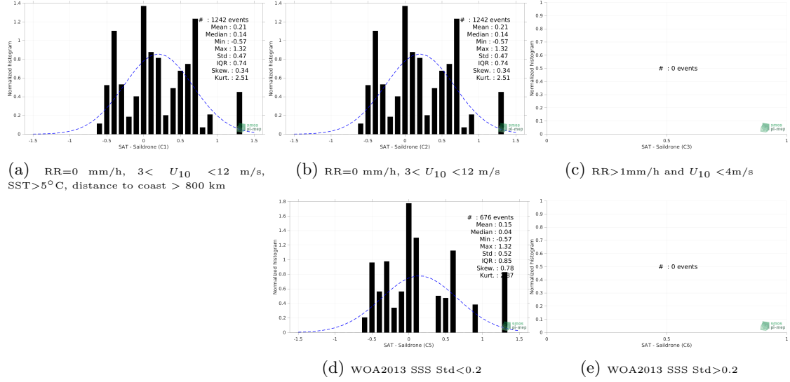
Figure 13: Normalized histogram of \Delta SSS (SMOS SSS L2Q v331 - No FLAG (CMEMS-CATDS-CPDC) - Saildrone) for 5 different subdatasets corresponding to: RR=0 mm/h, 3 < U_{10} < 12 m/s, SST>5°C, distance to coast > 800 km (a), RR=0 mm/h, 3 < U_{10} < 12 m/s (b), RR>1mm/h and U_{10} < 4 m/s (c), WOA2013 SSS Std<0.2 (d), WOA2013 SSS Std>0.2 (e).
