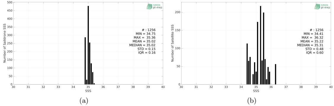
Figure 2: Histograms of SSS from Saifdrone (a) and SMOS SSS L2Q v331 - No FLAG (CMEMS-CATDS-CPDC) (b) considering all match-up pairs per bins of 0.1 over the OTT zone Pi-MEP region and for the full satellite product period.
