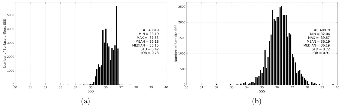
Figure 3: Histograms of SSS from Surface drifters (a) and SMOS SSS L2Q v331 - No FLAG (CMEMS-CATDS-CPDC) (b) considering all match-up pairs per bins of 0.1 over the OTT zone Pi-MEP region and for the full satellite product period.
