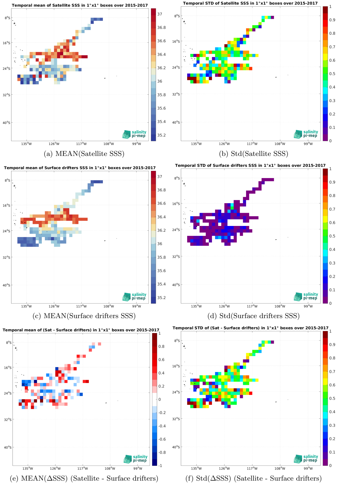
Figure 6: Temporal mean (left) and Std (right) of SSS from SMOS SSS L2Q v331 - No FLAG (CMEMS-CATDS-CPDC) (top), Surface drifters (middle), and of \Delta SSS (Satellite - Surface drifters). Only match-up pairs are used to generate these maps.
