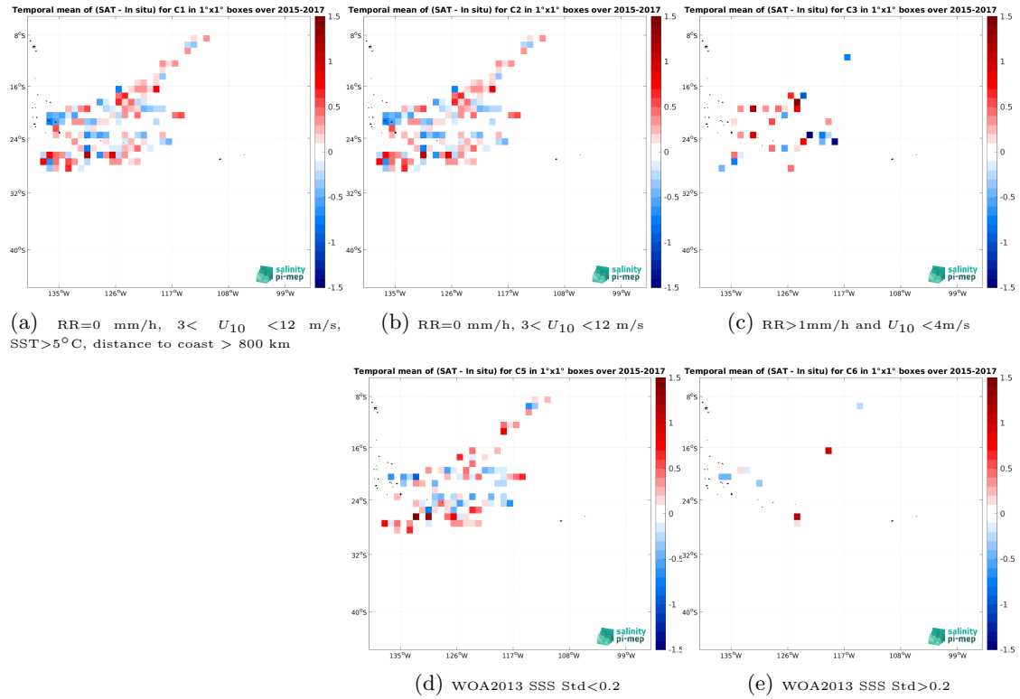
Figure 13: Temporal mean gridded over spatial boxes of size 1^\circ \times 1^\circ of \Delta SSS (SMOS SSS L2Q v331 - No FLAG (CMEMS-CATDS-CPDC) - Surface drifters) for 5 different subdatasets corresponding to:RR=0 mm/h, 3 < U_{10} < 12 m/s, SST >5^\circ C, distance to coast > 800 km (a), RR=0 mm/h, 3 < U_{10} < 12 m/s (b), RR >1 mm/h and U_{10} < 4 m/s (c), WOA2013 SSS Std <0.2 (d), WOA2013 SSS Std >0.2 (e).
