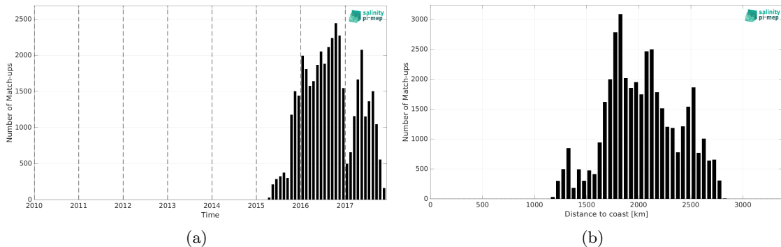
Figure 2: Number of match-ups between Surface drifters and SMOS SSS L2Q v331 - No FLAG (CMEMS-CATDS-CPDC) SSS as a function of time (a) and as function of the distance to coast (b) over the OTT zone Pi-MEP region and for the full satellite product period.
