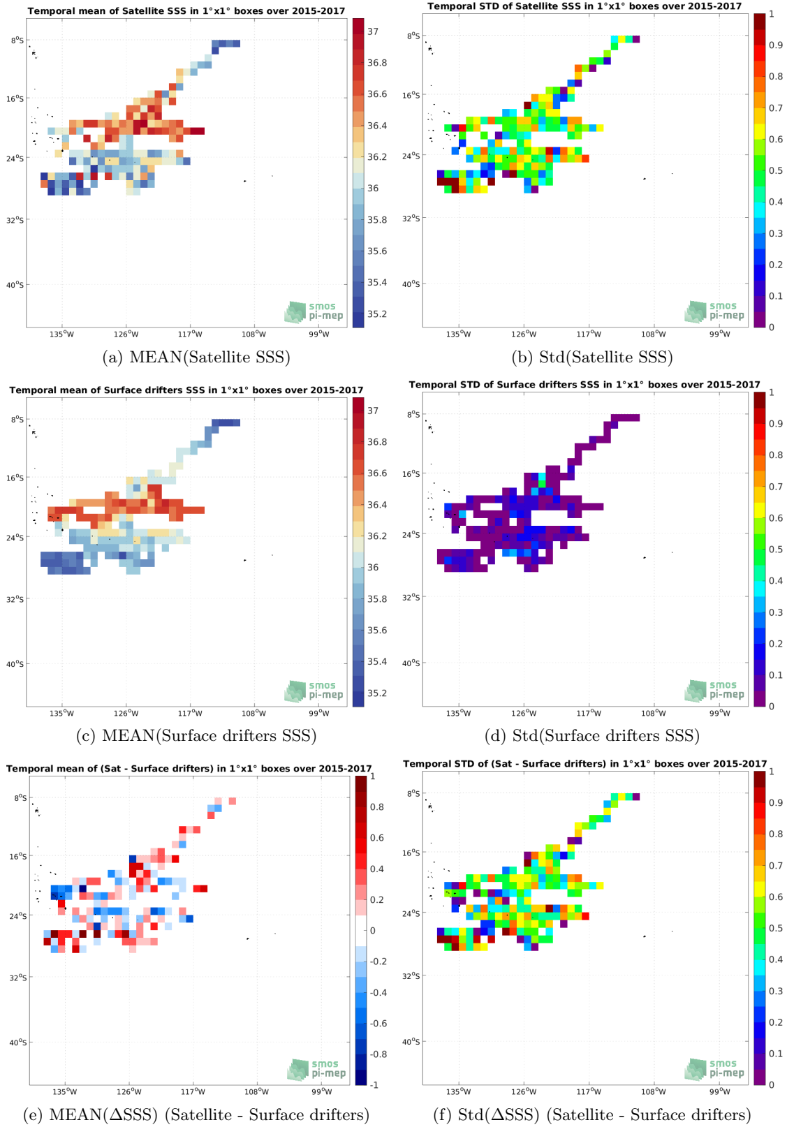
Figure 5: Temporal mean (left) and Std (right) of SSS from SMOS SSS L2Q v331 - No FLAG (CMEMS-CATDS-CPDC) (top), Surface drifters (middle), and of \Delta SSS (Satellite - Surface drifters). Only match-up pairs are used to generate these maps.
