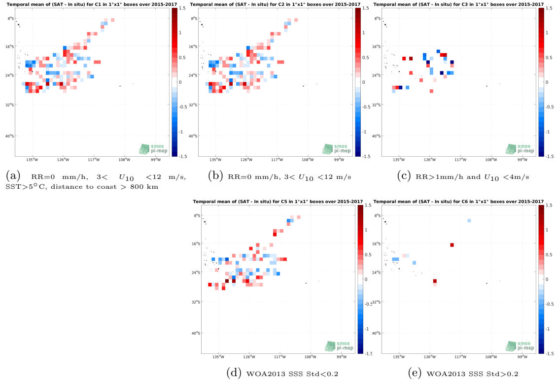
Figure 11: Temporal mean gridded over spatial boxes of size 1^{\circ}\times 1^{\circ} of \Delta\text{SSS} (SMOS SSS L2Q v331 - No FLAG (CMEMS-CATDS-CPDC) - Surface drifters) for 5 different subdatasets corresponding to:RR=0 mm/h, 3 < U_{10} < 12 m/s, SST >5^{\circ}\text{C} , distance to coast > 800 km (a), RR=0 mm/h, 3 < U_{10} < 12 m/s (b), RR >1 mm/h and U_{10} < 4 m/s (c), WOA2013 SSS Std <0.2 (d), WOA2013 SSS Std >0.2 (e).
