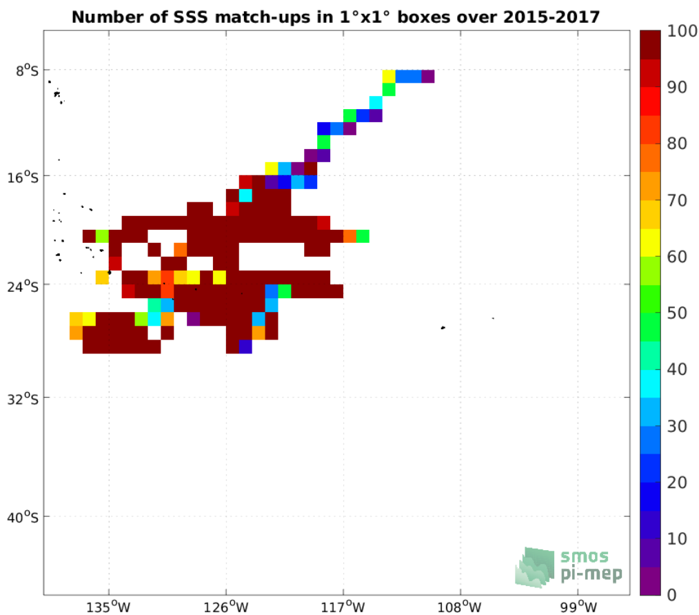
Figure 3: Number of SSS match-ups between Surface drifters SSS and the SMOS SSS L2Q v331 - No FLAG (CMEMS-CATDS-CPDC) SSS product for the OTT zone Pi-MEP region over 1^\circ \times 1^\circ boxes and for the full satellite product period.
