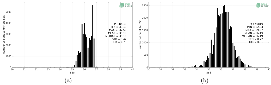
Figure 2: Histograms of SSS from Surface drifters (a) and SMOS SSS L2Q v331 - No FLAG (CMEMS-CATDS-CPDC) (b) considering all match-up pairs per bins of 0.1 over the OTT zone Pi-MEP region and for the full satellite product period.
