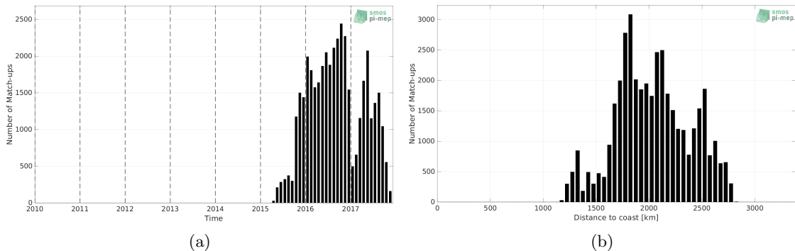
Figure 1: Number of match-ups between Surface drifters and SMOS SSS L2Q v331 - No FLAG (CMEMS-CATDS-CPDC) SSS as a function of time (a) and as function of the distance to coast (b) over the OTT zone Pi-MEP region and for the full satellite product period.
