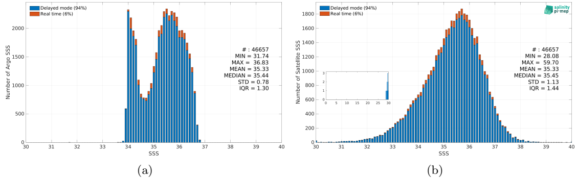
Figure 3: Histograms of SSS from Argo (a) and SMOS SSS L2Q v331 - No FLAG (CMEMS-CATDS-CPDC) (b) considering all match-up pairs per bins of 0.1 over the OTT zone Pi-MEP region and for the full satellite product period.
