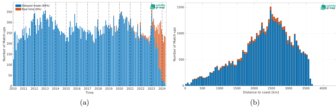
Figure 2: Number of match-ups between Argo and SMOS SSS L2Q v331 - No FLAG (CMEMS-CATDS-CPDC) SSS as a function of time (a) and as function of the distance to coast (b) over the OTT zone Pi-MEP region and for the full satellite product period.
