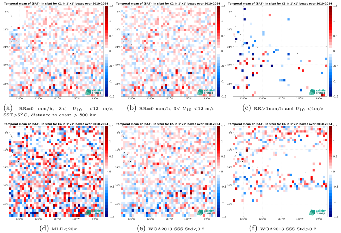
Figure 14: Temporal mean gridded over spatial boxes of size 1^\circ \times 1^\circ of \Delta SSS (SMOS SSS L2Q v331 - No FLAG (CMEMS-CATDS-CPDC) - Argo) for 6 different subdatasets corresponding to:RR=0 mm/h, 3 < U_{10} < 12 m/s, SST >5^\circ C, distance to coast > 800 km (a), RR=0 mm/h, 3 < U_{10} < 12 m/s (b), RR >1 mm/h and U_{10} < 4 m/s (c),MLD <20 m (d),WOA2013 SSS Std <0.2 (e),WOA2013 SSS Std >0.2 (f).
