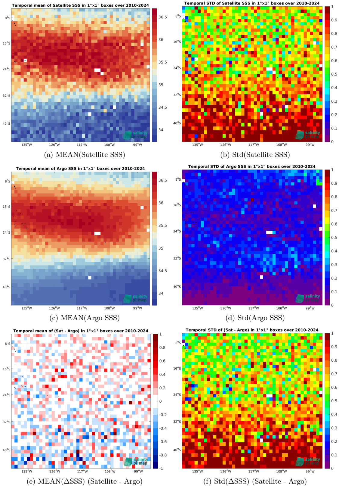
Figure 7: Temporal mean (left) and Std (right) of SSS from SMOS SSS L2Q v331 - No FLAG (CMEMS-CATDS-CPDC) (top), Argo (middle), and of \Delta SSS (Satellite - Argo). Only match-up pairs are used to generate these maps.
