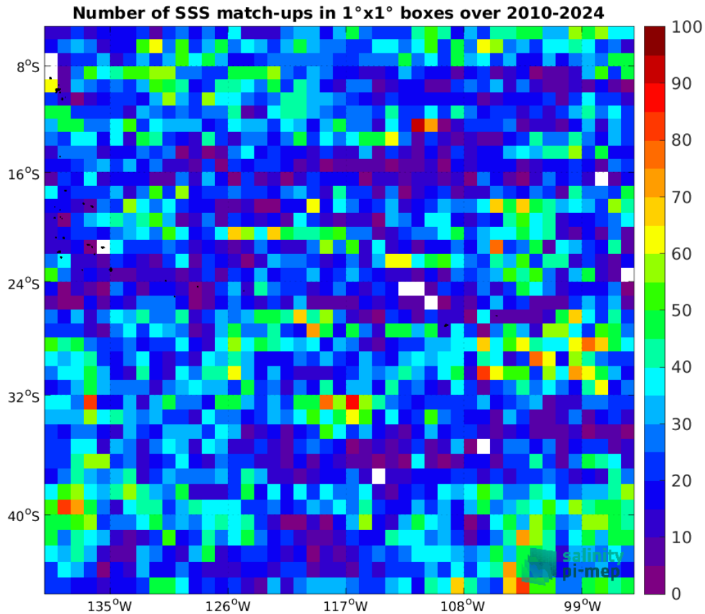
Figure 5: Number of SSS match-ups between Argo SSS and the SMOS SSS L2Q v331 - No FLAG (CMEMS-CATDS-CPDC) SSS product for the OTT zone Pi-MEP region over 1^\circ \times 1^\circ boxes and for the full satellite product period.
