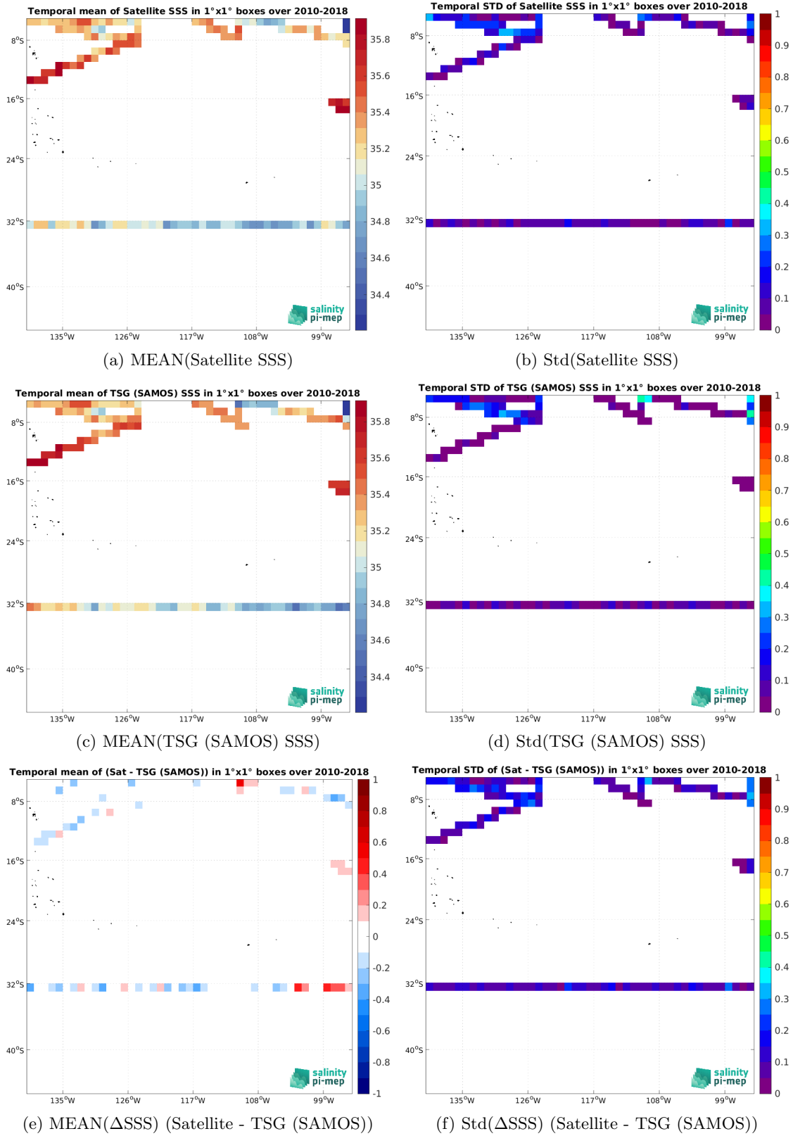
Figure 7: Temporal mean (left) and Std (right) of SSS from SMOS SSS L3 v9 - 9 Days (CATDS-CEC-LOCEAN) (top), TSG (SAMOS) (middle), and of \Delta SSS (Satellite - TSG (SAMOS)). Only match-up pairs are used to generate these maps.
