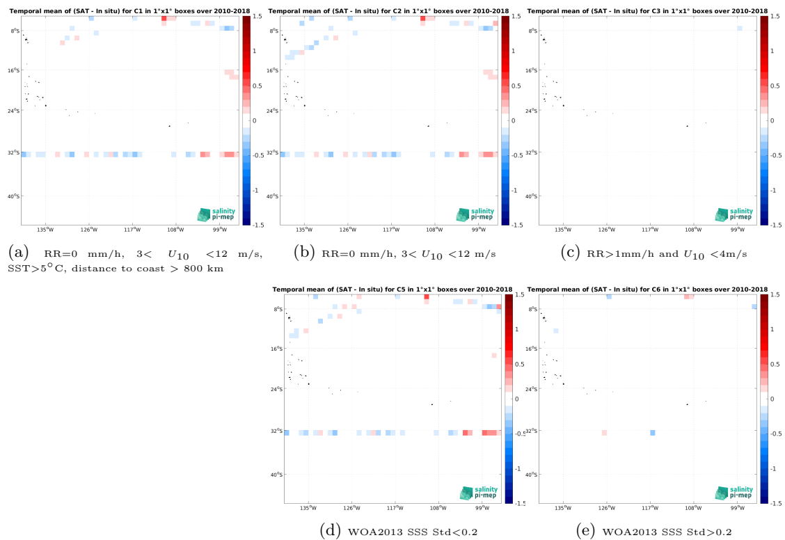
Figure 14: Temporal mean gridded over spatial boxes of size 1^\circ \times 1^\circ of \Delta SSS (SMOS SSS L3 v9 - 9 Days (CATDS-CEC-LOCEAN) - TSG (SAMOS)) for 5 different subdatasets corresponding to: RR=0 mm/h, 3 < U_{10} < 12 m/s, SST > 5^\circ C , distance to coast > 800 km (a), RR=0 mm/h, 3 < U_{10} < 12 m/s (b), RR > 1 mm/h and U_{10} < 4 m/s (c), WOA2013 SSS Std < 0.2 (d), WOA2013 SSS Std > 0.2 (e).
