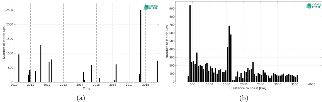
Figure 2: Number of match-ups between TSG (SAMOS) and SMOS SSS L3 v9 - 9 Days (CATDS-CEC-LOCEAN) SSS as a function of time (a) and as function of the distance to coast (b) over the OTT zone Pi-MEP region and for the full satellite product period.
