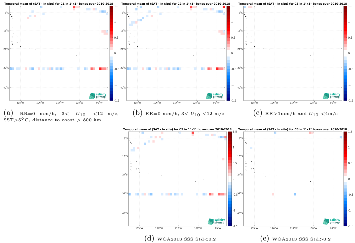
Figure 12: Temporal mean gridded over spatial boxes of size 1^{\circ}\times 1^{\circ} of \Delta\text{SSS} (SMOS SSS L3 v9 - 9 Days (CATDS-CEC-LOCEAN) - TSG (SAMOS)) for 5 different subdatasets corresponding to:RR=0 mm/h, 3 < U_{10} < 12 m/s, SST >5^{\circ}\text{C} , distance to coast > 800 km (a), RR=0 mm/h, 3 < U_{10} < 12 m/s (b), RR >1 mm/h and U_{10} < 4 m/s (c), WOA2013 SSS Std <0.2 (d), WOA2013 SSS Std >0.2 (e).
