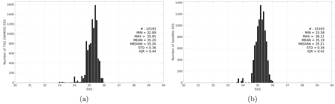
Figure 2: Histograms of SSS from TSG (SAMOS) (a) and SMOS SSS L3 v9 - 9 Days (CATDS-CEC-LOCEAN) (b) considering all match-up pairs per bins of 0.1 over the OTT zone Pi-MEP region and for the full satellite product period.
