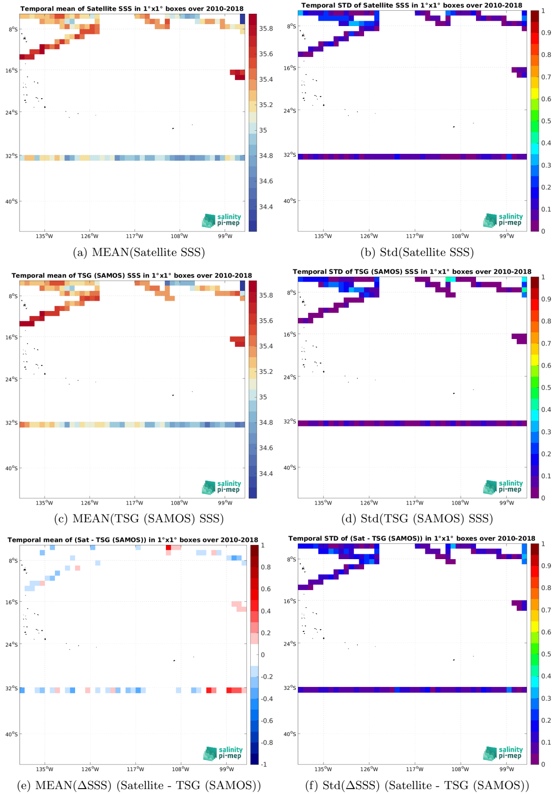
Figure 6: Temporal mean (left) and Std (right) of SSS from SMOS SSS L3 v9 - 9 Days (CATDS-CEC-LOCEAN) (top), TSG (SAMOS) (middle), and of \Delta SSS (Satellite - TSG (SAMOS)). Only match-up pairs are used to generate these maps.
