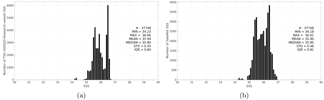
Figure 3: Histograms of SSS from TSG (GOSUD-Research-vessel) (a) and SMOS SSS L3 v9 - 9 Days (CATDS-CEC-LOCEAN) (b) considering all match-up pairs per bins of 0.1 over the OTT zone Pi-MEP region and for the full satellite product period.
