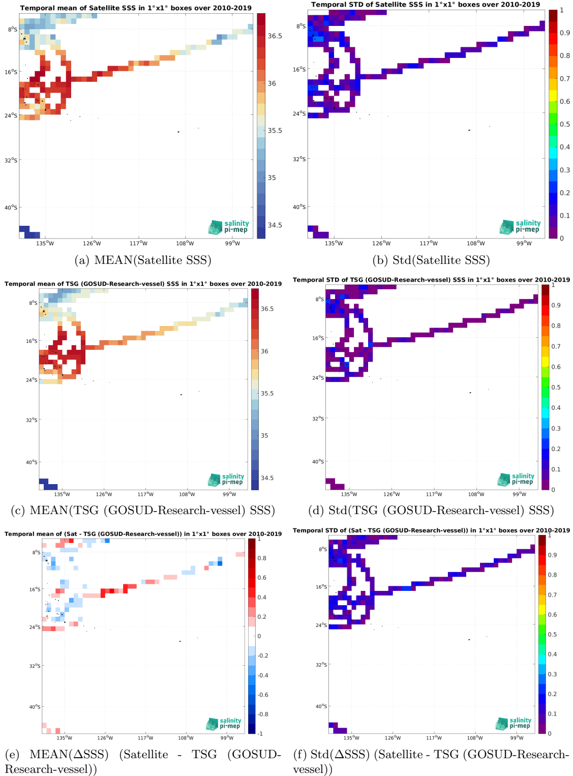
Figure 6: Temporal mean (left) and Std (right) of SSS from SMOS SSS L3 v9 - 9 Days (CATDS-CEC-LOCEAN) (top), TSG (GOSUD-Research-vessel) (middle), and of \Delta SSS (Satellite - TSG (GOSUD-Research-vessel)). Only match-up pairs are used to generate these maps.
