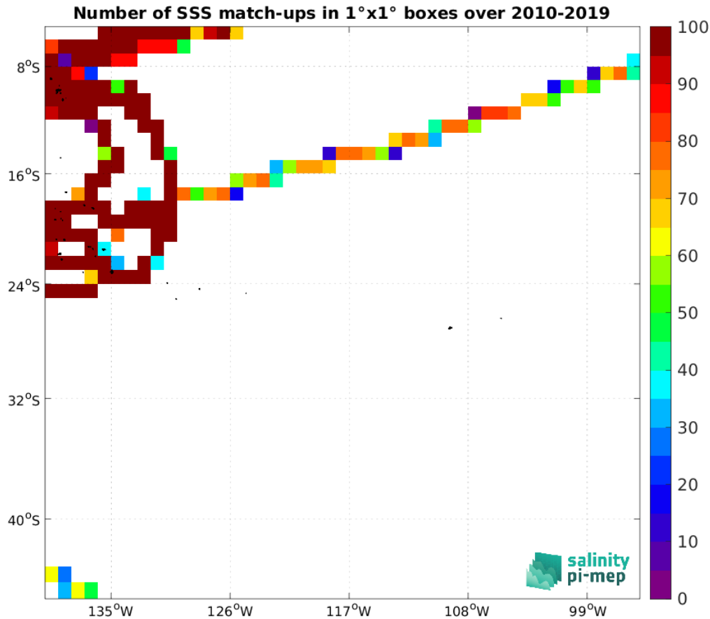
Figure 4: Number of SSS match-ups between TSG (GOSUD-Research-vessel) SSS and the SMOS SSS L3 v9 - 9 Days (CATDS-CEC-LOCEAN) SSS product for the OTT zone Pi-MEP region over 1^\circ \times 1^\circ boxes and for the full satellite product period.
