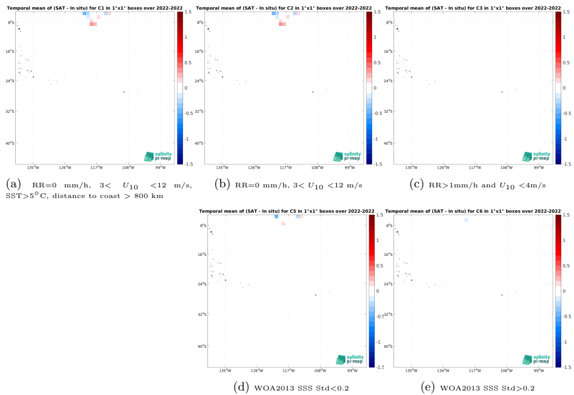
Figure 14: Temporal mean gridded over spatial boxes of size 1^\circ \times 1^\circ of \Delta SSS (SMOS SSS L3 v9 - 9 Days (CATDS-CEC-LOCEAN) - Saildrone) for 5 different subdatasets corresponding to:RR=0 mm/h, 3 < U_{10} < 12 m/s, SST >5^\circ\text{C} , distance to coast > 800 km (a), RR=0 mm/h, 3 < U_{10} < 12 m/s (b), RR >1 mm/h and U_{10} < 4 m/s (c), WOA2013 SSS Std <0.2 (d), WOA2013 SSS Std >0.2 (e).
