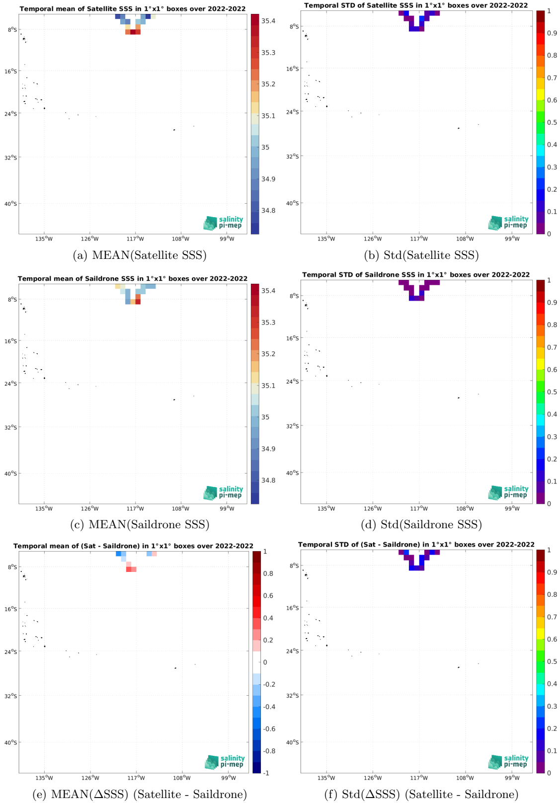
Figure 6: Temporal mean (left) and Std (right) of SSS from SMOS SSS L3 v9 - 9 Days (CATDS-CEC-LOCEAN) (top), Saildrone (middle), and of \Delta SSS (Satellite - Saildrone). Only match-up pairs are used to generate these maps.
