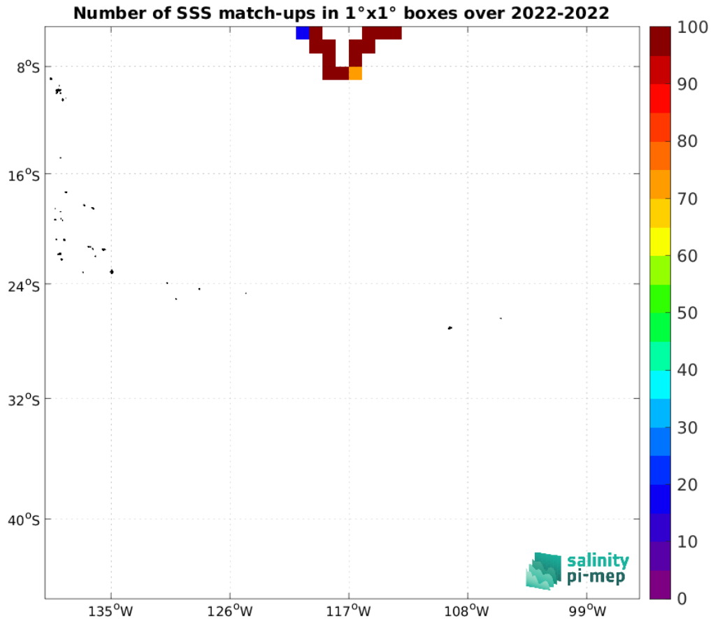
Figure 4: Number of SSS match-ups between Saildrone SSS and the SMOS SSS L3 v9 - 9 Days (CATDS-CEC-LOCEAN) SSS product for the OTT zone Pi-MEP region over 1^\circ \times 1^\circ boxes and for the full satellite product period.
