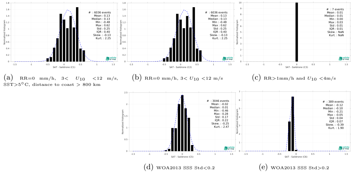
Figure 13: Normalized histogram of \Delta SSS (SMOS SSS L3 v9 - 9 Days (CATDS-CEC-LOCEAN) - Saildrone) for 5 different subdatasets corresponding to: RR=0 mm/h, 3 < U_{10} < 12 m/s, SST > 5°C, distance to coast > 800 km (a), RR=0 mm/h, 3 < U_{10} < 12 m/s (b), RR > 1mm/h and U_{10} < 4 m/s (c), WOA2013 SSS Std < 0.2 (d), WOA2013 SSS Std > 0.2 (e).
