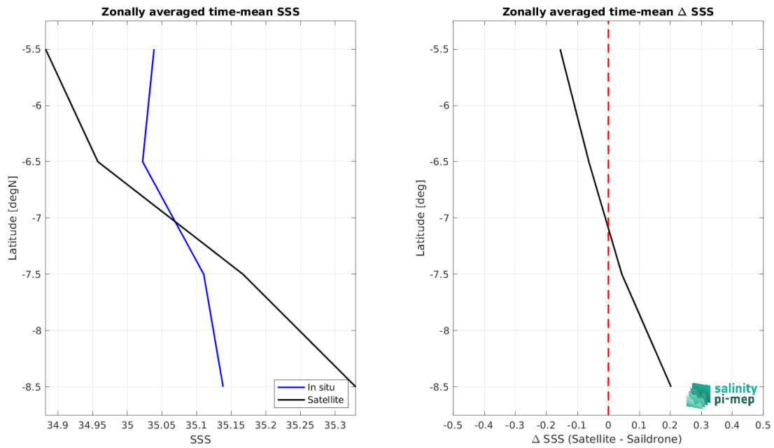
Figure 8: Left panel: Zonal mean SSS from SMOS SSS L3 v9 - 9 Days (CATDS-CEC-LOCEAN) satellite product (black) and from Sairdrone (blue). Right panel: Zonal mean of \Delta SSS (Satellite - Sairdrone) for all the collected Pi-MEP match-up pairs estimated over the full satellite product period.
