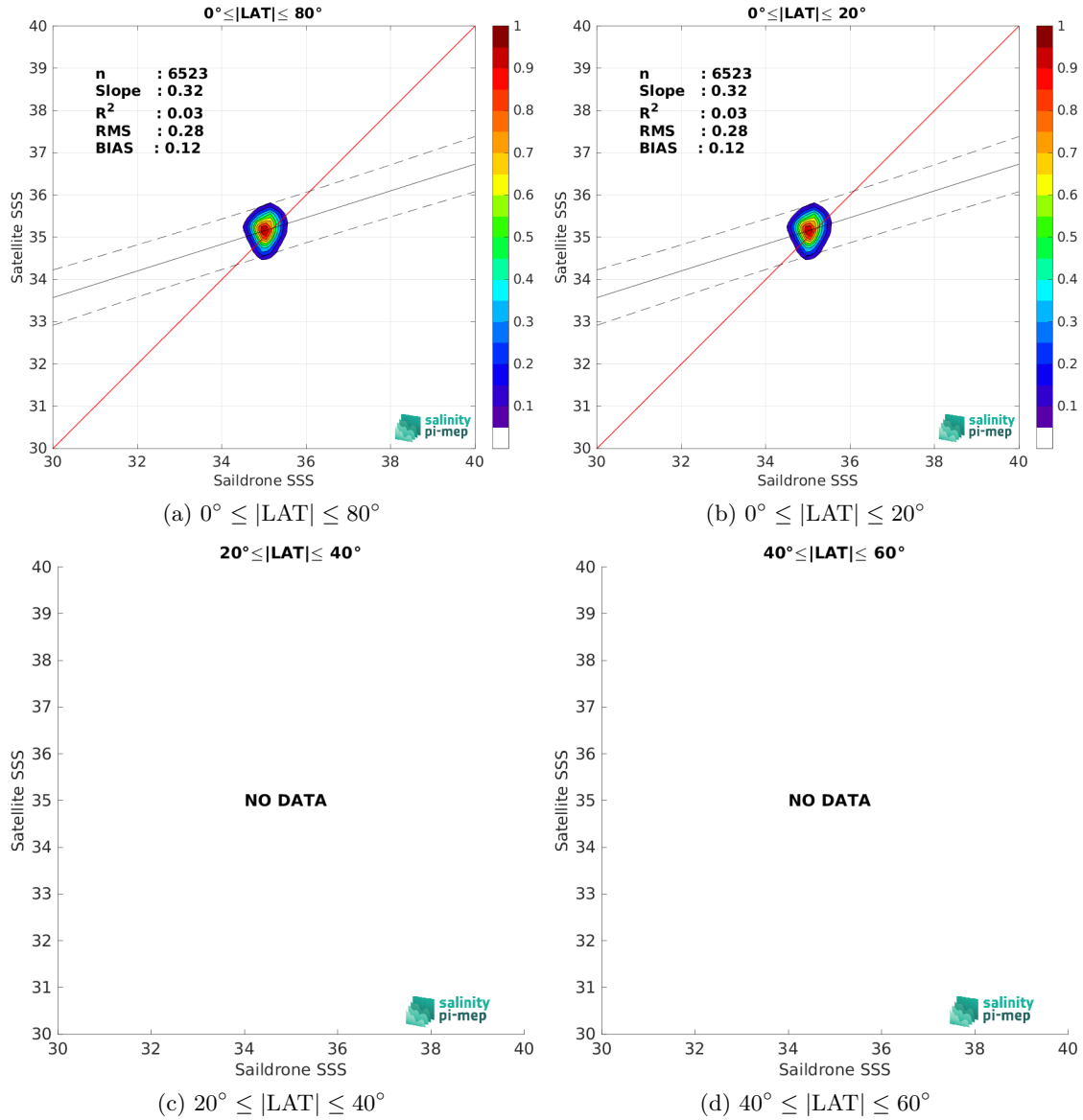
Figure 9: Contour maps of the concentration of SMOS SSS L3 v9 - 9 Days (CATDS-CEC-LOCEAN) SSS (y-axis) versus Saildrone SSS (x-axis) at match-up pairs for different latitude bands. For each plot, the red line shows x=y . The black thin and dashed lines indicate a linear fit through the data cloud and the \pm 95\% confidence levels, respectively. The number match-up pairs n , the slope and R^2 coefficient of the linear fit, the root mean square (RMS) and the mean bias between satellite and in situ data are indicated for each latitude band in each plots.
