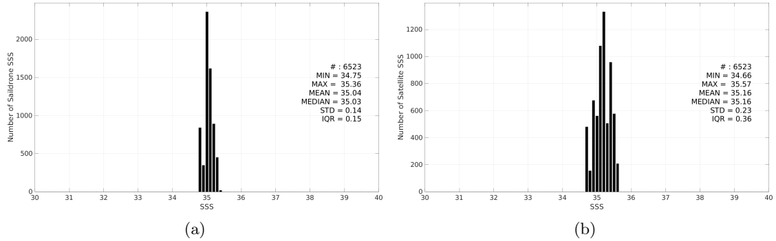
Figure 2: Histograms of SSS from Saildrone (a) and SMOS SSS L3 v9 - 9 Days (CATDS-CEC-LOCEAN) (b) considering all match-up pairs per bins of 0.1 over the OTT zone Pi-MEP region and for the full satellite product period.
