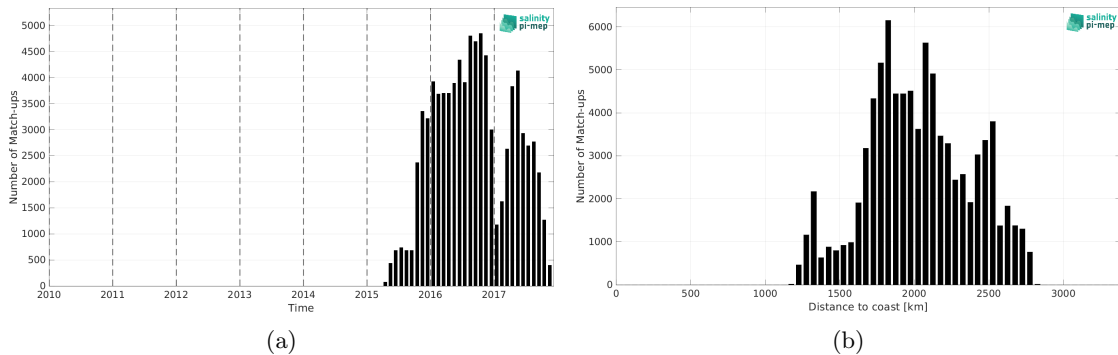
Figure 2: Number of match-ups between Surface drifters and SMOS SSS L3 v9 - 9 Days (CATDS-CEC-LOCEAN) SSS as a function of time (a) and as function of the distance to coast (b) over the OTT zone Pi-MEP region and for the full satellite product period.
