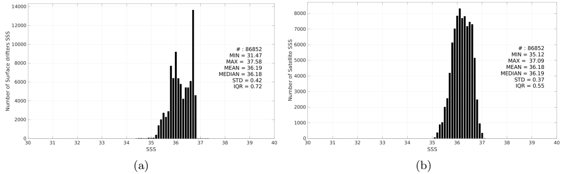
Figure 3: Histograms of SSS from Surface drifters (a) and SMOS SSS L3 v9 - 9 Days (CATDS-CEC-LOCEAN) (b) considering all match-up pairs per bins of 0.1 over the OTT zone Pi-MEP region and for the full satellite product period.
