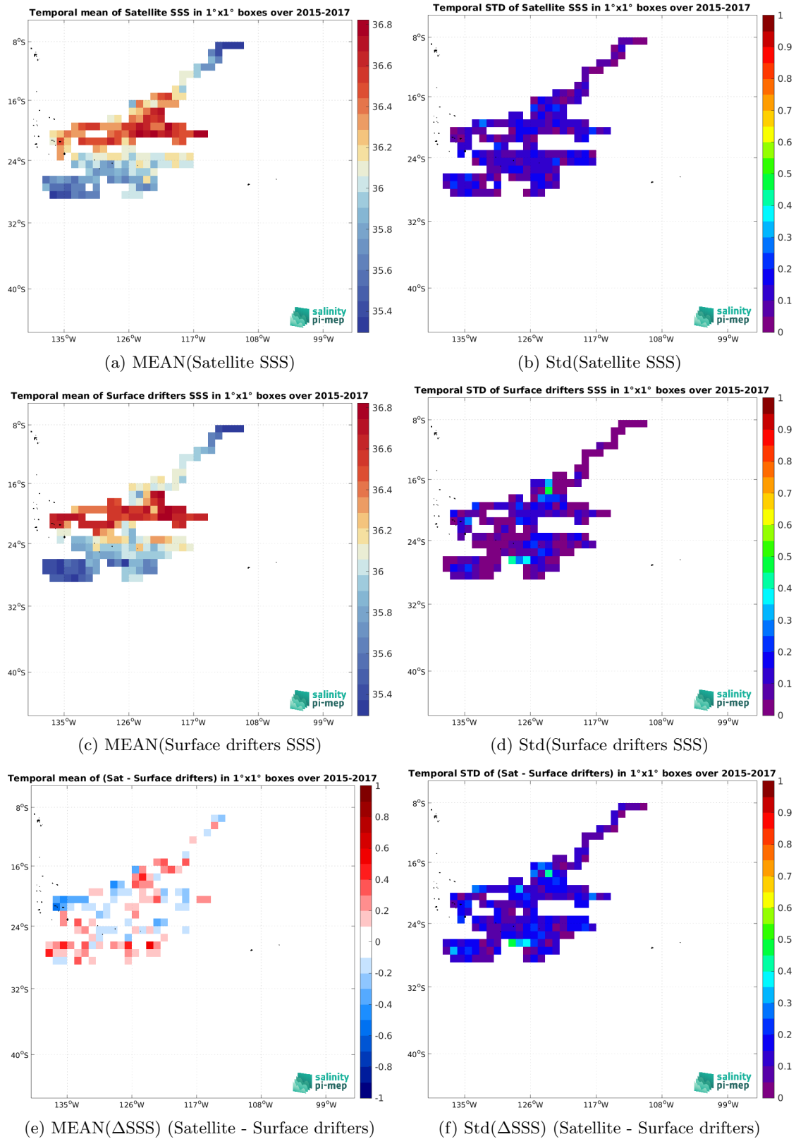
Figure 6: Temporal mean (left) and Std (right) of SSS from SMOS SSS L3 v9 - 9 Days (CATDS-CEC-LOCEAN) (top), Surface drifters (middle), and of \Delta SSS (Satellite - Surface drifters). Only match-up pairs are used to generate these maps.
