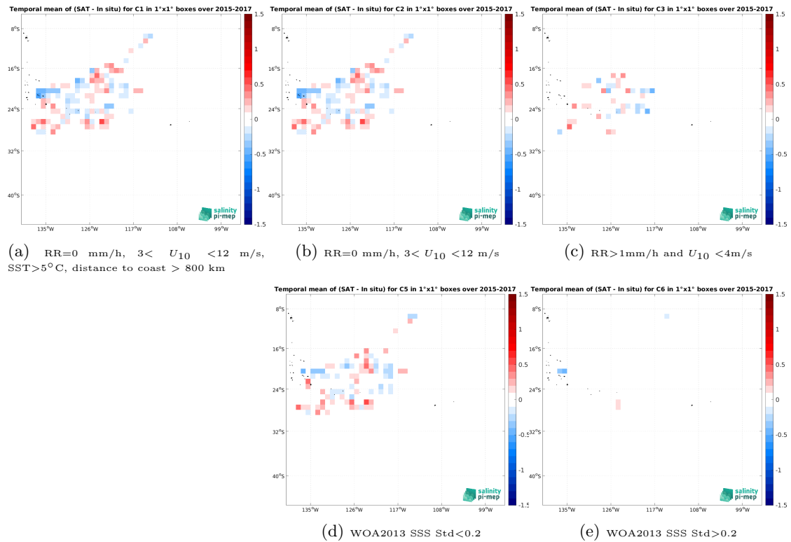
Figure 13: Temporal mean gridded over spatial boxes of size 1^\circ \times 1^\circ of \Delta SSS (SMOS SSS L3 v9 - 9 Days (CATDS-CEC-LOCEAN) - Surface drifters) for 5 different subdatasets corresponding to:RR=0 mm/h, 3 < U_{10} < 12 m/s, SST >5^\circ C, distance to coast > 800 km (a), RR=0 mm/h, 3 < U_{10} < 12 m/s (b), RR >1 mm/h and U_{10} < 4 m/s (c), WOA2013 SSS Std <0.2 (d), WOA2013 SSS Std >0.2 (e).
