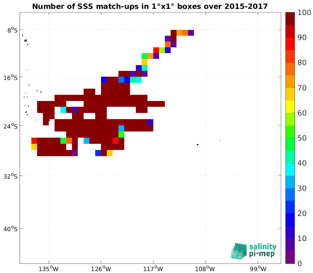
Figure 3: Number of SSS match-ups between Surface drifters SSS and the SMOS SSS L3 v9 - 9 Days (CATDS-CEC-LOCEAN) SSS product for the OTT zone Pi-MEP region over 1°x1° boxes and for the full satellite product period.
