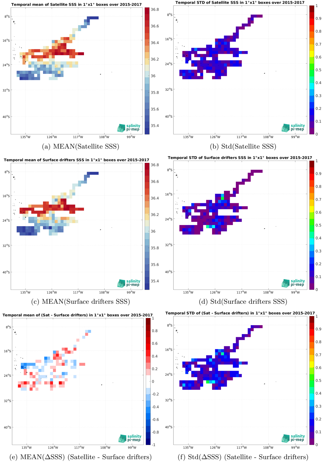
Figure 5: Temporal mean (left) and Std (right) of SSS from SMOS SSS L3 v9 - 9 Days (CATDS-CEC-LOCEAN) (top), Surface drifters (middle), and of \Delta SSS (Satellite - Surface drifters). Only match-up pairs are used to generate these maps.
