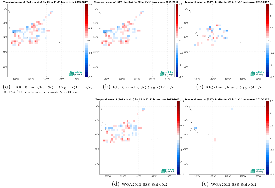
Figure 11: Temporal mean gridded over spatial boxes of size 1^{\circ}\times 1^{\circ} of \Delta\text{SSS} (SMOS SSS L3 v9 - 9 Days (CATDS-CEC-LOCEAN) - Surface drifters) for 5 different subdatasets corresponding to:RR=0 mm/h, 3 < U_{10} < 12 m/s, SST >5^{\circ}\text{C} , distance to coast > 800 km (a), RR=0 mm/h, 3 < U_{10} < 12 m/s (b), RR >1 mm/h and U_{10} < 4 m/s (c), WOA2013 SSS Std <0.2 (d), WOA2013 SSS Std >0.2 (e).
