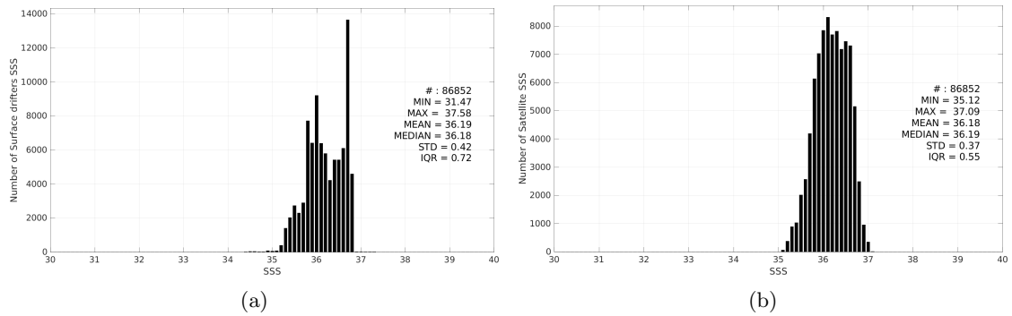
Figure 2: Histograms of SSS from Surface drifters (a) and SMOS SSS L3 v9 - 9 Days (CATDS-CEC-LOCEAN) (b) considering all match-up pairs per bins of 0.1 over the OTT zone Pi-MEP region and for the full satellite product period.
