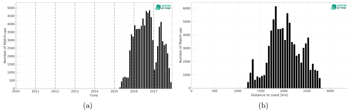
Figure 1: Number of match-ups between Surface drifters and SMOS SSS L3 v9 - 9 Days (CATDS-CEC-LOCEAN) SSS as a function of time (a) and as function of the distance to coast (b) over the OTT zone Pi-MEP region and for the full satellite product period.
