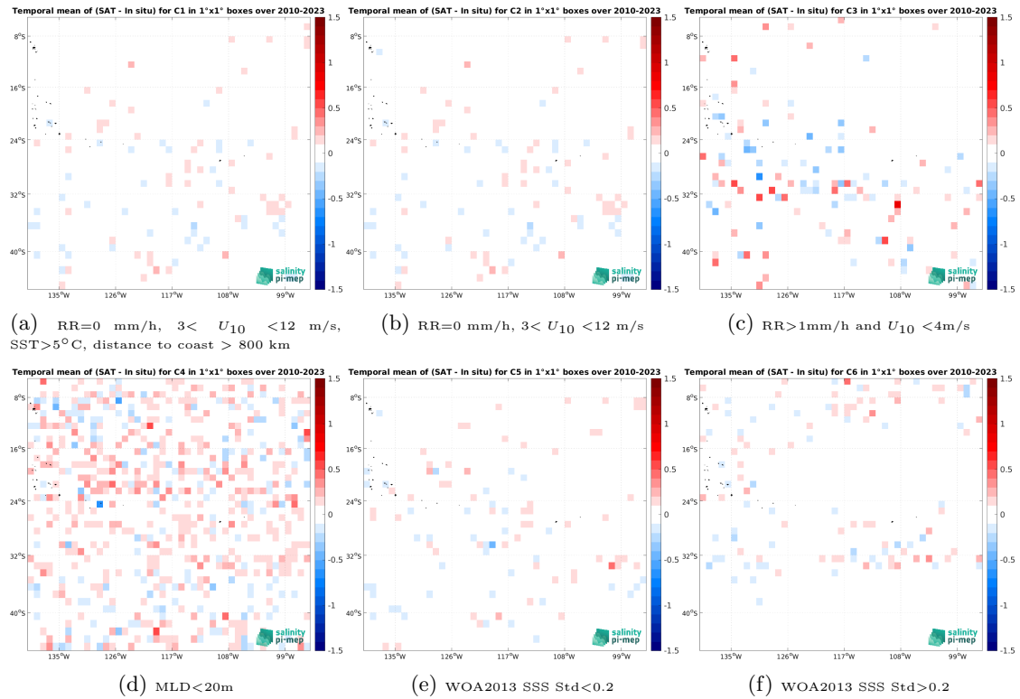
Figure 14: Temporal mean gridded over spatial boxes of size 1^\circ \times 1^\circ of \Delta SSS (SMOS SSS L3 v9 - 9 Days (CATDS-CEC-LOCEAN) - Argo) for 6 different subdatasets corresponding to: RR=0 mm/h, 3 < U_{10} < 12 m/s, SST > 5^\circ C , distance to coast > 800 km (a), RR=0 mm/h, 3 < U_{10} < 12 m/s (b), RR > 1 mm/h and U_{10} < 4 m/s (c), MLD < 20 m (d), WOA2013 SSS Std < 0.2 (e), WOA2013 SSS Std > 0.2 (f).
