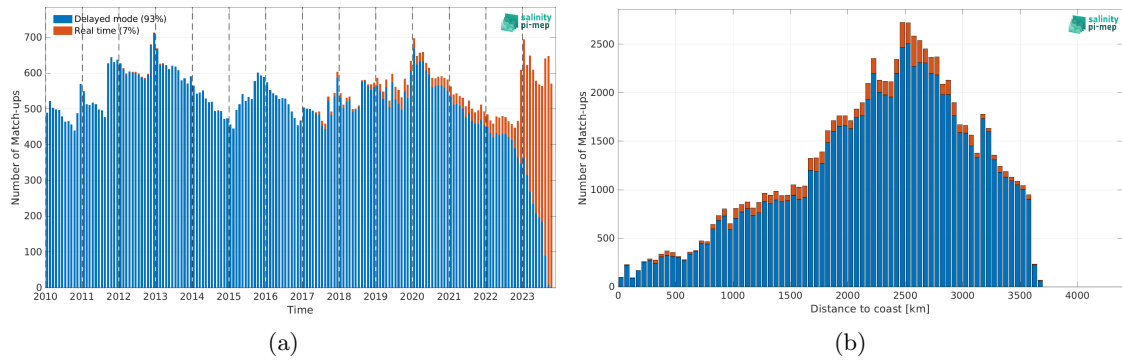
Figure 1: Number of match-ups between Argo and SMOS SSS L3 v9 - 9 Days (CATDS-CEC-LOCEAN) SSS as a function of time (a) and as function of the distance to coast (b) over the OTT zone Pi-MEP region and for the full satellite product period.
