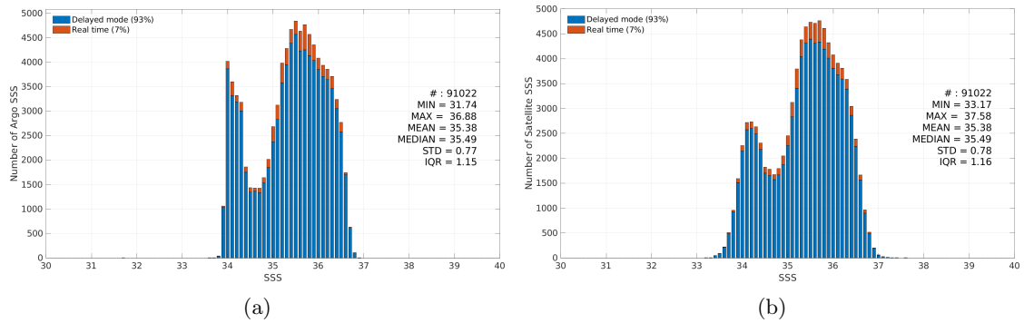
Figure 2: Histograms of SSS from Argo (a) and SMOS SSS L3 v9 - 9 Days (CATDS-CEC-LOCEAN) (b) considering all match-up pairs per bins of 0.1 over the OTT zone Pi-MEP region and for the full satellite product period.
