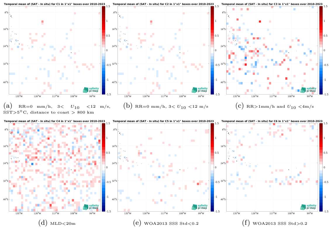
Figure 12: Temporal mean gridded over spatial boxes of size 1^\circ \times 1^\circ of \Delta SSS (SMOS SSS L3 v9 - 9 Days (CATDS-CEC-LOCEAN) - Argo) for 6 different subdatasets corresponding to:RR=0 mm/h, 3 < U_{10} < 12 m/s, SST >5^\circ C, distance to coast > 800 km (a), RR=0 mm/h, 3 < U_{10} < 12 m/s (b), RR >1 mm/h and U_{10} < 4 m/s (c),MLD <20 m (d),WOA2013 SSS Std <0.2 (e),WOA2013 SSS Std >0.2 (f).
