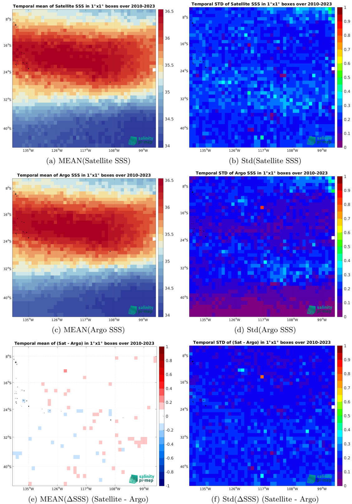
Figure 6: Temporal mean (left) and Std (right) of SSS from SMOS SSS L3 v9 - 9 Days (CATDS-CEC-LOCEAN) (top), Argo (middle), and of \Delta SSS (Satellite - Argo). Only match-up pairs are used to generate these maps.
