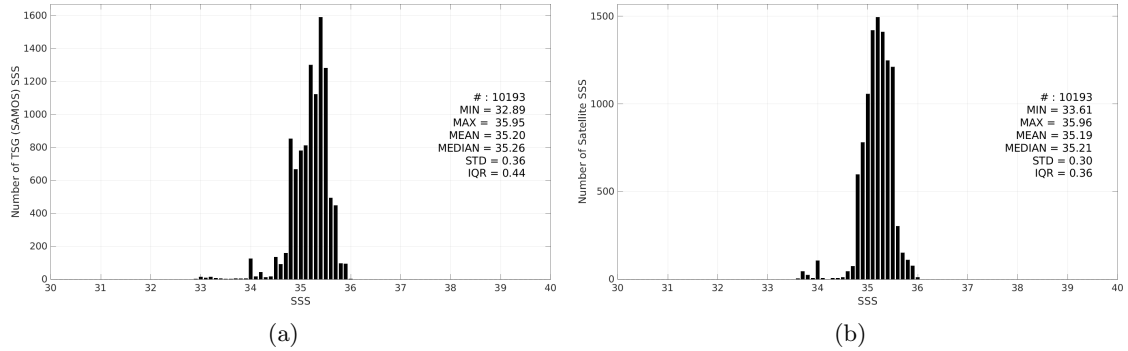
Figure 3: Histograms of SSS from TSG (SAMOS) (a) and SMOS SSS L3 v9 - 18 Days (CATDS-CEC-LOCEAN) (b) considering all match-up pairs per bins of 0.1 over the OTT zone Pi-MEP region and for the full satellite product period.
