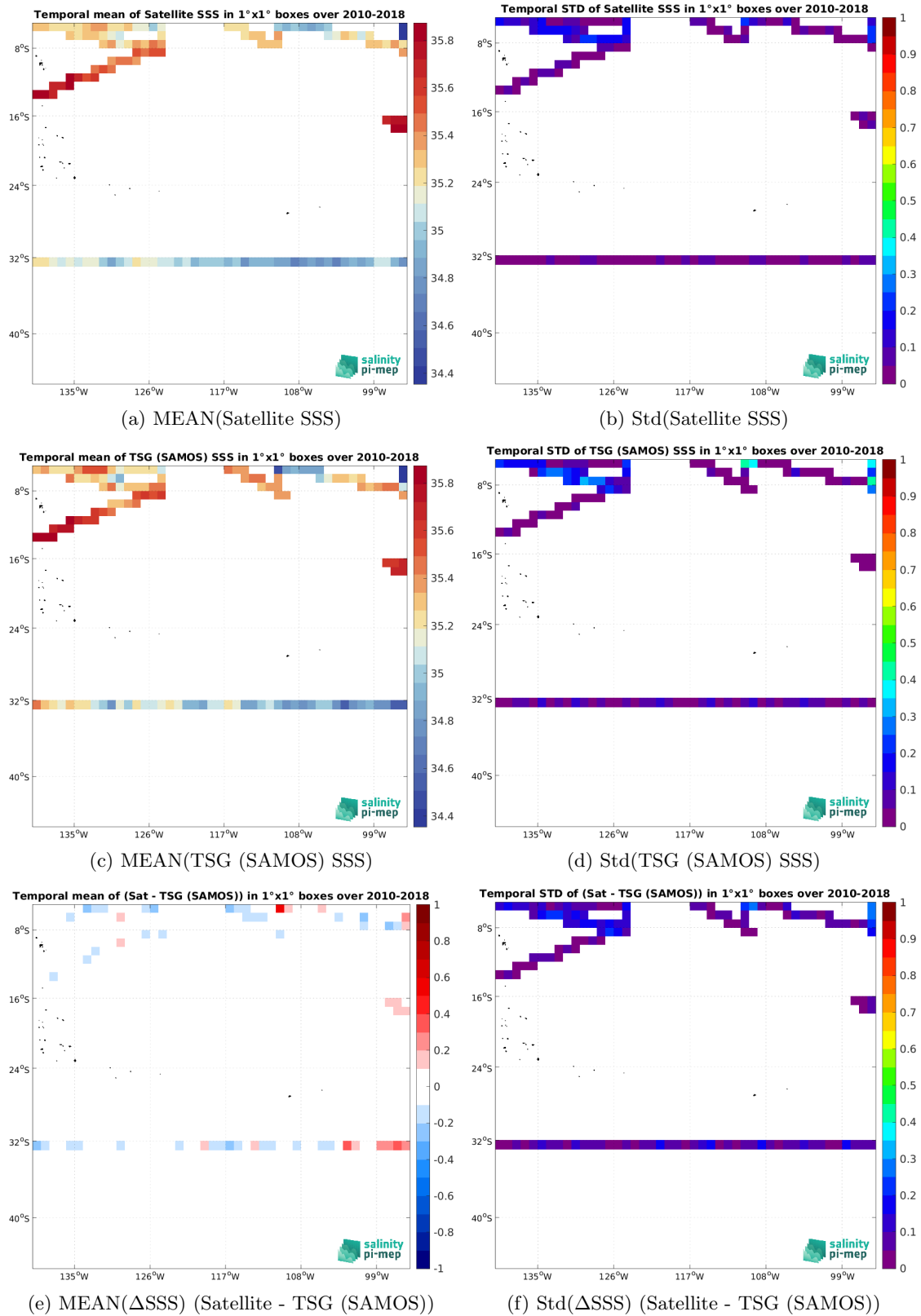
Figure 7: Temporal mean (left) and Std (right) of SSS from SMOS SSS L3 v9 - 18 Days (CATDS-CEC-LOCEAN) (top), TSG (SAMOS) (middle), and of \Delta SSS (Satellite - TSG (SAMOS)). Only match-up pairs are used to generate these maps.
