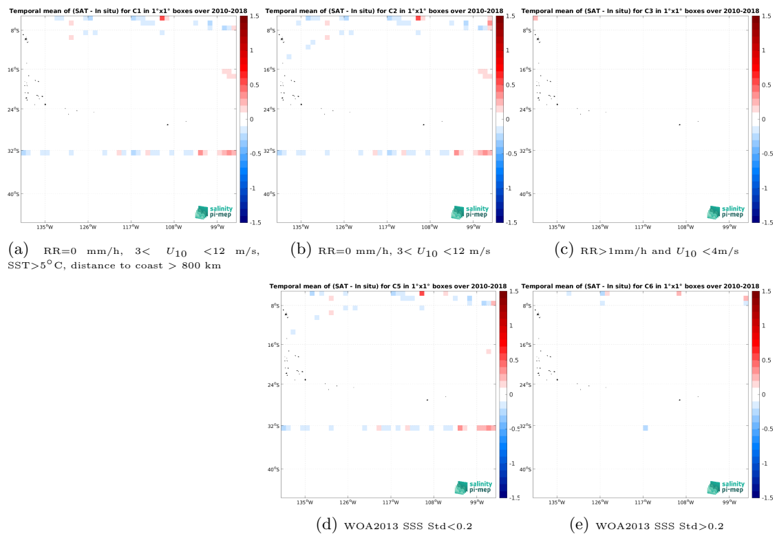
Figure 14: Temporal mean gridded over spatial boxes of size 1^\circ \times 1^\circ of \Delta SSS (SMOS SSS L3 v9 - 18 Days (CATDS-CEC-LOCEAN) - TSG (SAMOS)) for 5 different subdatasets corresponding to: RR=0 mm/h, 3 < U_{10} < 12 m/s, SST > 5^\circ\text{C} , distance to coast > 800 km (a), RR=0 mm/h, 3 < U_{10} < 12 m/s (b), RR > 1 mm/h and U_{10} < 4 m/s (c), WOA2013 SSS Std < 0.2 (d), WOA2013 SSS Std > 0.2 (e).
