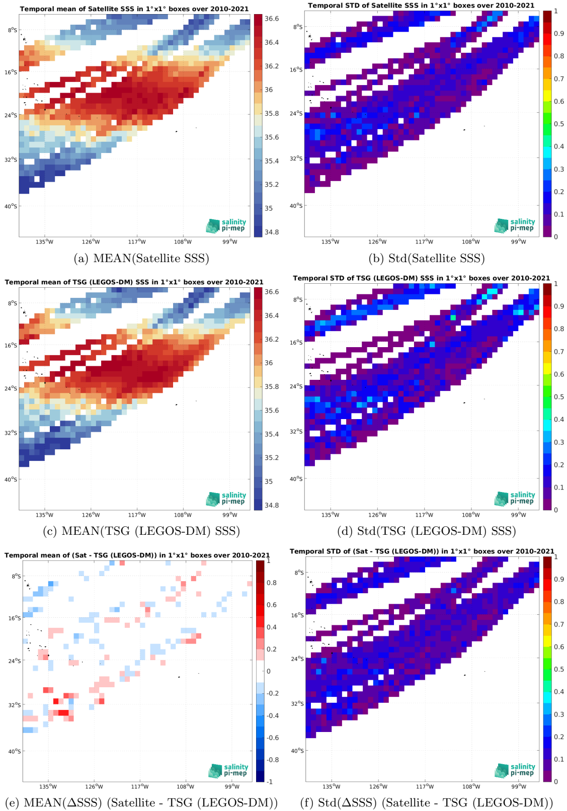
Figure 7: Temporal mean (left) and Std (right) of SSS from SMOS SSS L3 v9 - 18 Days (CATDS-CEC-LOCEAN) (top), TSG (LEGOS-DM) (middle), and of \Delta SSS (Satellite - TSG (LEGOS-DM)). Only match-up pairs are used to generate these maps.
