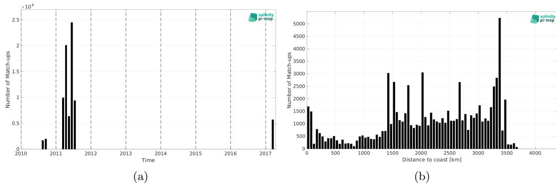
Figure 2: Number of match-ups between TSG (GOSUD-Sailing-ship) and SMOS SSS L3 v9 - 18 Days (CATDS-CEC-LOCEAN) SSS as a function of time (a) and as function of the distance to coast (b) over the OTT zone Pi-MEP region and for the full satellite product period.
