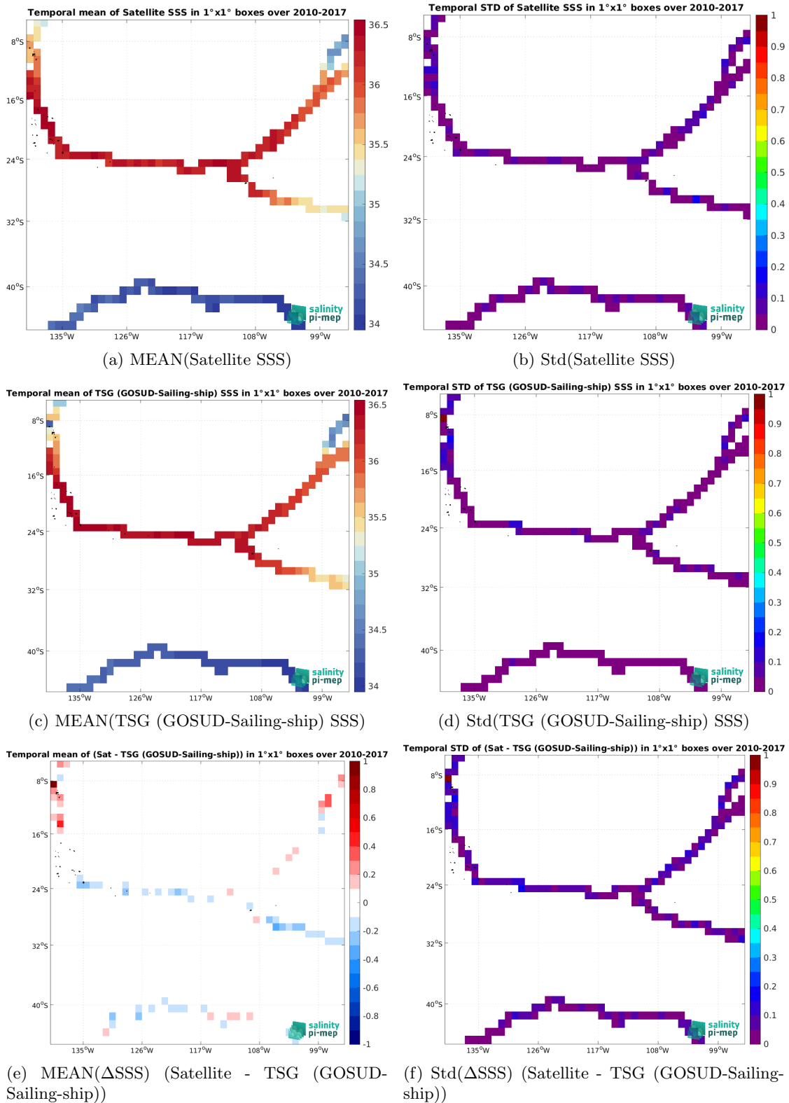
Figure 7: Temporal mean (left) and Std (right) of SSS from SMOS SSS L3 v9 - 18 Days (CATDS-CEC-LOCEAN) (top), TSG (GOSUD-Sailing-ship) (middle), and of \Delta\text{SSS} (Satellite - TSG (GOSUD-Sailing-ship)). Only match-up pairs are used to generate these maps.
