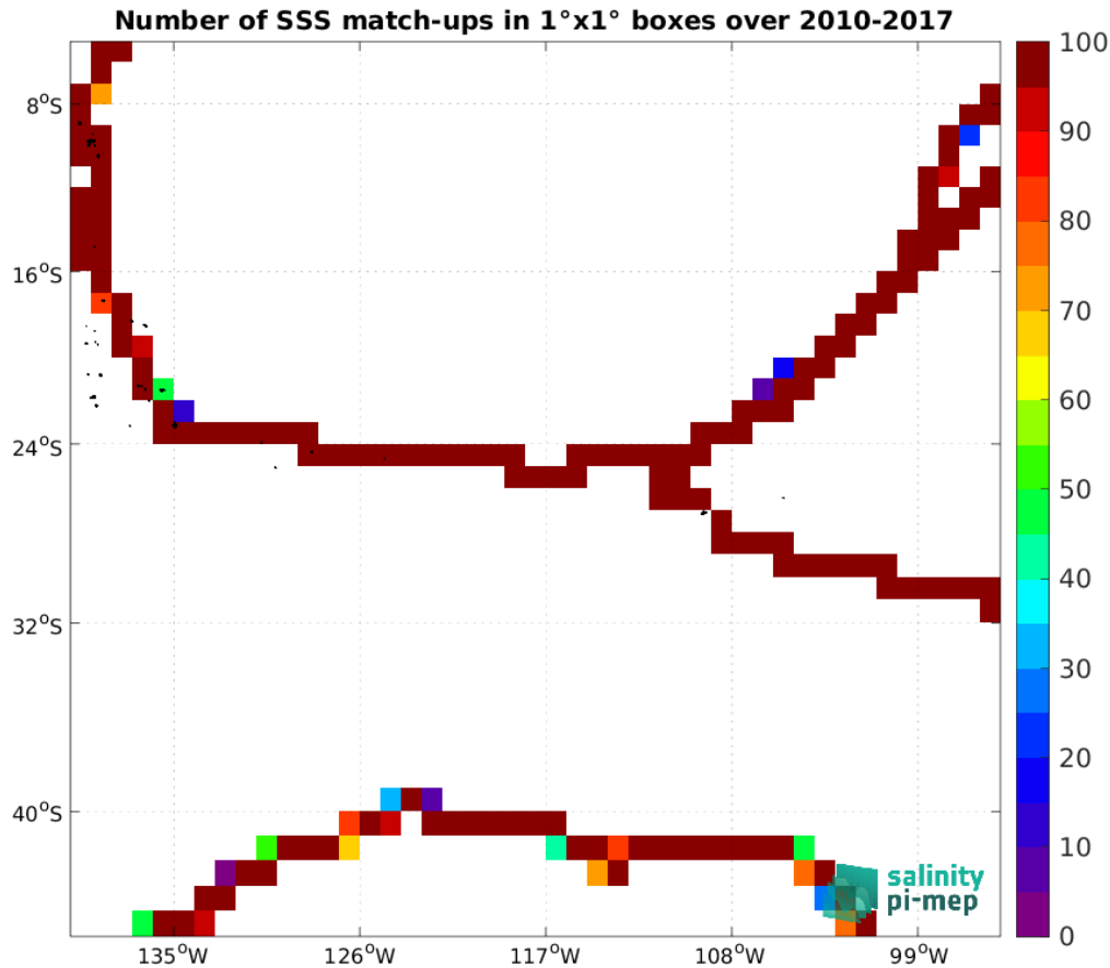
Figure 5: Number of SSS match-ups between TSG (GOSUD-Sailing-ship) SSS and the SMOS SSS L3 v9 - 18 Days (CATDS-CEC-LOCEAN) SSS product for the OTT zone Pi-MEP region over 1^\circ \times 1^\circ boxes and for the full satellite product period.
