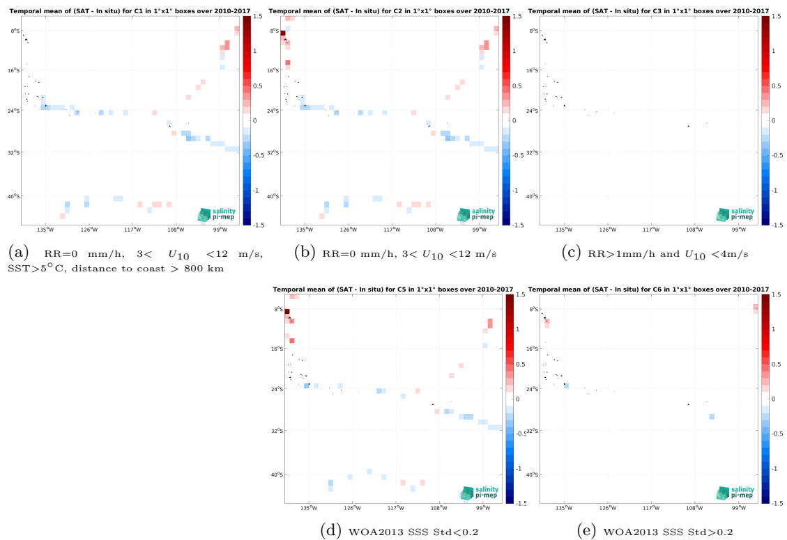
Figure 12: Temporal mean gridded over spatial boxes of size 1^\circ \times 1^\circ of \Delta SSS (SMOS SSS L3 v9 - 18 Days (CATDS-CEC-LOCEAN) - TSG (GOSUD-Sailing-ship)) for 5 different subdatasets corresponding to:RR=0 mm/h, 3 < U_{10} < 12 m/s, SST >5^\circ\text{C} , distance to coast > 800 km (a), RR=0 mm/h, 3 < U_{10} < 12 m/s (b), RR >1 mm/h and U_{10} < 4 m/s (c), WOA2013 SSS Std <0.2 (d), WOA2013 SSS Std >0.2 (e).
