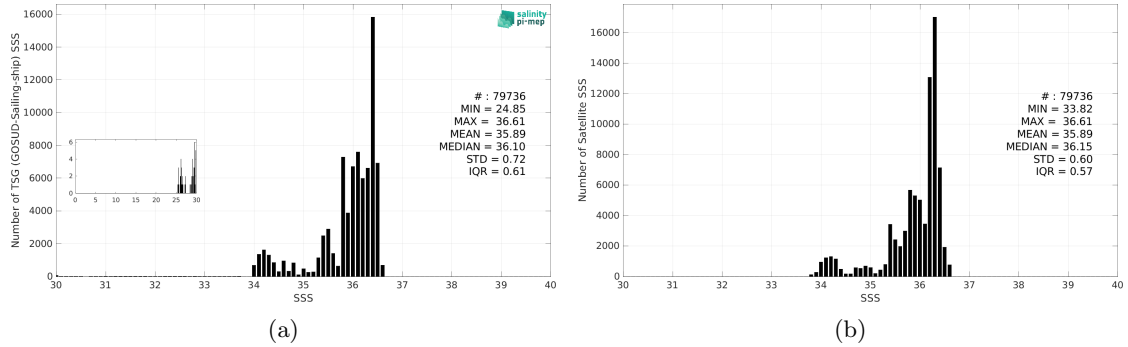
Figure 2: Histograms of SSS from TSG (GOSUD-Sailing-ship) (a) and SMOS SSS L3 v9 - 18 Days (CATDS-CEC-LOCEAN) (b) considering all match-up pairs per bins of 0.1 over the OTT zone Pi-MEP region and for the full satellite product period.
