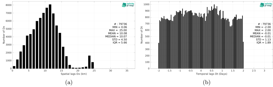
Figure 5: Histograms of the spatial (a) and temporal (b) lags between the location/time of the TSG (GOSUD-Sailing-ship) measurement and the date of the corresponding SMOS SSS L3 v9 - 18 Days (CATDS-CEC-LOCEAN) SSS pixel.
