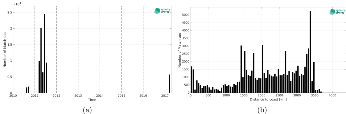
Figure 1: Number of match-ups between TSG (GOSUD-Sailing-ship) and SMOS SSS L3 v9 - 18 Days (CATDS-CEC-LOCEAN) SSS as a function of time (a) and as function of the distance to coast (b) over the OTT zone Pi-MEP region and for the full satellite product period.
