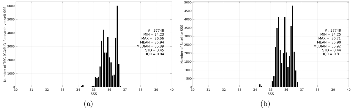
Figure 3: Histograms of SSS from TSG (GOSUD-Research-vessel) (a) and SMOS SSS L3 v9 - 18 Days (CATDS-CEC-LOCEAN) (b) considering all match-up pairs per bins of 0.1 over the OTT zone Pi-MEP region and for the full satellite product period.
