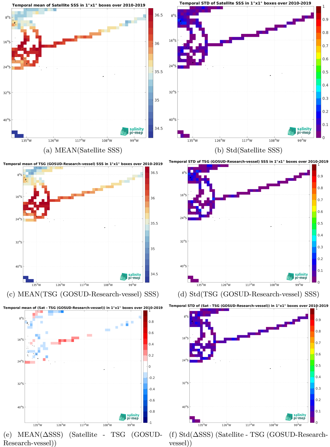
Figure 7: Temporal mean (left) and Std (right) of SSS from SMOS SSS L3 v9 - 18 Days (CATDS-CEC-LOCEAN) (top), TSG (GOSUD-Research-vessel) (middle), and of \Delta SSS (Satellite - TSG (GOSUD-Research-vessel)). Only match-up pairs are used to generate these maps.
