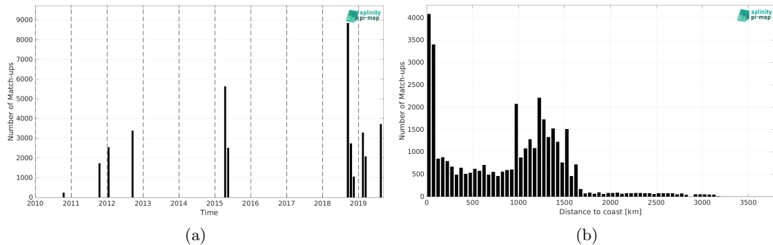
Figure 2: Number of match-ups between TSG (GOSUD-Research-vessel) and SMOS SSS L3 v9 - 18 Days (CATDS-CEC-LOCEAN) SSS as a function of time (a) and as function of the distance to coast (b) over the OTT zone Pi-MEP region and for the full satellite product period.
