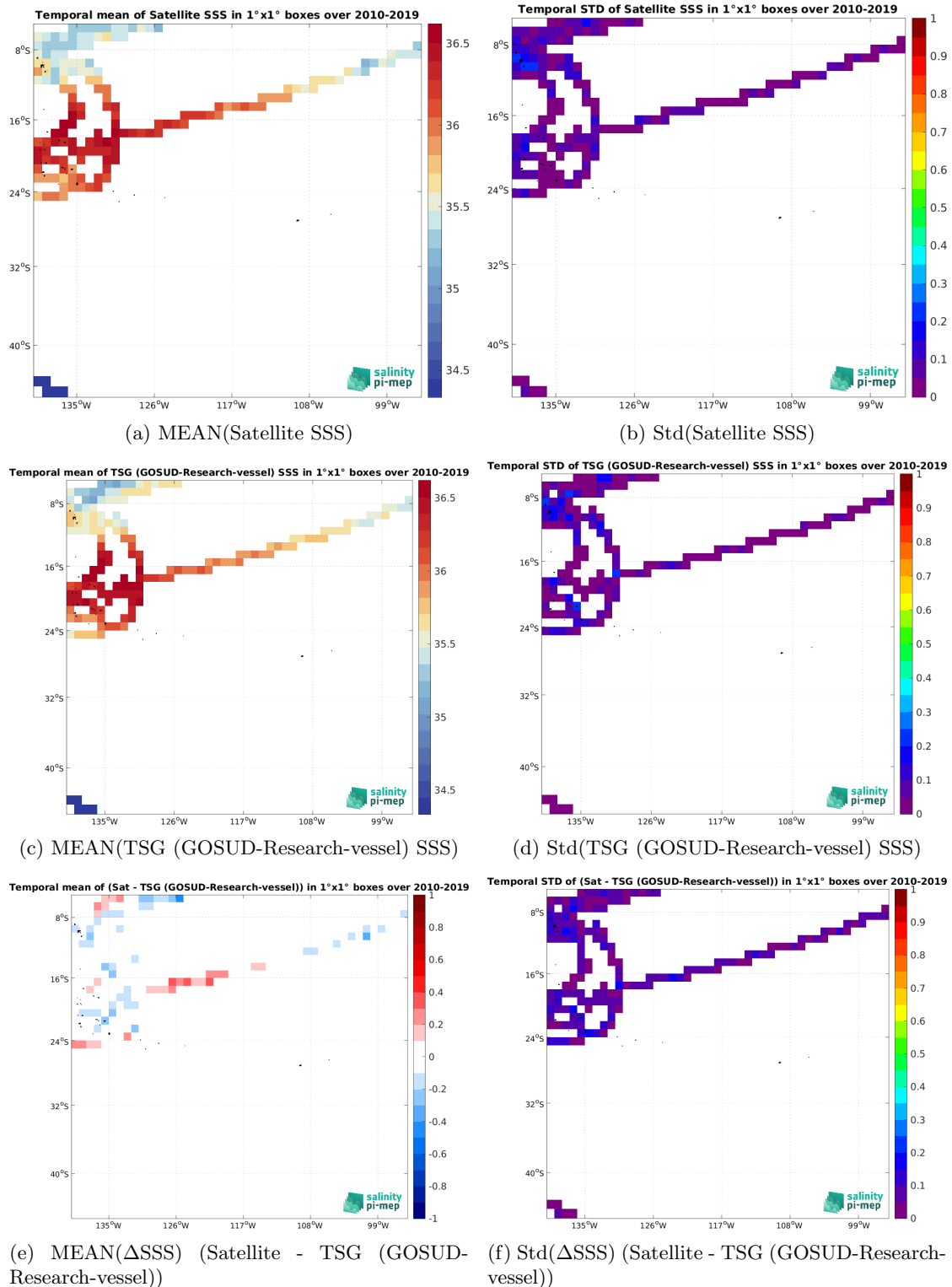
Figure 6: Temporal mean (left) and Std (right) of SSS from SMOS SSS L3 v9 - 18 Days (CATDS-CEC-LOCEAN) (top), TSG (GOSUD-Research-vessel) (middle), and of \Delta SSS (Satellite - TSG (GOSUD-Research-vessel)). Only match-up pairs are used to generate these maps.
