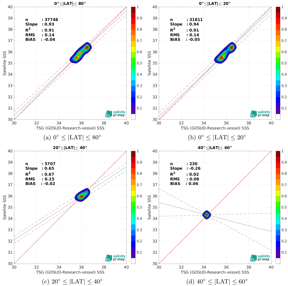
Figure 9: Contour maps of the concentration of SMOS SSS L3 v9 - 18 Days (CATDS-CEC-LOCEAN) SSS ( y -axis) versus TSG (GOSUD-Research-vessel) SSS ( x -axis) at match-up pairs for different latitude bands. For each plot, the red line shows x=y . The black thin and dashed lines indicate a linear fit through the data cloud and the \pm 95\% confidence levels, respectively. The number match-up pairs n , the slope and R^2 coefficient of the linear fit, the root mean square (RMS) and the mean bias between satellite and in situ data are indicated for each latitude band in each plots.
