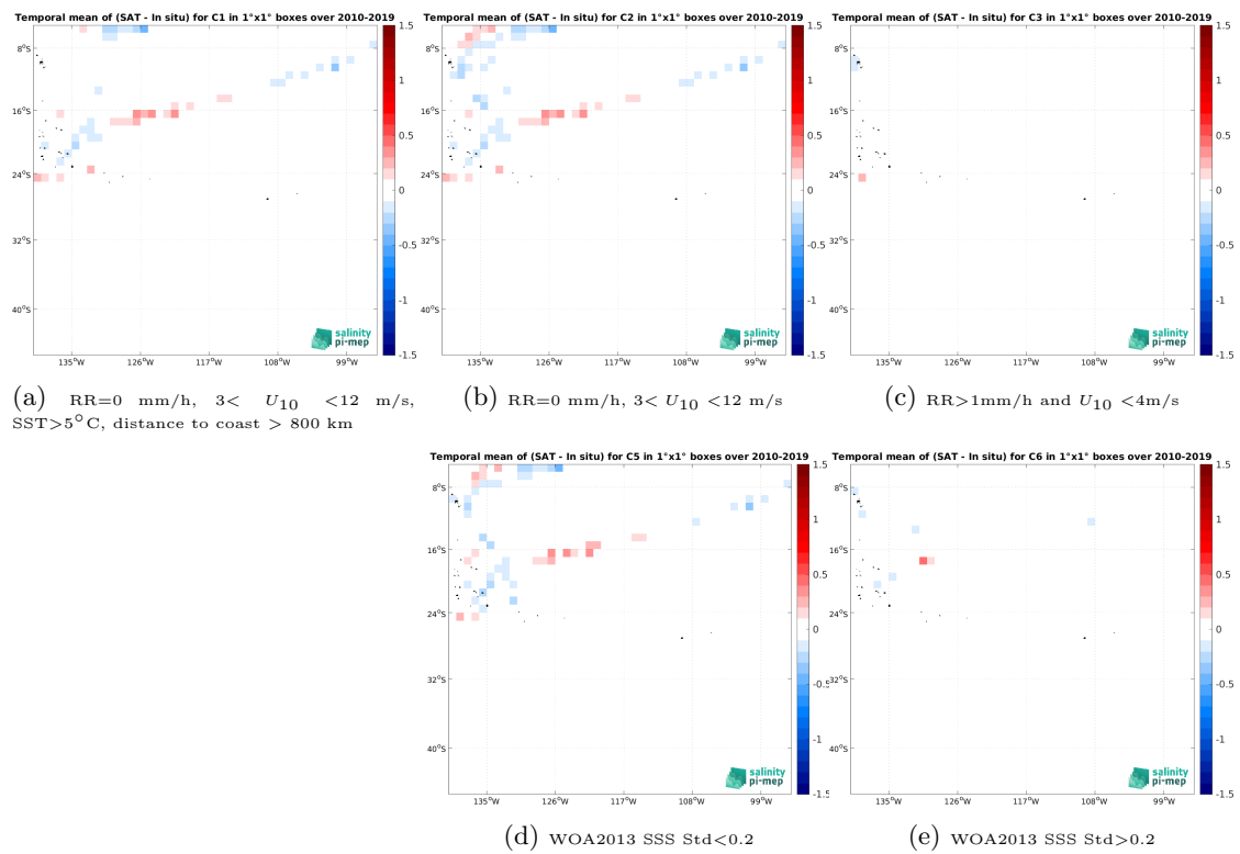
Figure 12: Temporal mean gridded over spatial boxes of size 1^\circ \times 1^\circ of \Delta SSS (SMOS SSS L3 v9 - 18 Days (CATDS-CEC-LOCEAN) - TSG (GOSUD-Research-vessel)) for 5 different subdatasets corresponding to: RR=0 mm/h, 3 < U_{10} < 12 m/s, SST > 5^\circ C , distance to coast > 800 km (a), RR=0 mm/h, 3 < U_{10} < 12 m/s (b), RR > 1 mm/h and U_{10} < 4 m/s (c), WOA2013 SSS Std < 0.2 (d), WOA2013 SSS Std > 0.2 (e).
