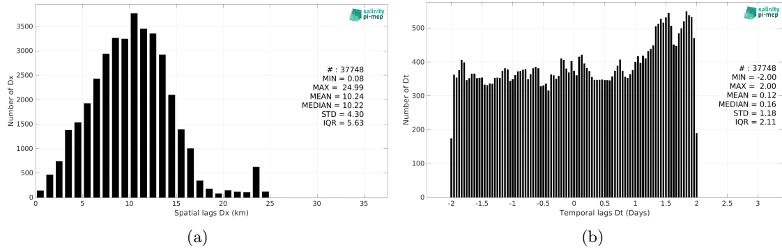
Figure 5: Histograms of the spatial (a) and temporal (b) lags between the location/time of the TSG (GOSUD-Research-vessel) measurement and the date of the corresponding SMOS SSS L3 v9 - 18 Days (CATDS-CEC-LOCEAN) SSS pixel.
