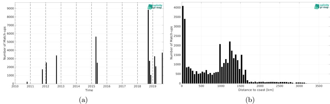
Figure 1: Number of match-ups between TSG (GOSUD-Research-vessel) and SMOS SSS L3 v9 - 18 Days (CATDS-CEC-LOCEAN) SSS as a function of time (a) and as function of the distance to coast (b) over the OTT zone Pi-MEP region and for the full satellite product period.
