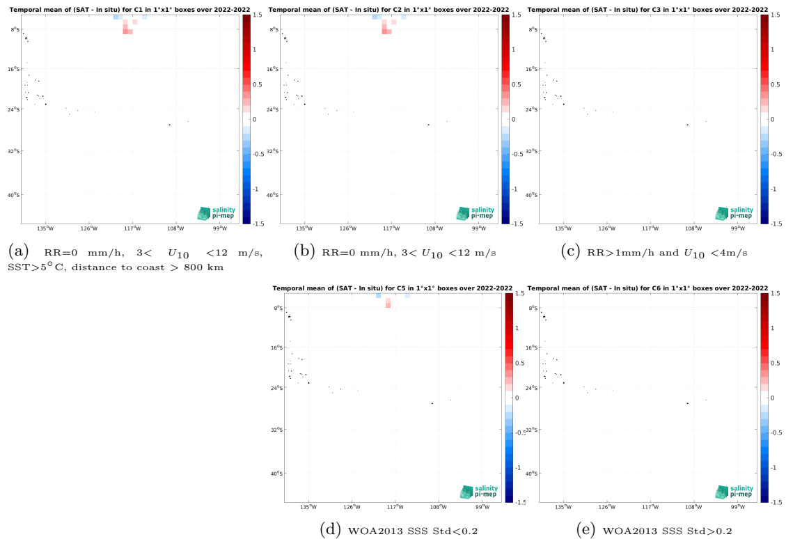
Figure 14: Temporal mean gridded over spatial boxes of size 1^\circ \times 1^\circ of \Delta SSS (SMOS SSS L3 v9 - 18 Days (CATDS-CEC-LOCEAN) - Sairdrone) for 5 different subdatasets corresponding to:RR=0 mm/h, 3 < U_{10} < 12 m/s, SST >5^\circ\text{C} , distance to coast > 800 km (a), RR=0 mm/h, 3 < U_{10} < 12 m/s (b), RR >1 mm/h and U_{10} < 4 m/s (c), WOA2013 SSS Std <0.2 (d), WOA2013 SSS Std >0.2 (e).
