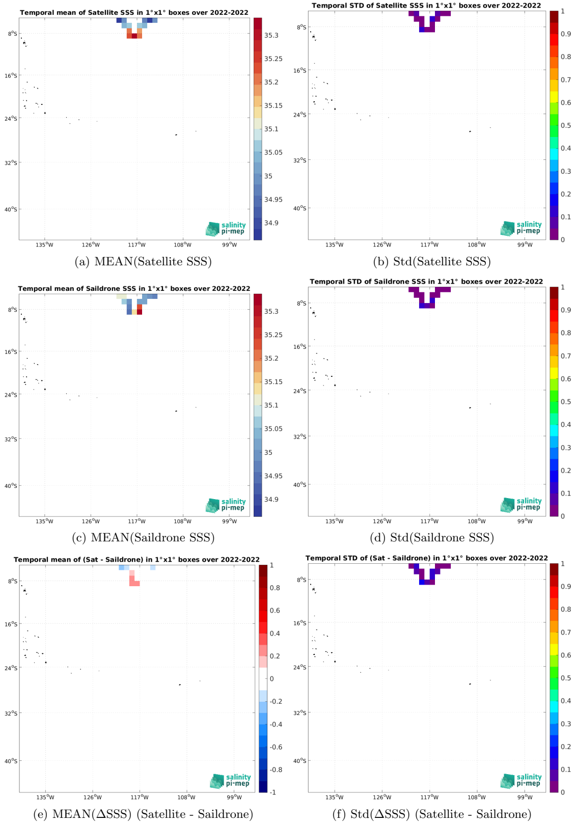
Figure 7: Temporal mean (left) and Std (right) of SSS from SMOS SSS L3 v9 - 18 Days (CATDS-CEC-LOCEAN) (top), Saildrone (middle), and of \Delta SSS (Satellite - Saildrone). Only match-up pairs are used to generate these maps.
