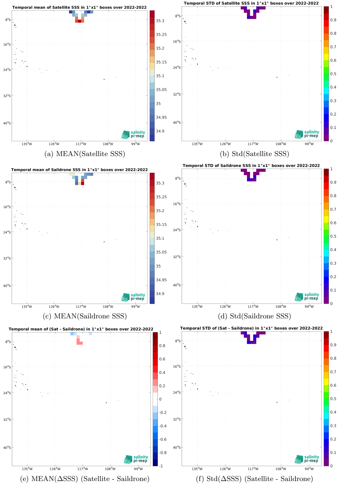
Figure 6: Temporal mean (left) and Std (right) of SSS from SMOS SSS L3 v9 - 18 Days (CATDS-CEC-LOCEAN) (top), Saildrone (middle), and of \Delta SSS (Satellite - Saildrone). Only match-up pairs are used to generate these maps.
