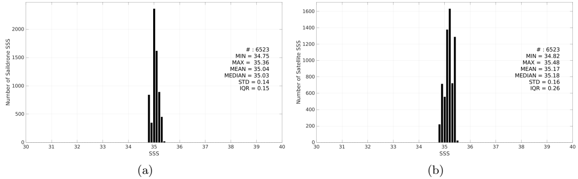
Figure 2: Histograms of SSS from Saildrone (a) and SMOS SSS L3 v9 - 18 Days (CATDS-CEC-LOCEAN) (b) considering all match-up pairs per bins of 0.1 over the OTT zone Pi-MEP region and for the full satellite product period.
