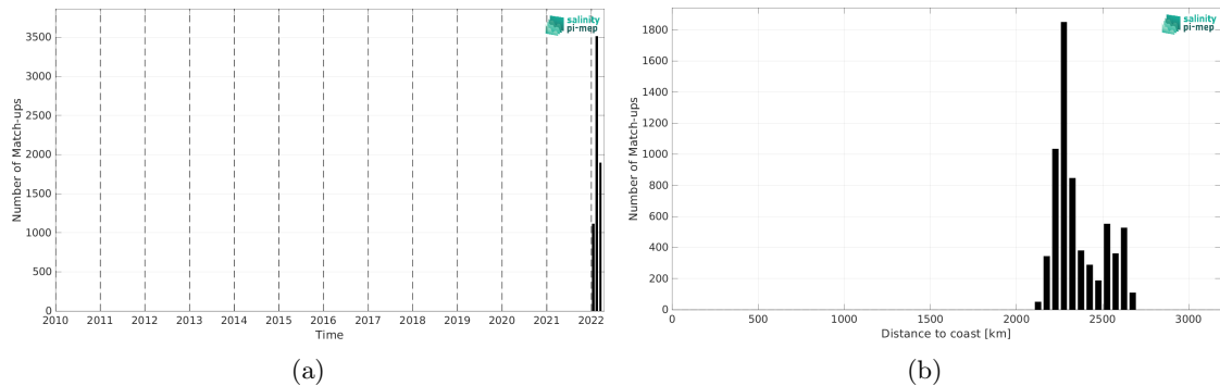
Figure 1: Number of match-ups between Saildrone and SMOS SSS L3 v9 - 18 Days (CATDS-CEC-LOCEAN) SSS as a function of time (a) and as function of the distance to coast (b) over the OTT zone Pi-MEP region and for the full satellite product period.
