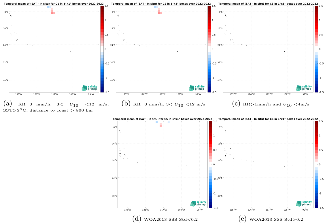
Figure 12: Temporal mean gridded over spatial boxes of size 1^\circ \times 1^\circ of \Delta SSS (SMOS SSS L3 v9 - 18 Days (CATDS-CEC-LOCEAN) - Sairdrone) for 5 different subdatasets corresponding to:RR=0 mm/h, 3 < U_{10} < 12 m/s, SST >5^\circ C, distance to coast > 800 km (a), RR=0 mm/h, 3 < U_{10} < 12 m/s (b), RR >1 mm/h and U_{10} < 4 m/s (c), WOA2013 SSS Std <0.2 (d), WOA2013 SSS Std >0.2 (e).
