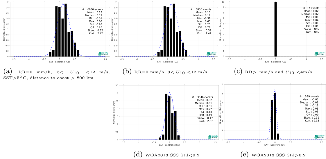
Figure 13: Normalized histogram of \Delta SSS (SMOS SSS L3 v9 - 18 Days (CATDS-CEC-LOCEAN) - Sairdronne) for 5 different subdatasets corresponding to: RR=0 mm/h, 3 < U_{10} < 12 m/s, SST > 5°C, distance to coast > 800 km (a), RR=0 mm/h, 3 < U_{10} < 12 m/s (b), RR > 1mm/h and U_{10} < 4 m/s (c), WOA2013 SSS Std < 0.2 (d), WOA2013 SSS Std > 0.2 (e).
